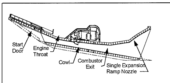
Figure 2: Scramjet Cross-Section
