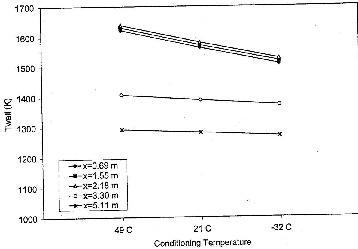
Figure 7. M256/M829A2 calibrated MACE wall temperature profile analysis for HC chromium maximum surface temperature.
