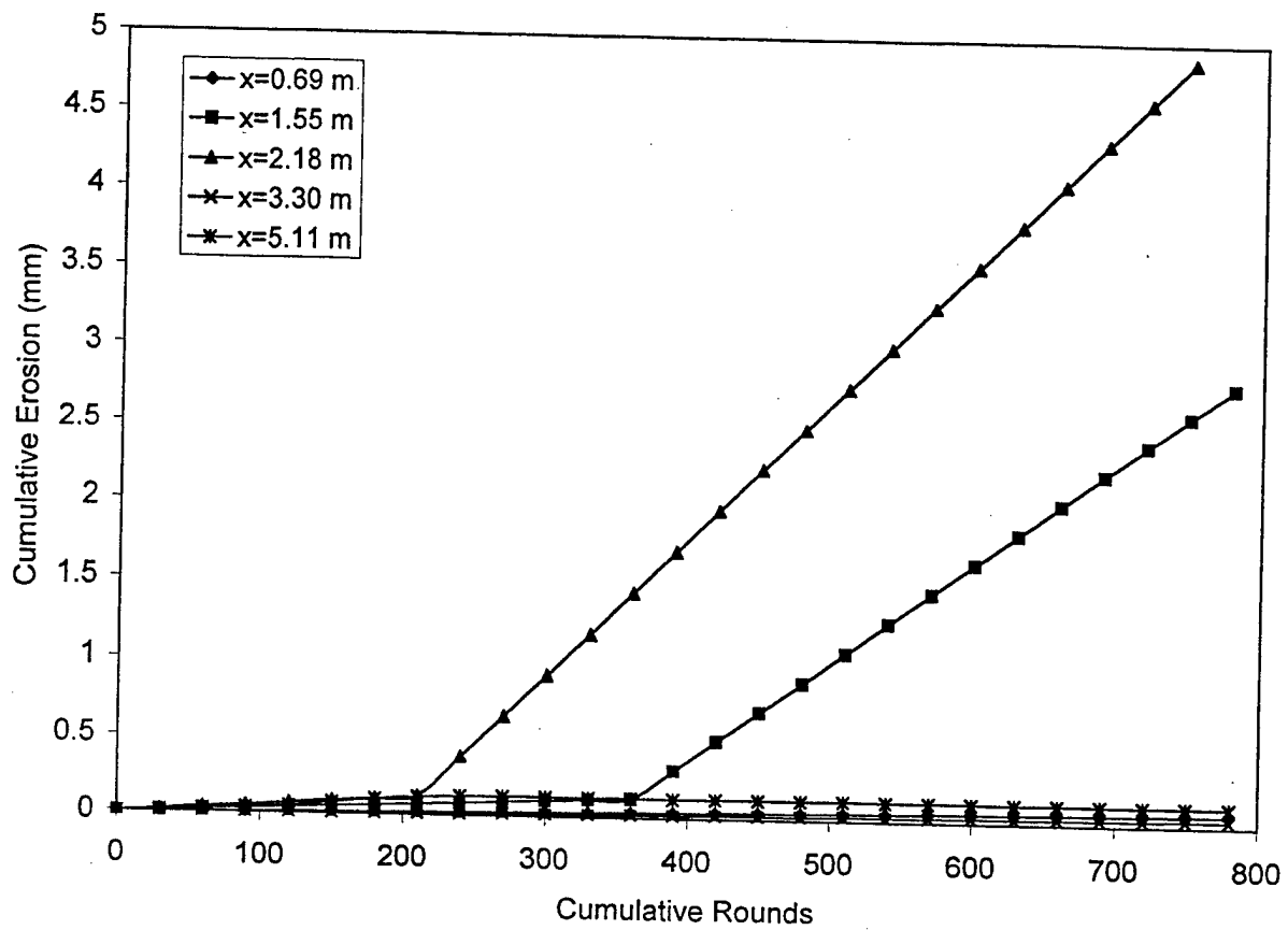
Figure 12. M256/M829A2 MACE cumulative erosion analysis for the unrealistic, but informative case of only -32°C conditioned rounds.
