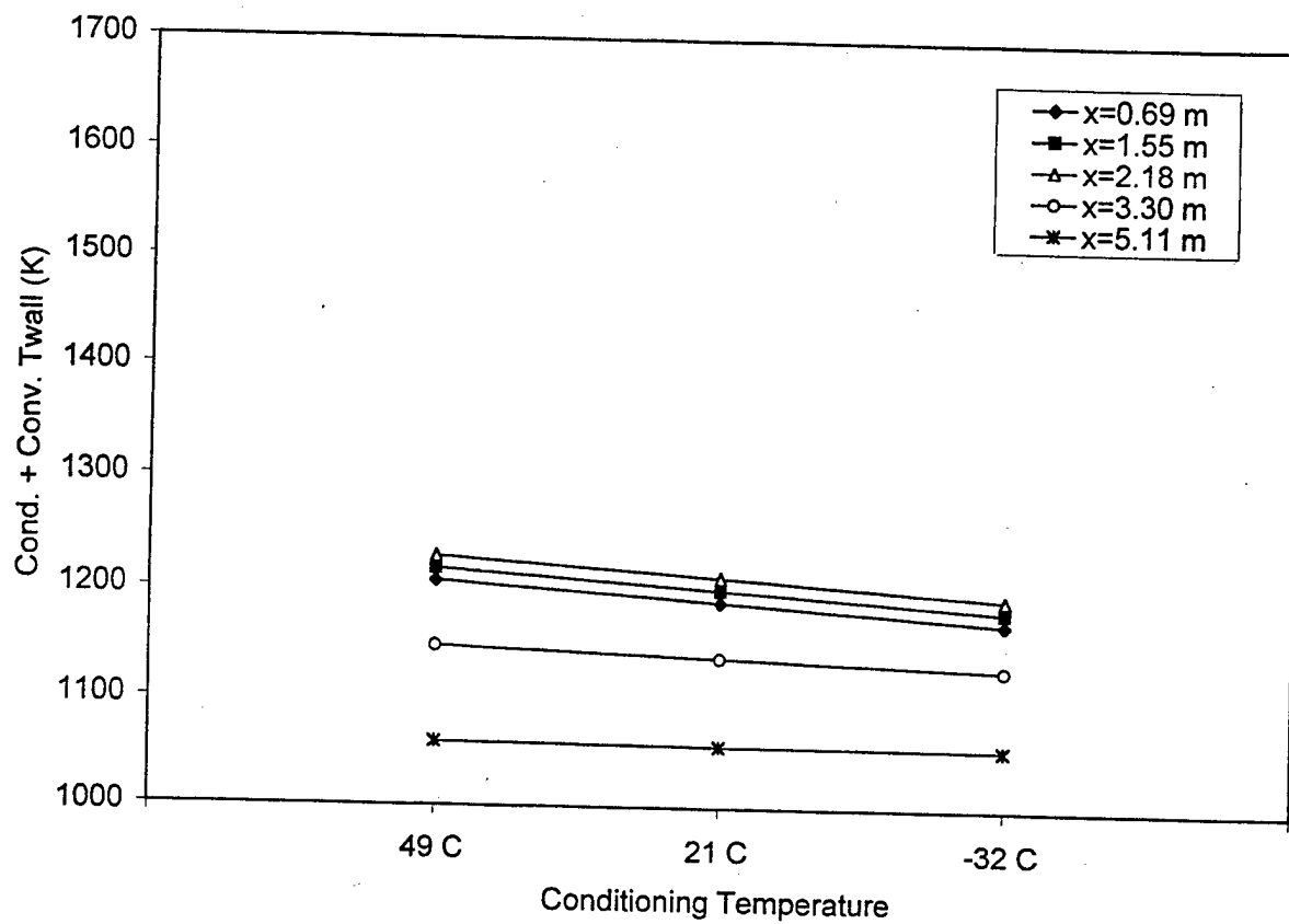
Figure 8. M256/M829A2 calibrated MACE wall temperature profile analysis for A723 maximum interface wall temperature.
