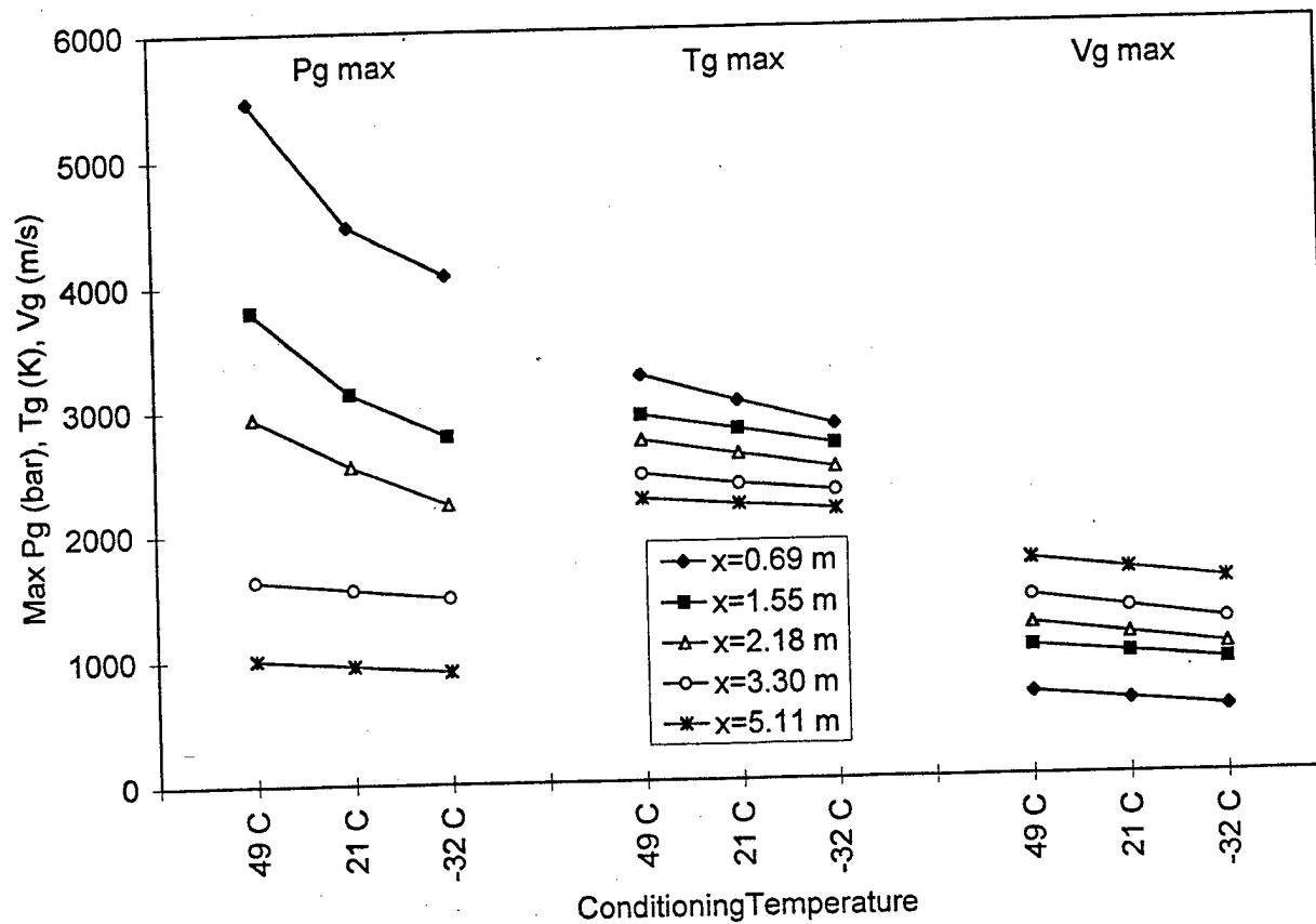
Figure 1. M829A2 calibrated XNOVAKTC interior ballistic analysis for maximum values of gas pressure, gas temperature, and gas velocity.
