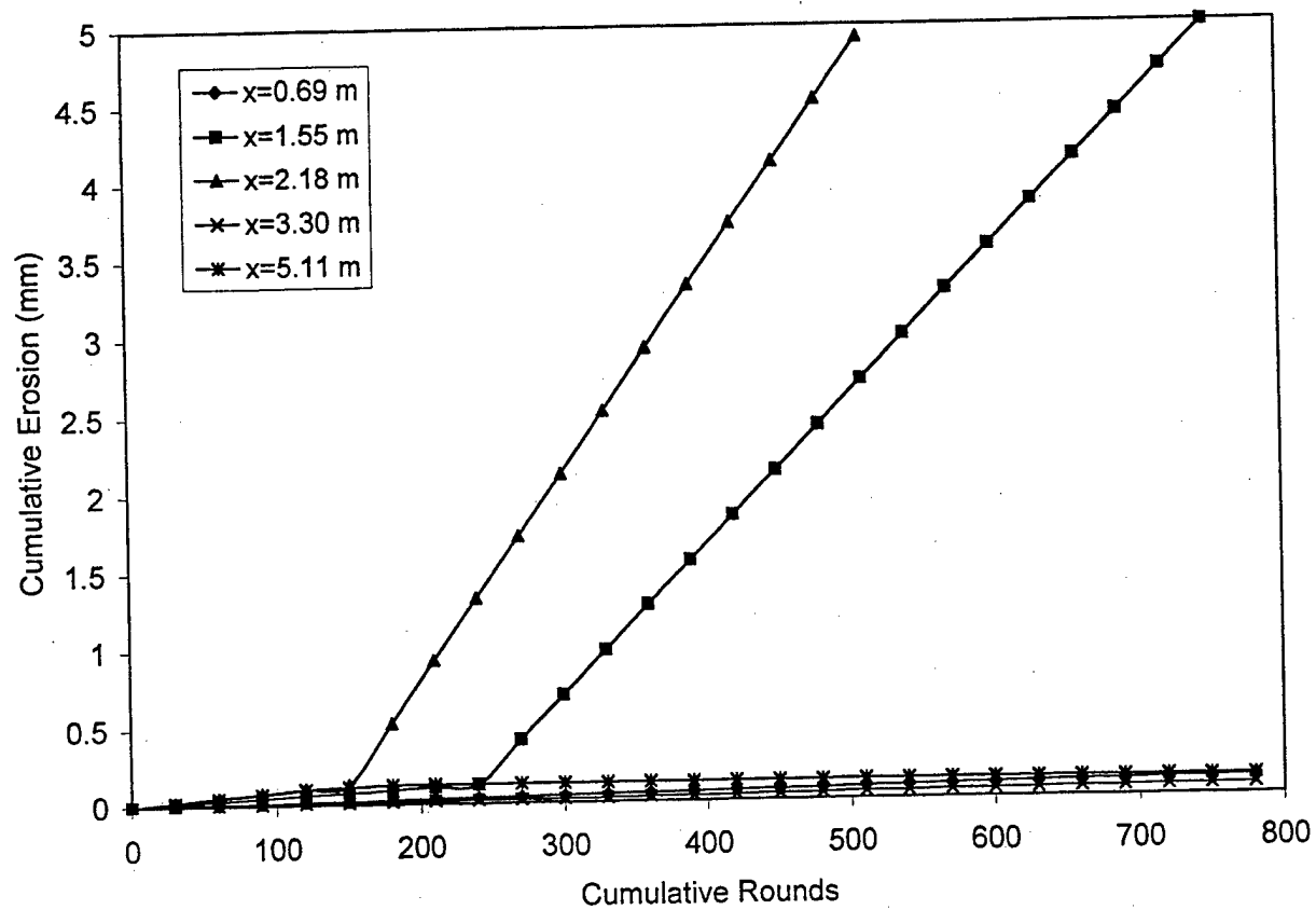
Figure 11. M256/M829A2 MACE cumulative erosion analysis for the unrealistic, but informative case of only 21°C conditioned rounds.
