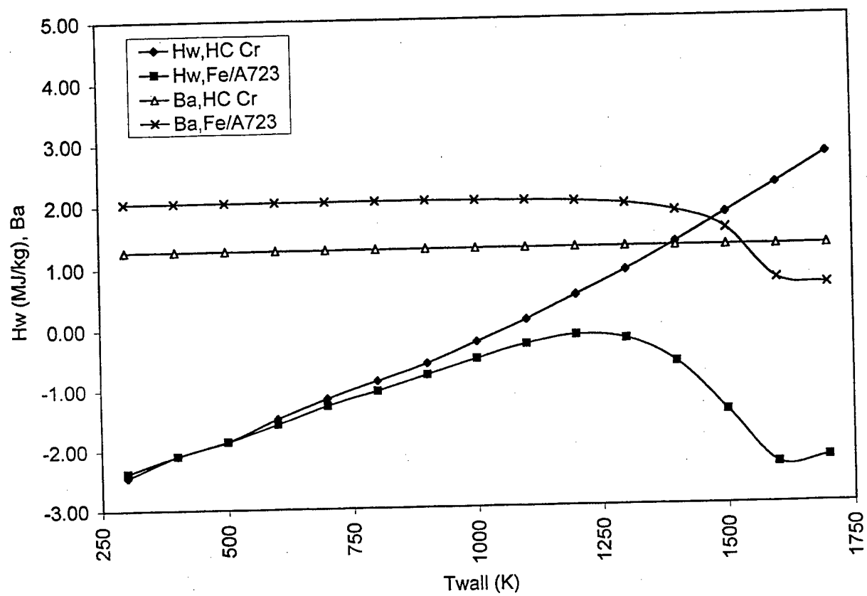
Figure 3. M829A2 calibrated CCET thermochemical analysis of reacting wall enthalpy and ablation potential.
