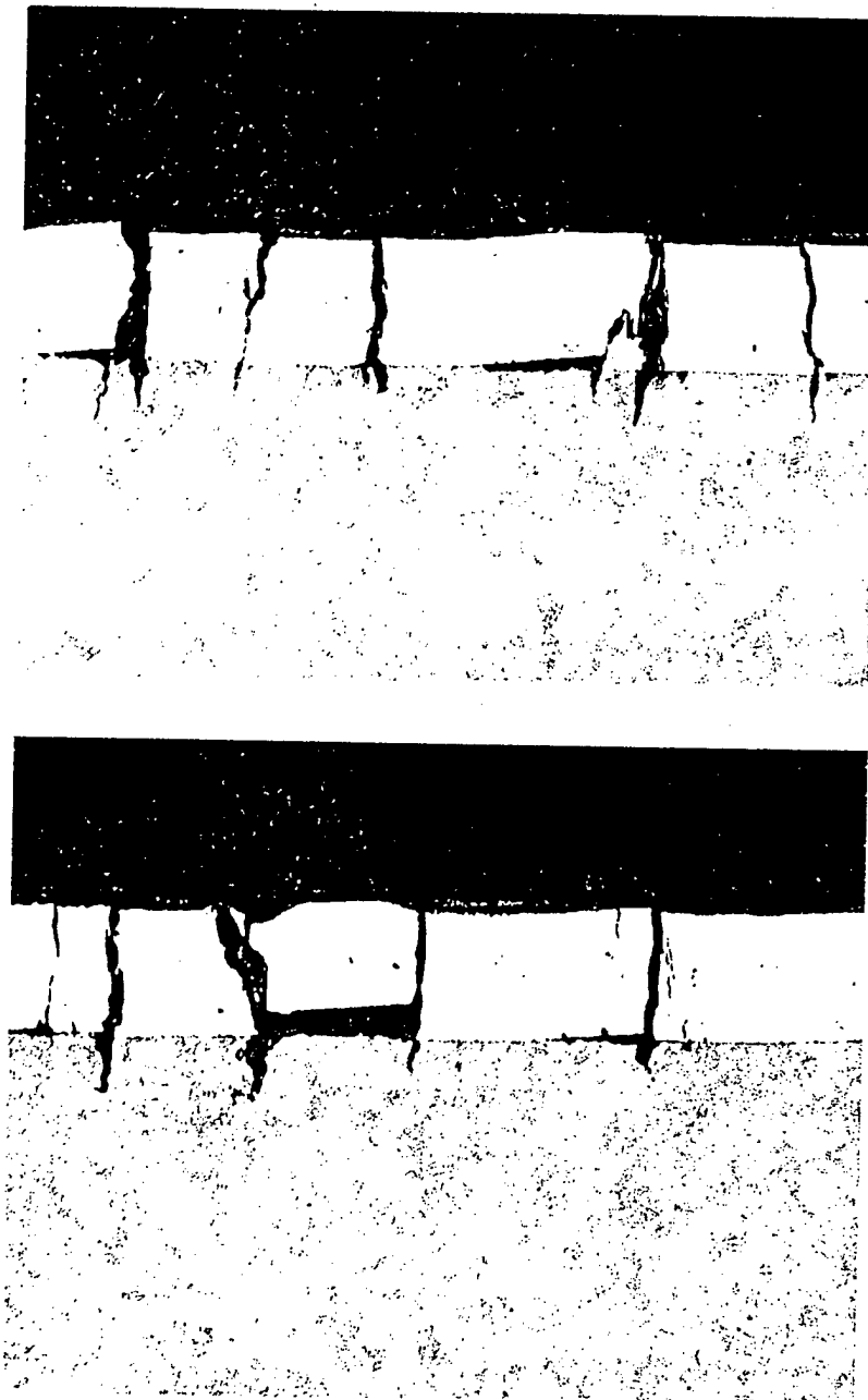
Figure 6. Tube #1988 metallographs at 1.55 meters representing 1.2 to 2.4 meter region (100x).
