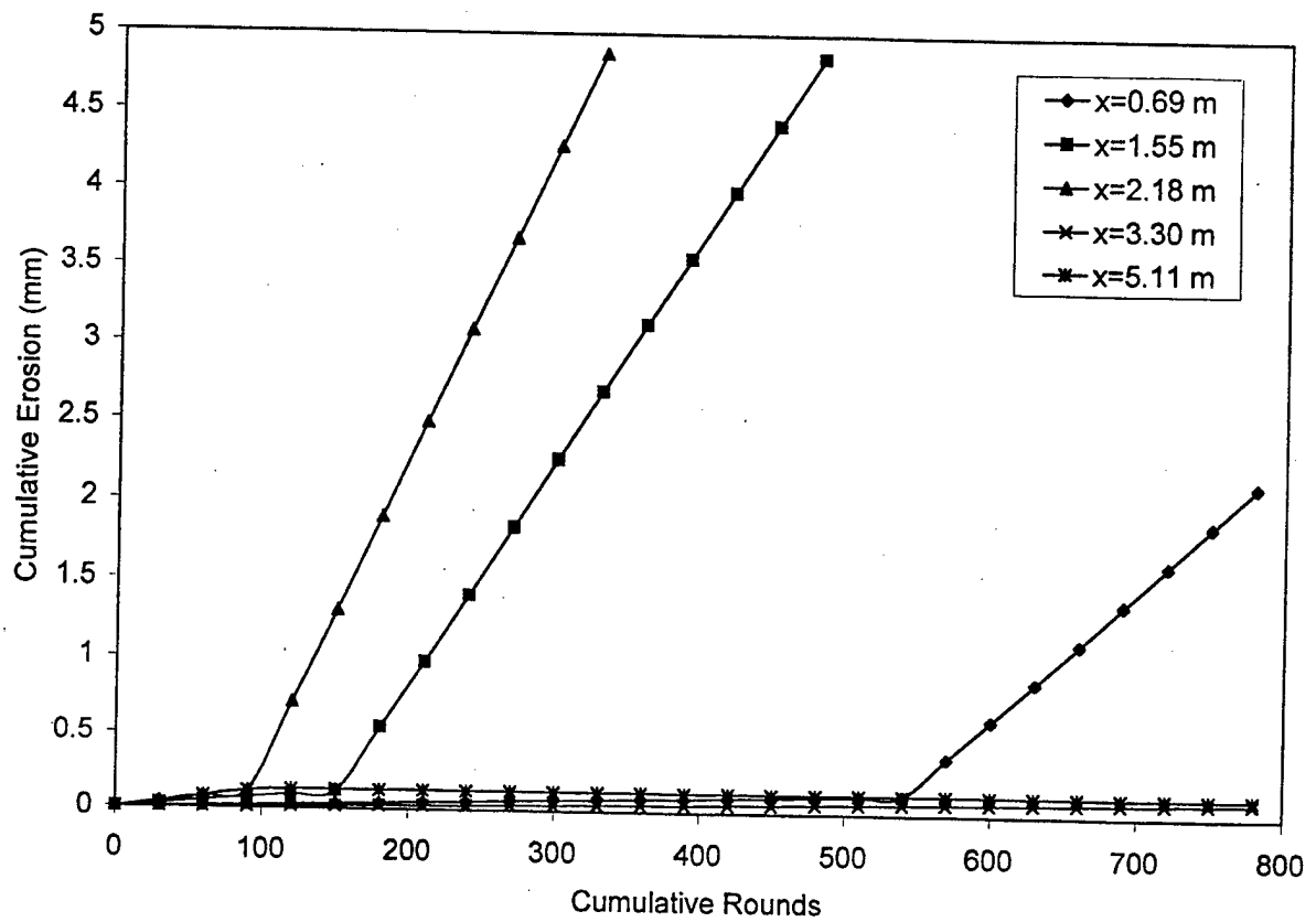
Figure 10. M256/M829A2 MACE cumulative erosion analysis for the unrealistic, but informative case of only 49°C conditioned rounds.
