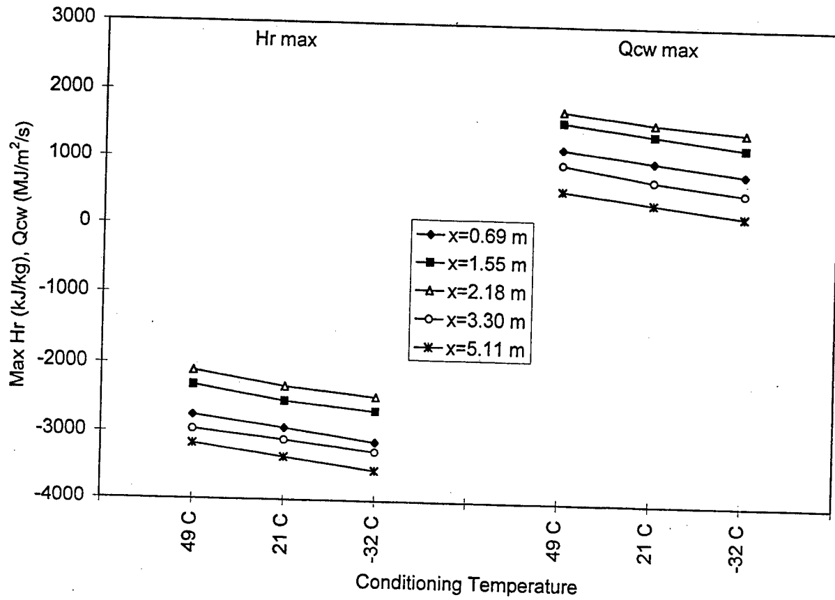
Figure 2. M829A2 calibrated MABL analysis for maximum values of recovery enthalpy and cold wall heat flux.
