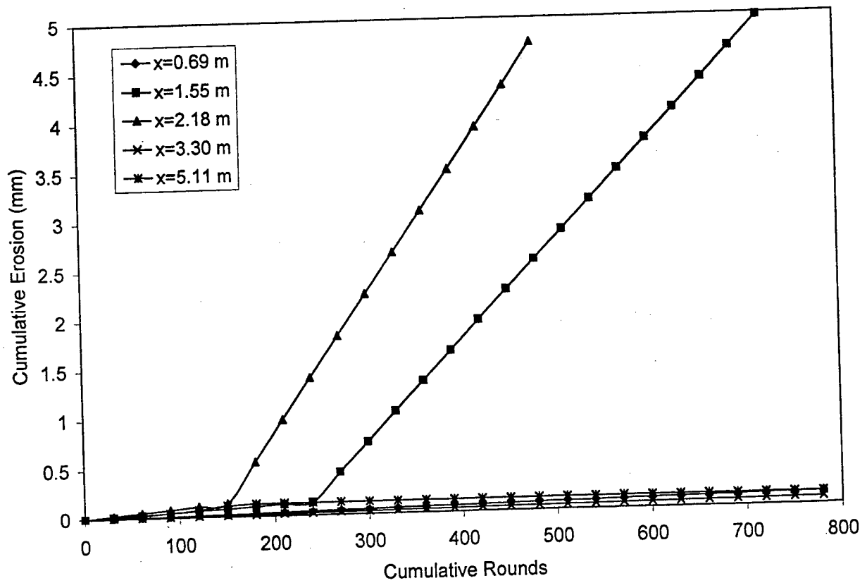
Figure 13. M256/M829A2 MACE cumulative erosion analysis for the semi-realistic and informative case of an equal distribution of hot/ambient/cold-conditioned rounds.
