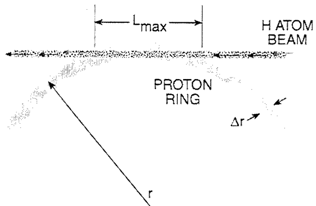
Figure 4. Geometry for neutral H atom injection into the CBFR. To be trapped, the H atoms must be ionized while traversing the chord of length \leq L_{\max} .
