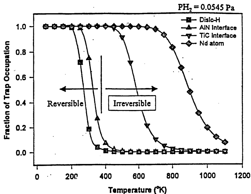
Figure 1. Fraction of filling by hydrogen at trap sites as a function of temperature for various hydrogen-trap binding energies.
