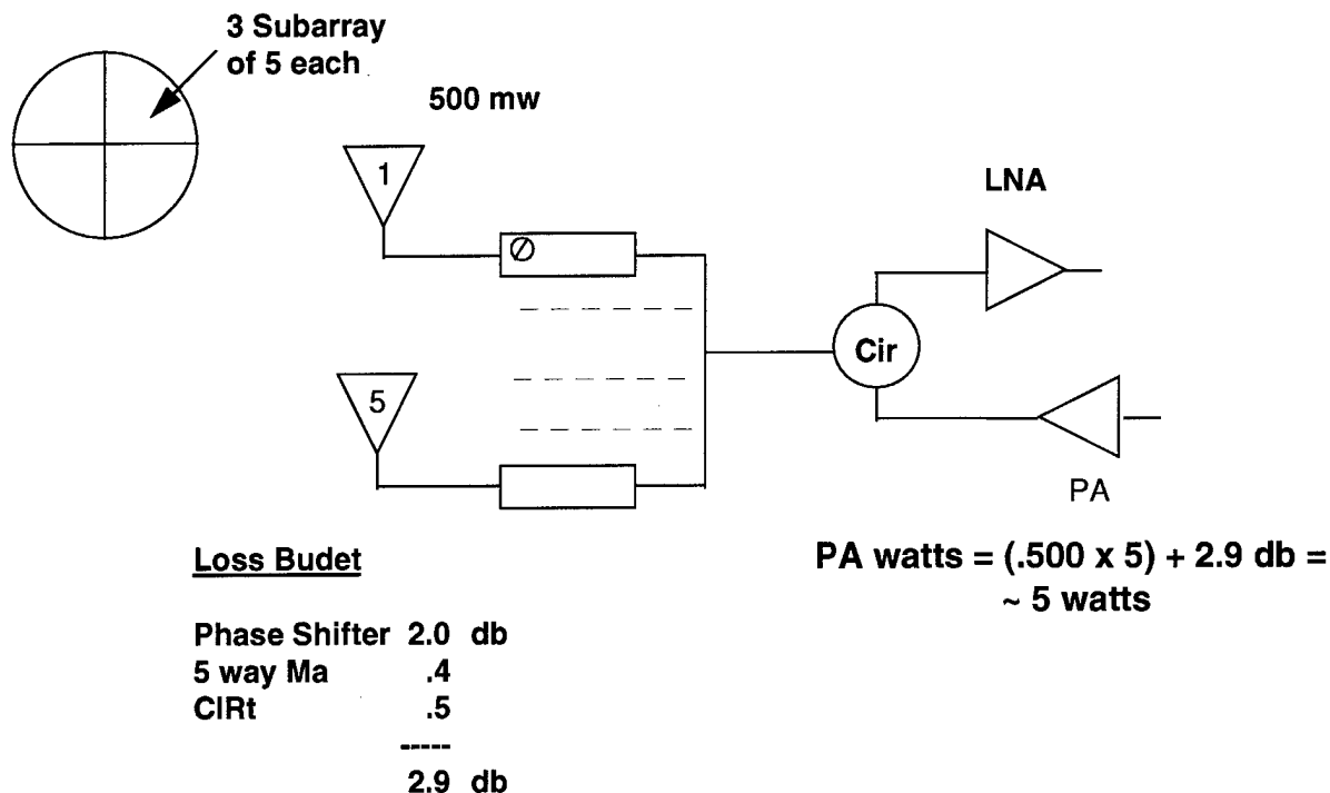
Figure 14. X-Band ESA Functional Block Diagram
