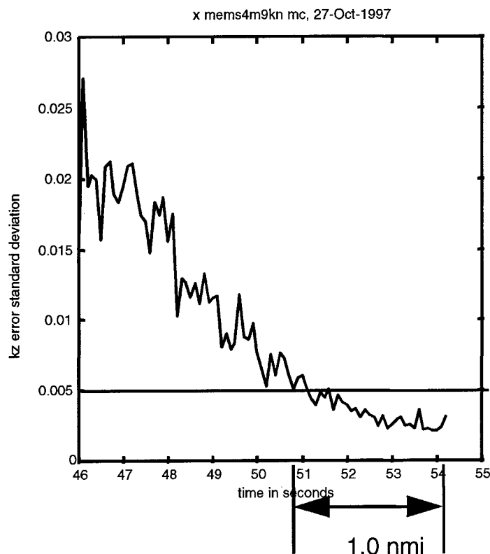
Figure 10. X-Band Elevation Angle Error vs. Mission Time
