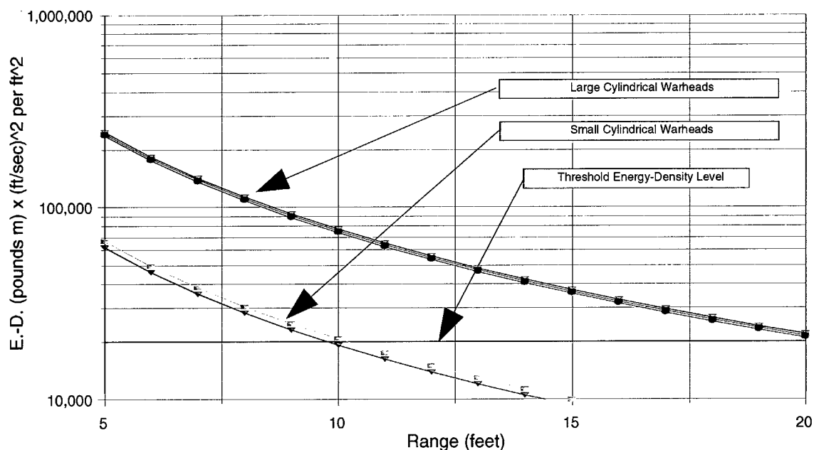
Figure 23. Energy Density vs Range for Cylindrical Warheads
