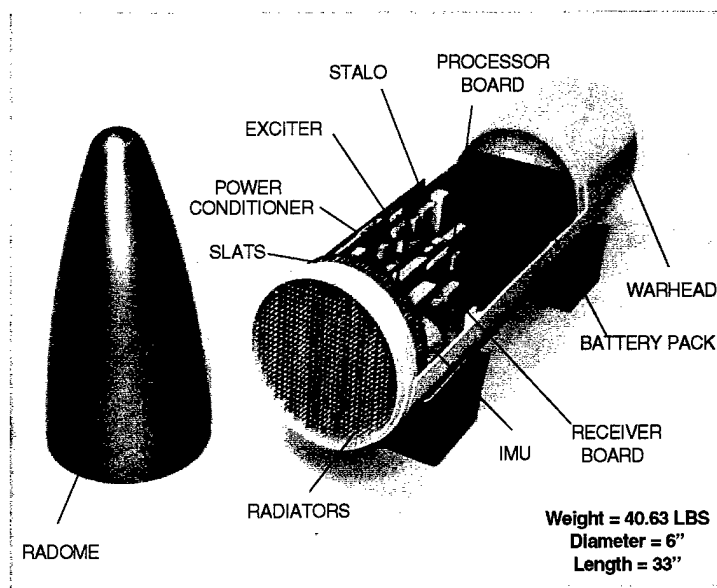
Figure 6. Ka-Band Seeker Mockup
