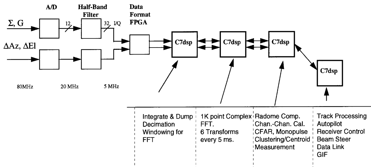
Figure 17. X-Band Digital Processor Functional Block Diagram
