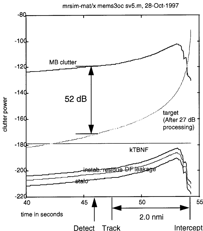
Figure 9. X-Band Seeker Performance
