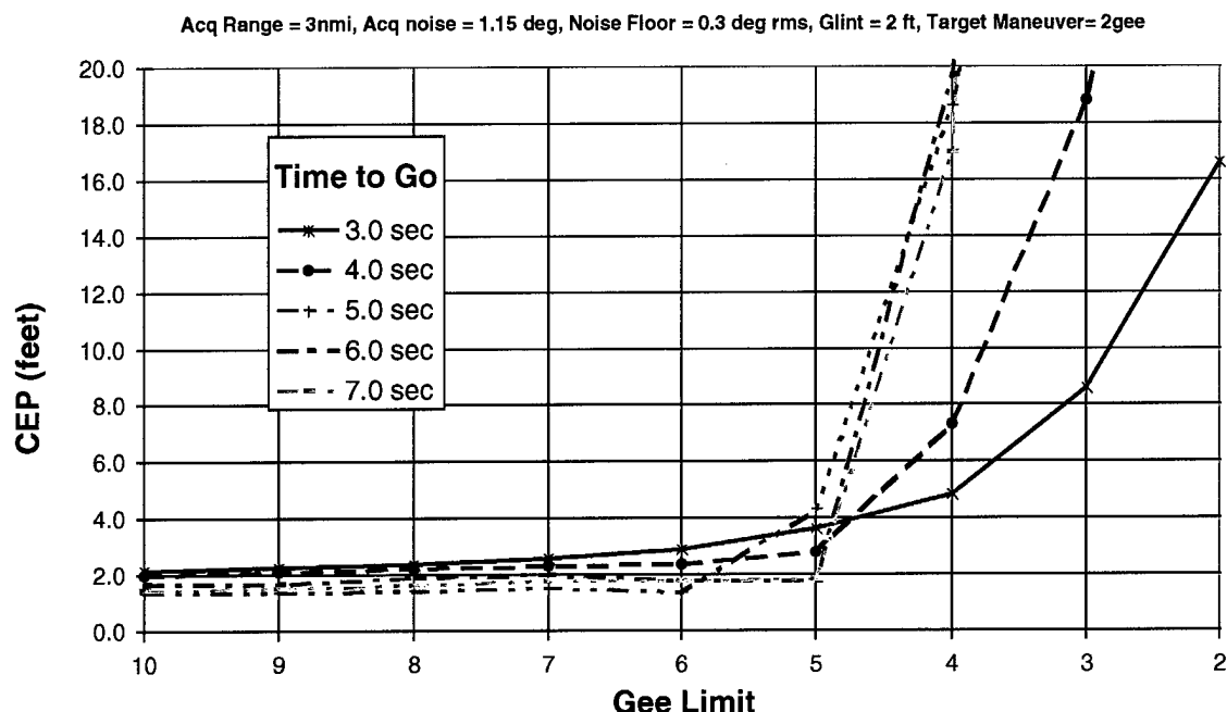
Figure 21. Airframe Gee Requirement Parametric Study
