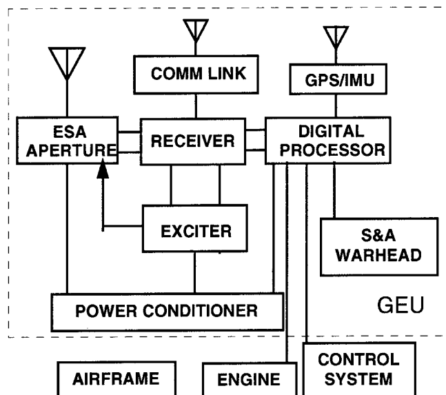
Figure 4. Interceptor Development Block Diagram
