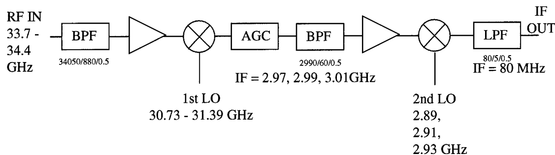
Figure 19. Ka-Band Receiver Functional Block Diagram
