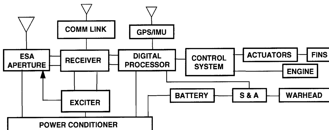
Figure 13. MLI System Block Diagram
