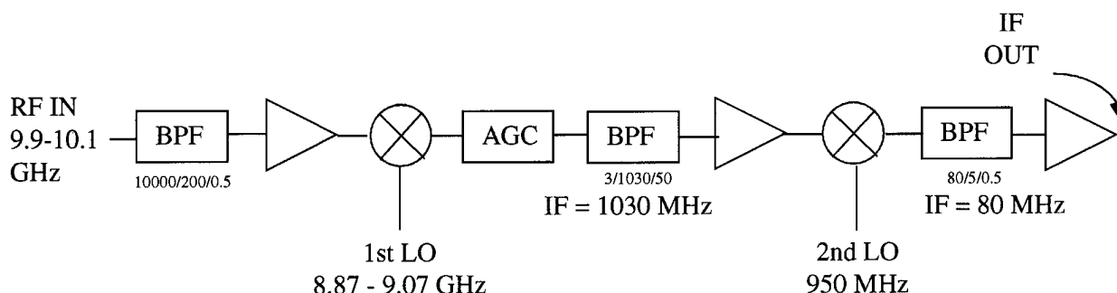
Figure 15. X-Band Receiver Functional Block Diagram
