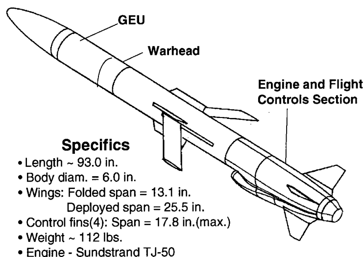
Figure 3. LCCMD Interceptor Concept
