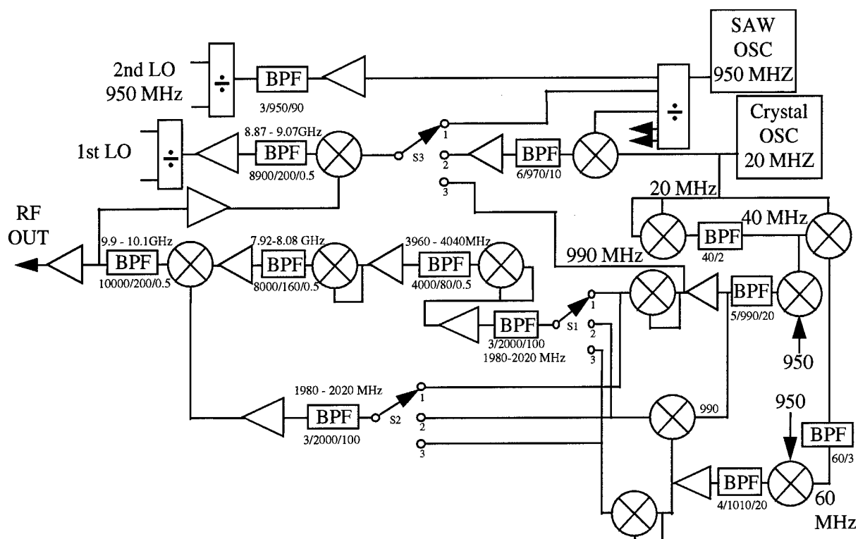
Figure 16. X-Band Exciter Functional Block Diagram
