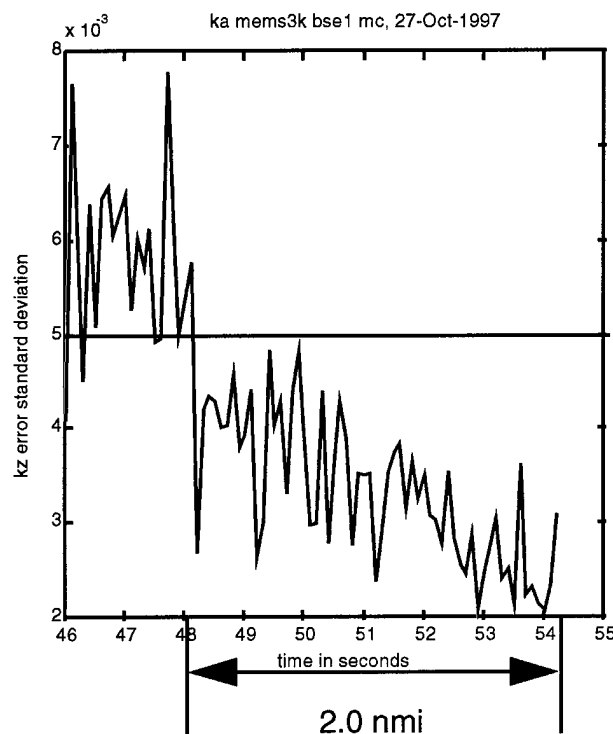
Figure 12. Ka-Band Elevation Angle Noise vs. Mission Time
