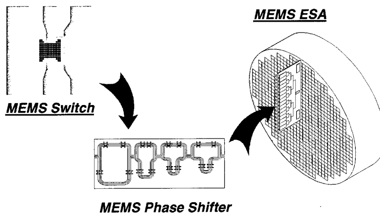
Figure 5. Electronically Scanned Antenna (ESA)
