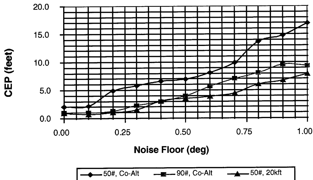
Figure 22. 6DOF CEP Predictions versus Range Independent Angle Noise with Engine Thrust and Engagement Geometry as a Parameter
