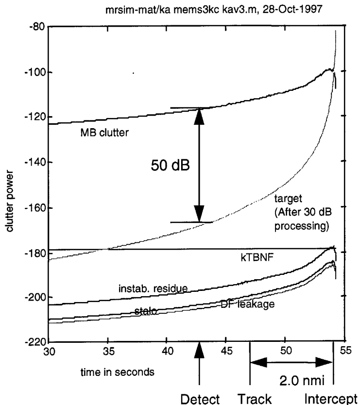
Figure 11. Ka-Band Seeker Performance vs. Mission Time
