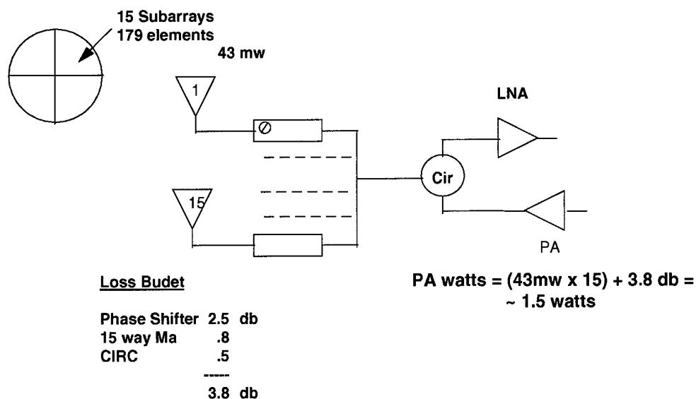
Figure 18. Ka-Band ESA Functional Block Diagram
