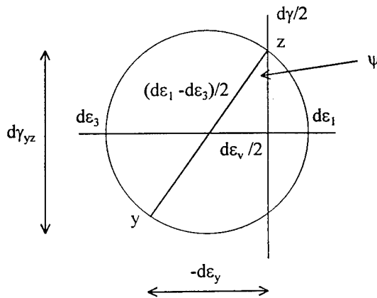
Figure 1.11 Angle of Dilation ( \Psi ) -Mohr Circle
