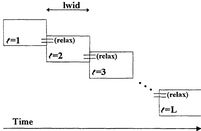
Figure 3: A Lagrangian cascade partitions the rows and columns of a monolith into many Lagrangian subproblems \ell of contiguous time periods. Overlapping rows are Lagrange-relaxed.
