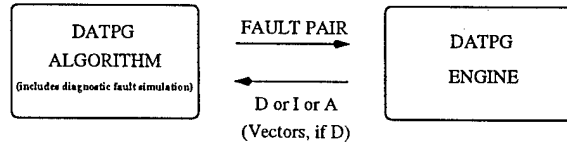
Figure 3: DATPG and the diagnostic engine
