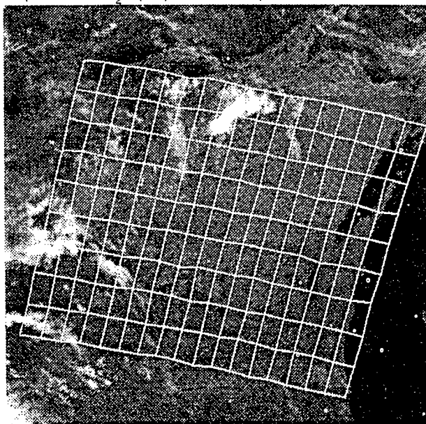
Figure 3. AVHRR 10.7 \mu\text{m} Image for the Analysis Area of Figure 1, With the HIRS Grid Overlay
