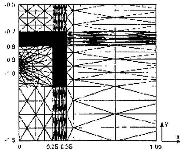
Figure 2. Finite-element mesh showing mesh refinement necessary for insulation and pipe.
