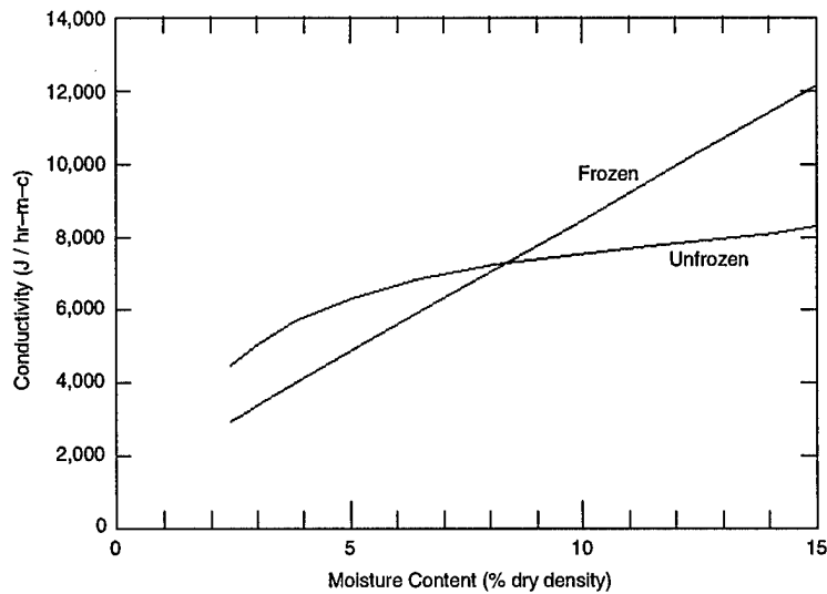
Figure 12. Frozen and unfrozen thermal conductivity, plotted against moisture content, of 1800 kg/m 3 sandy soil. (From Kersten 1949.)
