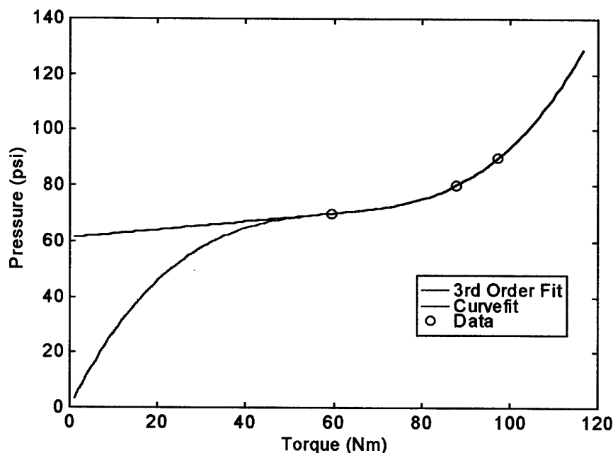
Figure 16: Pressure Versus Torque at 1070 RPM.
