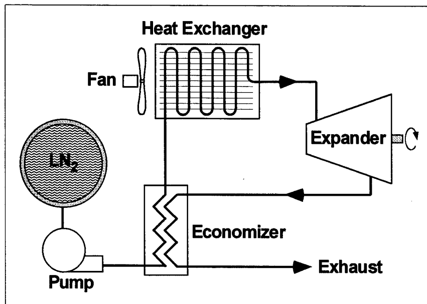
Figure 3: Liquid Nitrogen Propulsion System.
