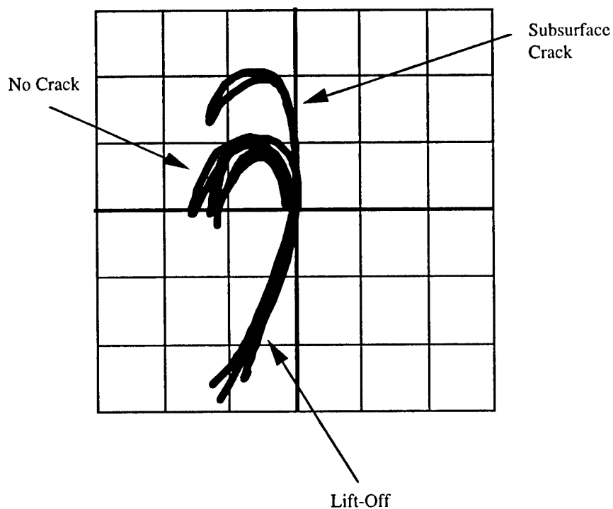
FIGURE 49. EDDY-CURRENT INSTRUMENT DISPLAY FOR SUBSURFACE CRACK
