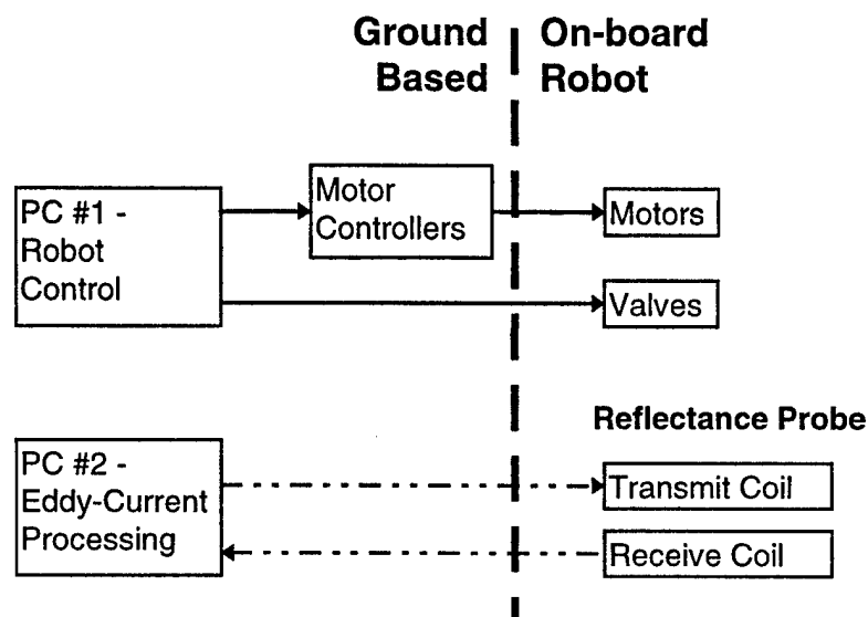
FIGURE 1. FIRST-PHASE SYSTEM ARCHITECTURE
