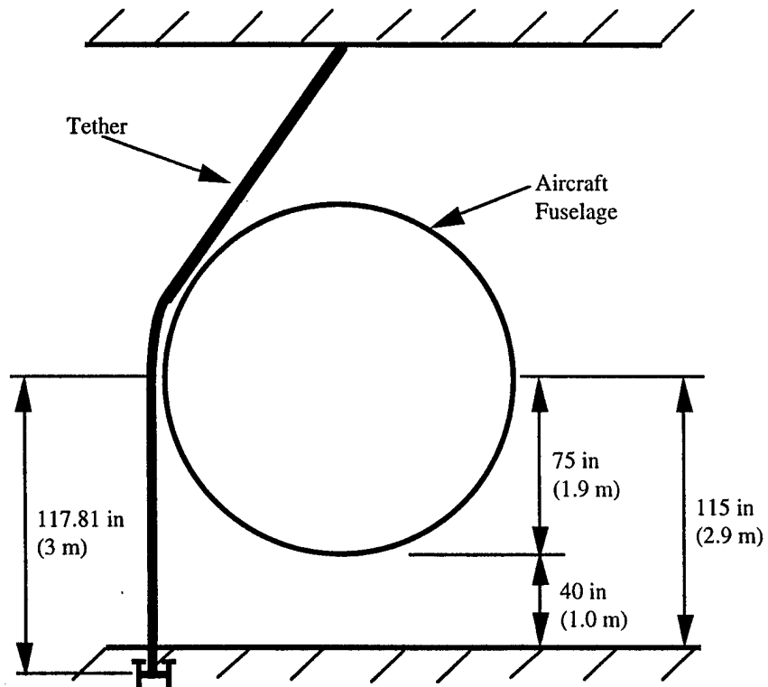
FIGURE 20. TETHER LIMITATION
