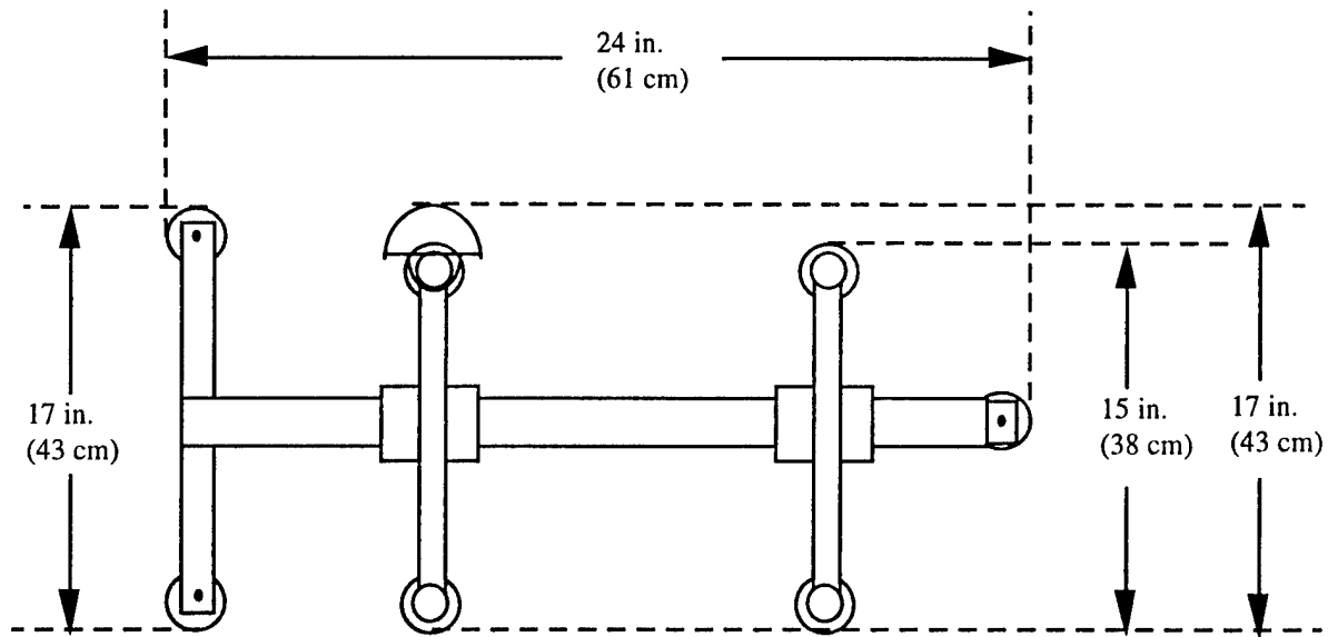
FIGURE 7. ROBOT DIMENSIONS (OVERHEAD VIEW)
