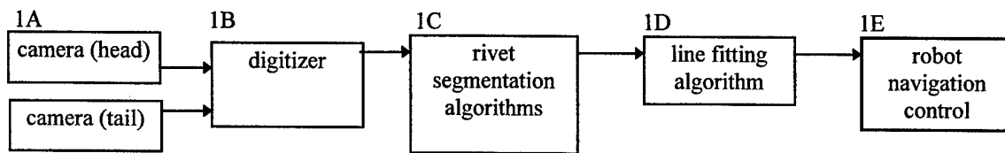
FIGURE 59. RIVET SEGMENTATION AND LINE-FITTING IN ROBOT NAVIGATION
