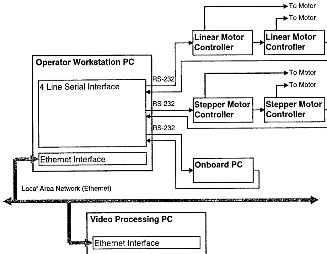
FIGURE 39. COMMUNICATIONS SUBSYSTEM
