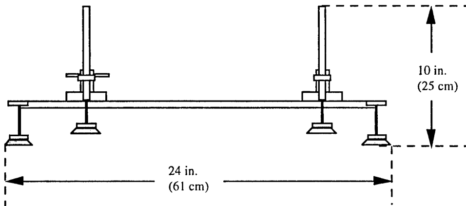
FIGURE 8. ROBOT DIMENSIONS (SIDE VIEW)
