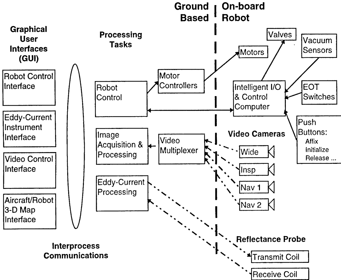
FIGURE 3. SECOND-PHASE SYSTEM ARCHITECTURE
