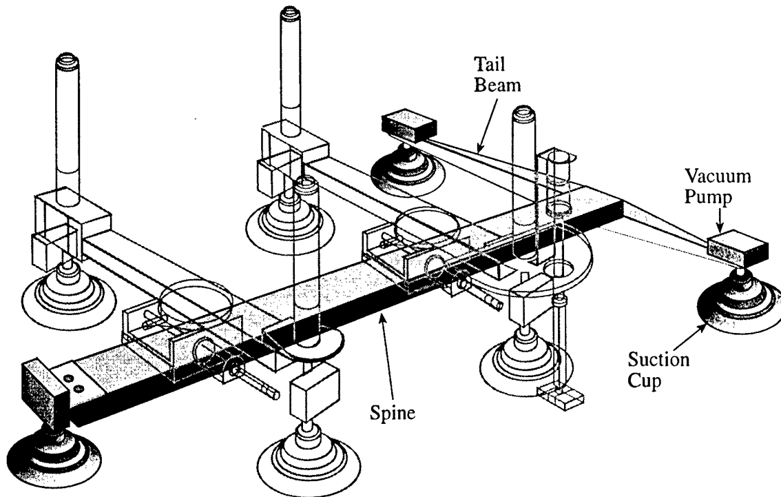
FIGURE 15. DRAWING OF THE SPINE ASSEMBLY
