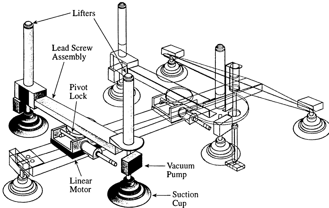
FIGURE 10. DRAWING OF THE STABILIZER BRIDGE
