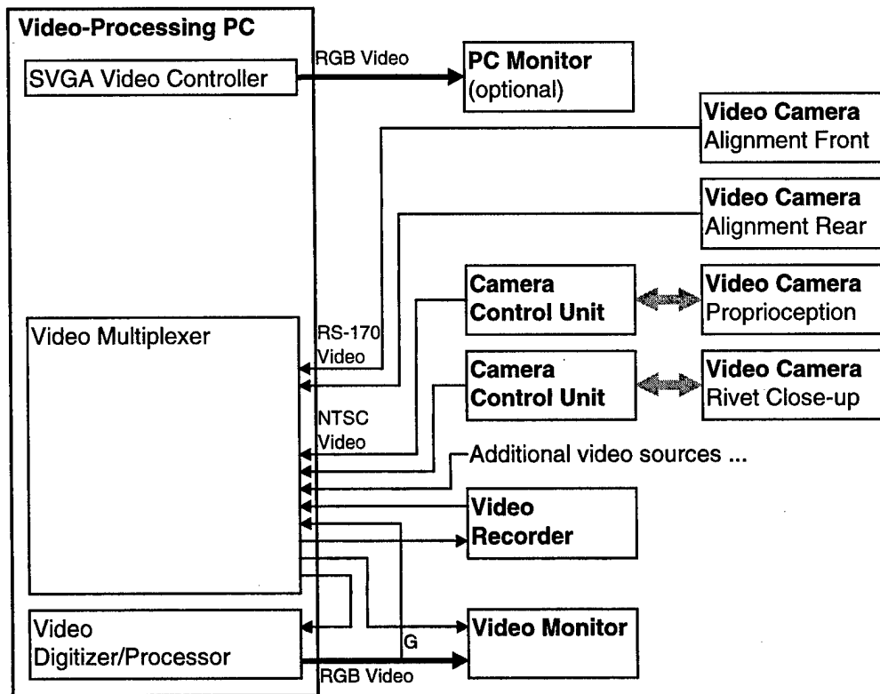
FIGURE 56. VIDEO SUBSYSTEM
