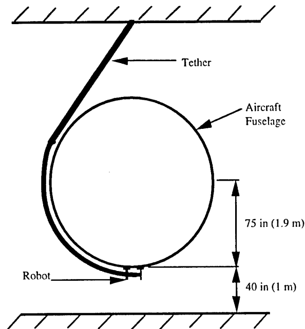
FIGURE 19. ROBOT TETHERED TO BOTTOM OF AIRCRAFT
