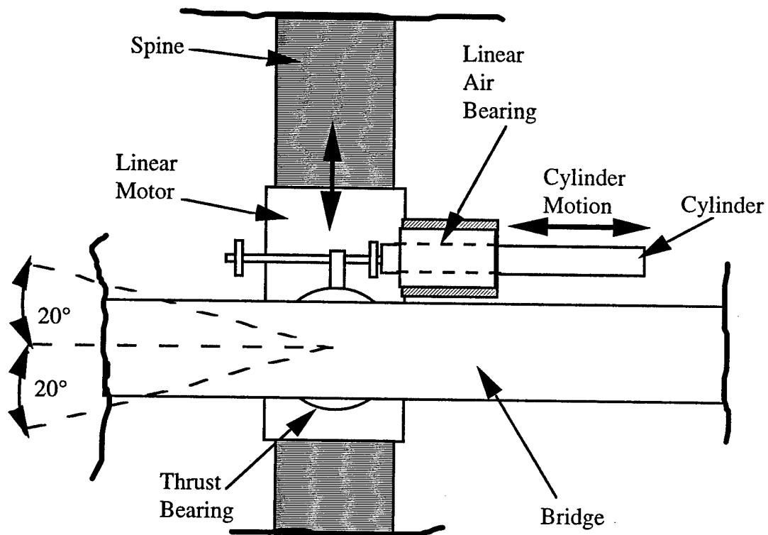
FIGURE 12. PIVOT LOCK SCHEMATIC (UNLOCKED)
