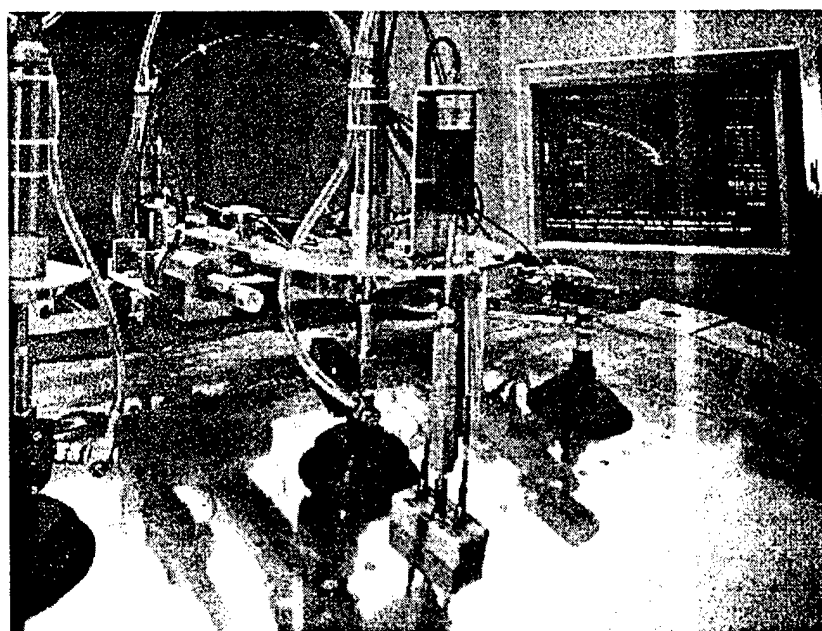
FIGURE 46. EDDY-CURRENT SENSOR DEPLOYED BY FIRST-PHASE ROBOT
