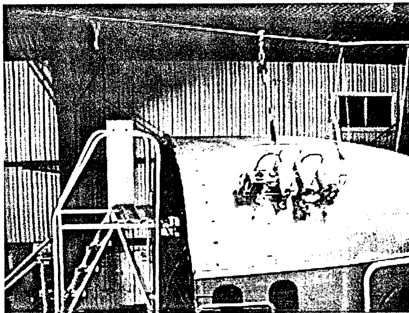
FIGURE 5. SECOND-PHASE ROBOT ON DC-9 NOSE SECTION
