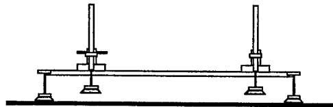
FIGURE 28. UNALIGNED ROBOT (SIDE VIEW)
