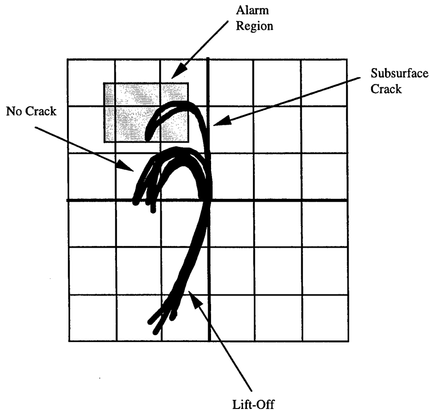
FIGURE 55. ALARM REGION ON AN IMPEDANCE-PLANE DISPLAY
