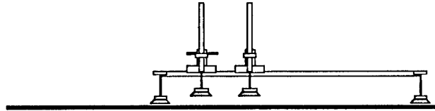
FIGURE 25. WALKING MOTION: SPINE ASSEMBLY LOWERED
