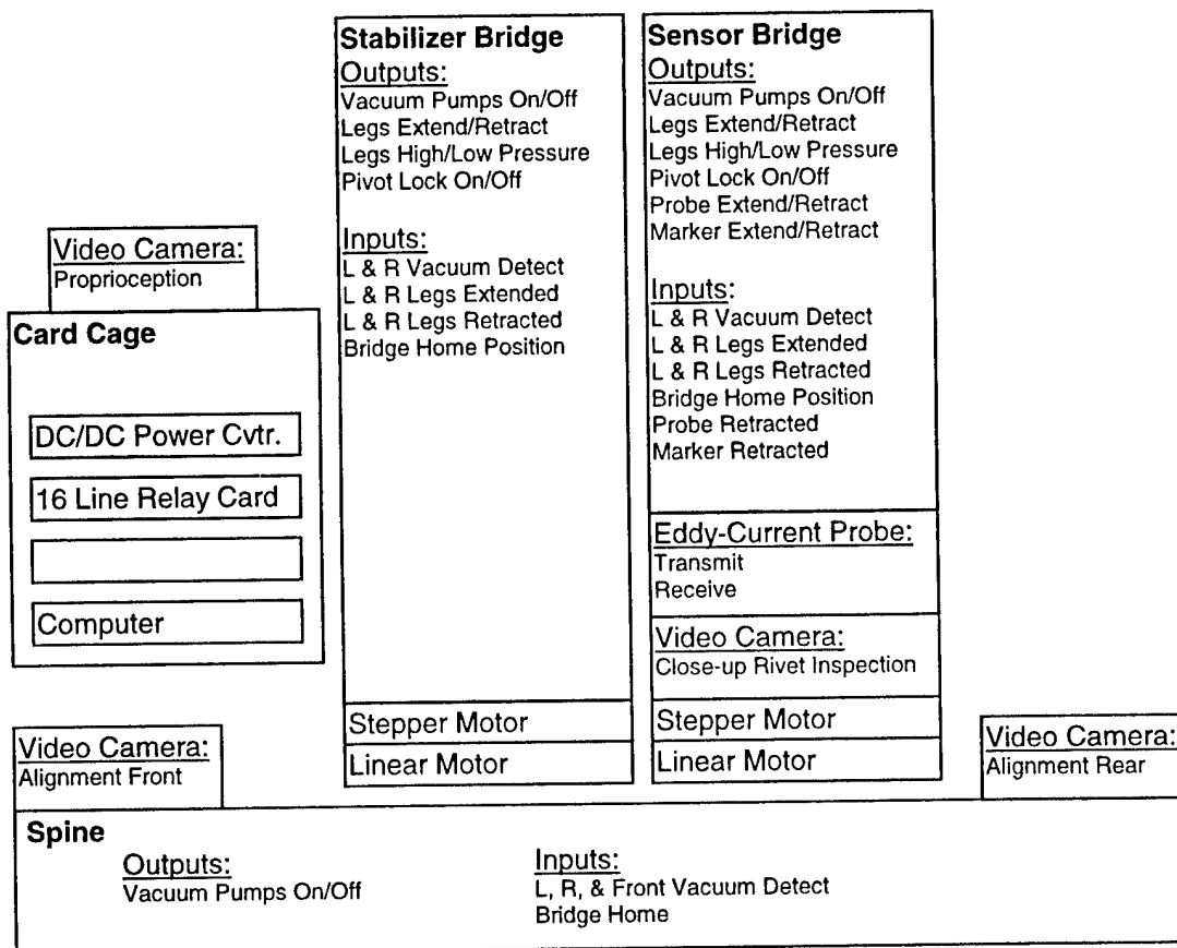
FIGURE 35. ON-BOARD COMPUTER AND ROBOT ELECTRONICS
