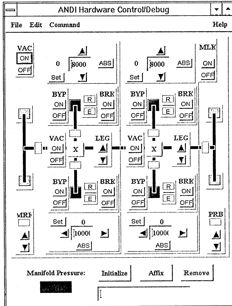
FIGURE 40. ROBOT CONTROL INTERFACE
