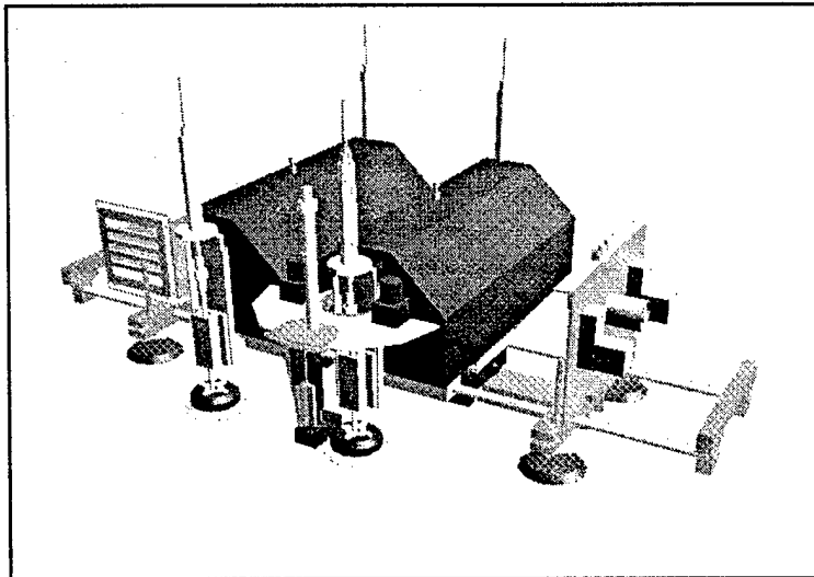
FIGURE 44. THREE-DIMENSIONAL RENDERING OF THE ROBOT
