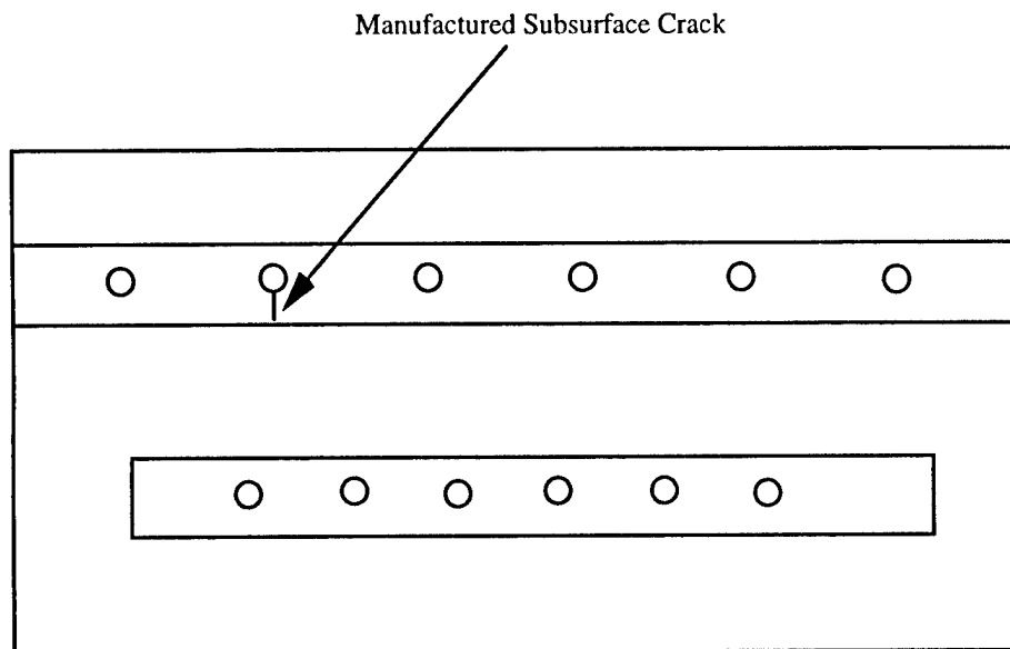
FIGURE 48. CALIBRATION STANDARD (BACK)
