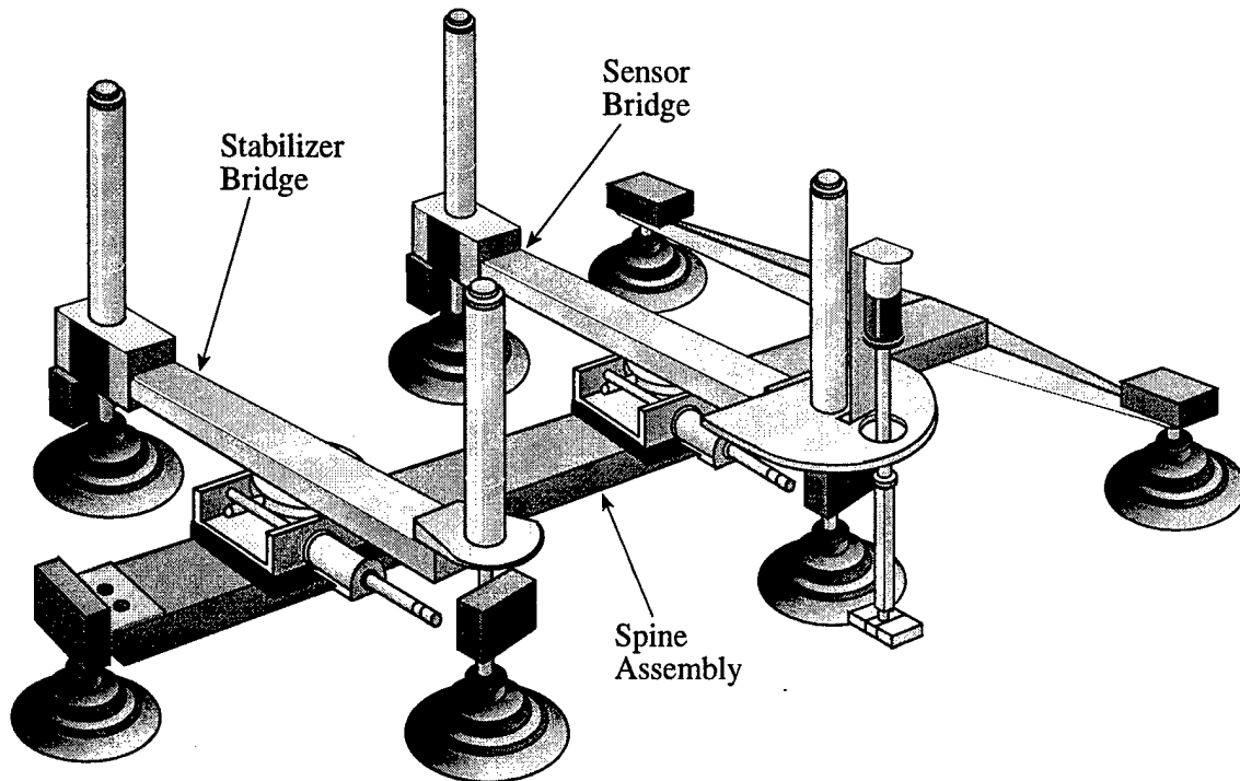
FIGURE 6. DRAWING OF THE CRUCIFORM ROBOT
