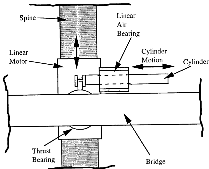
FIGURE 13. PIVOT LOCK SCHEMATIC (LOCKED)
