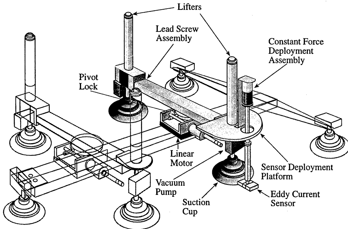
FIGURE 14. DRAWING OF THE SENSOR BRIDGE
