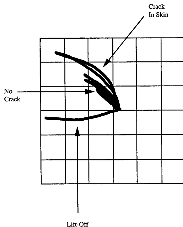
FIGURE 50. EDDY-CURRENT INSTRUMENT DISPLAY FOR SURFACE CRACK
