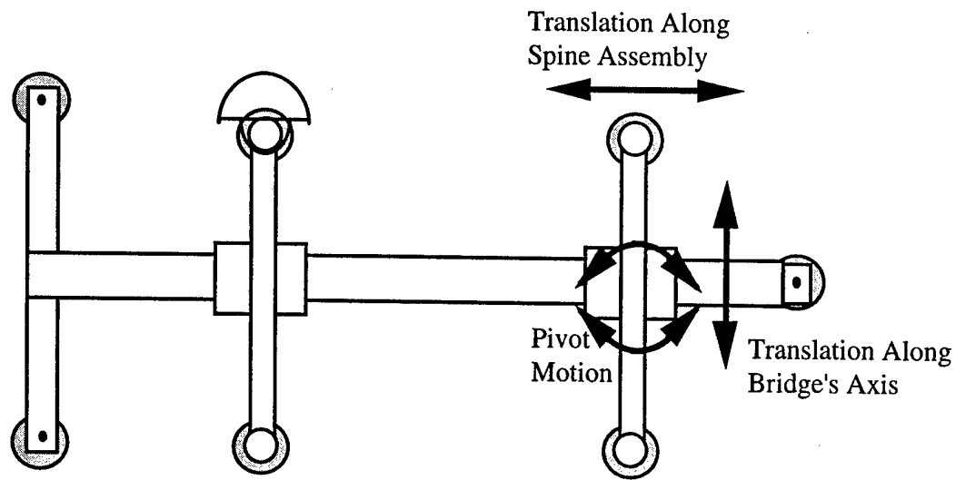
FIGURE 11. STABILIZER BRIDGE MOTIONS
