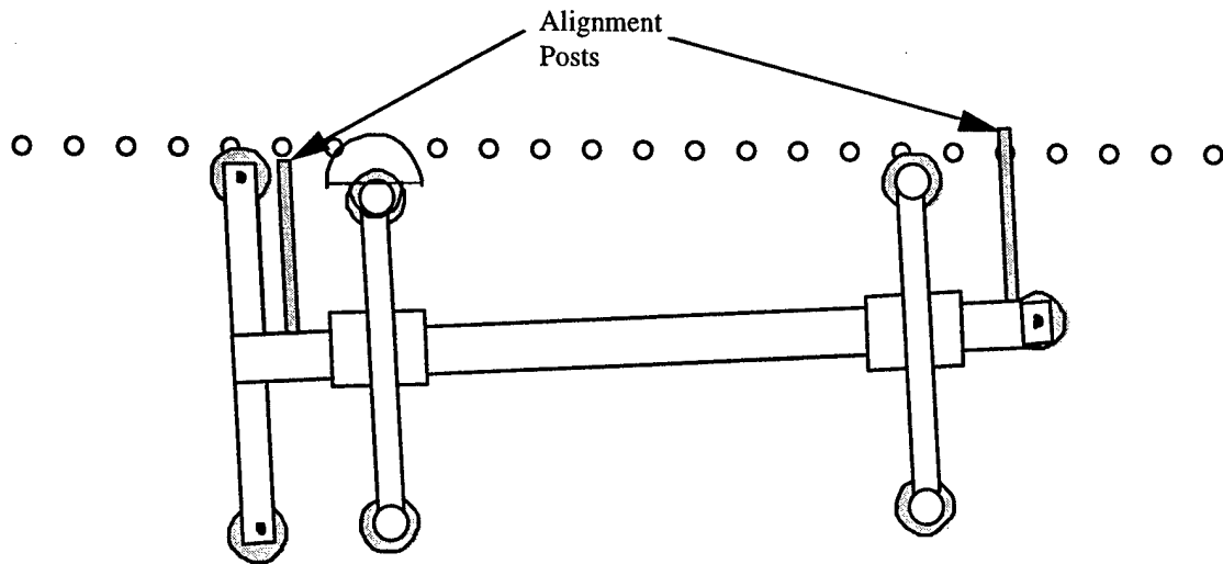
FIGURE 27. UNALIGNED ROBOT (OVERHEAD VIEW)
