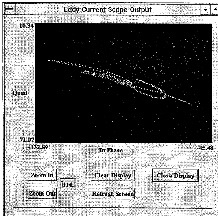
FIGURE 53. EDDY-CURRENT IMPEDANCE PLANE DISPLAY
