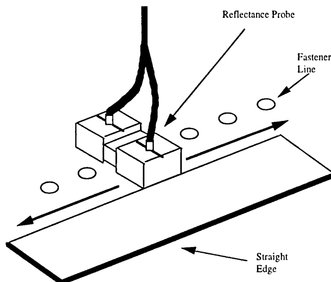
FIGURE 45. REFLECTANCE EDDY-CURRENT SENSOR
