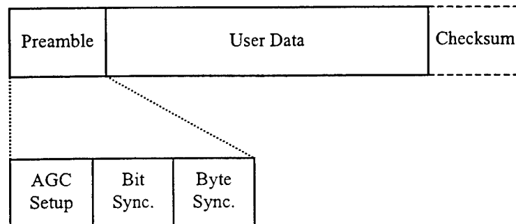
Figure II.6: Structure of a Typical Packet-Radio Frame [45]
