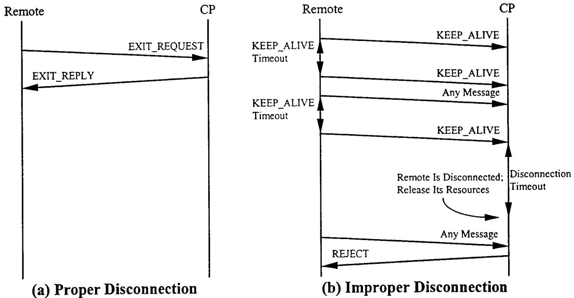
Figure III.6: Disconnection Procedure Diagrams
