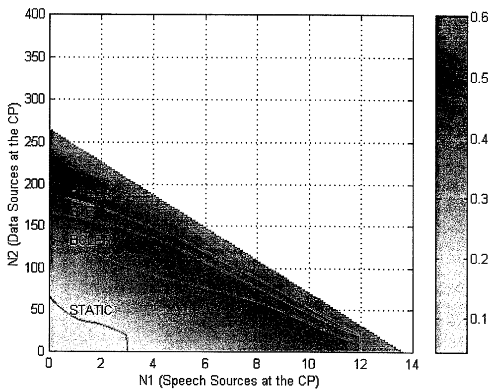
Figure VII.3: Admissible Region and Normalized Throughput for Partial Remote Status, Scenario 2
