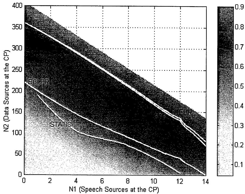
Figure VII.8: Admissible Region and Normalized Throughput for Complete Remote Status, Scenario 2
