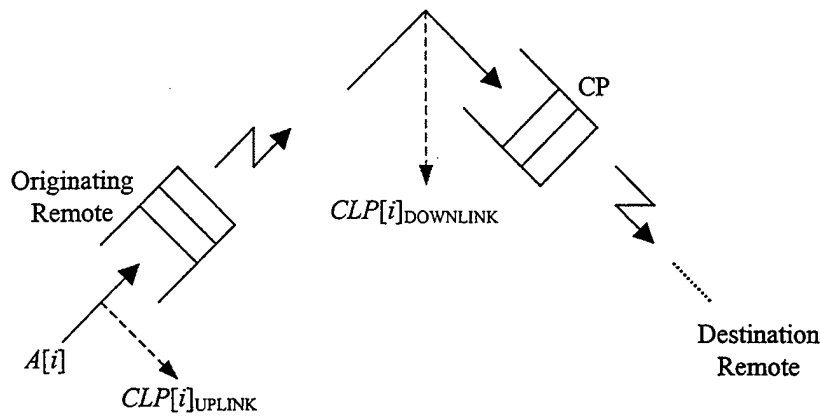
Figure VI.12: Flow of Cells and Possible Losses in a Remote-to-Remote Connection
