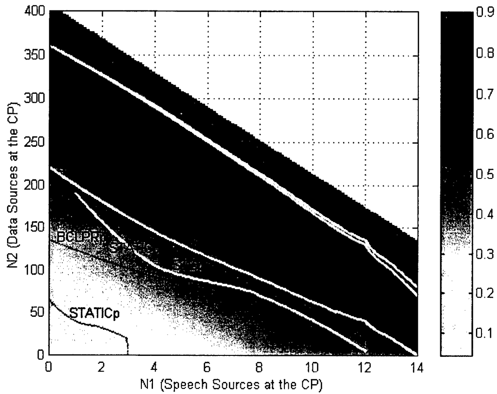
Figure VII.13: Admissible Region and Normalized Throughput for Partial- and Complete-Status Cases, Scenario 2
