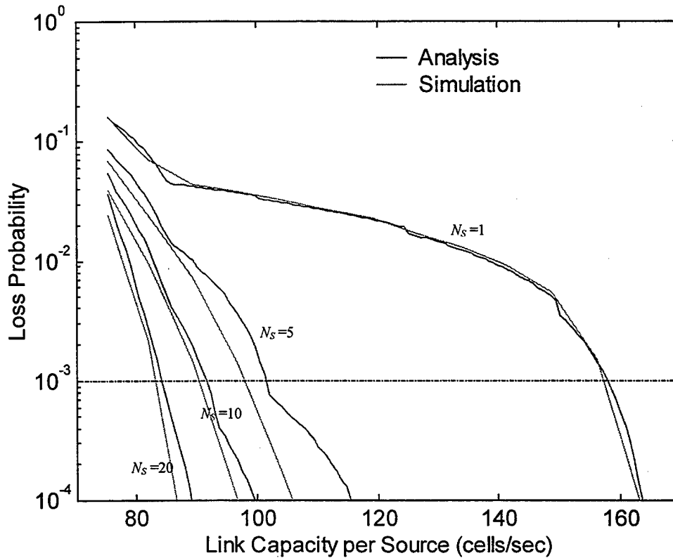
Figure V.4: Loss Probability for N_S Multiplexed Speech Sources
