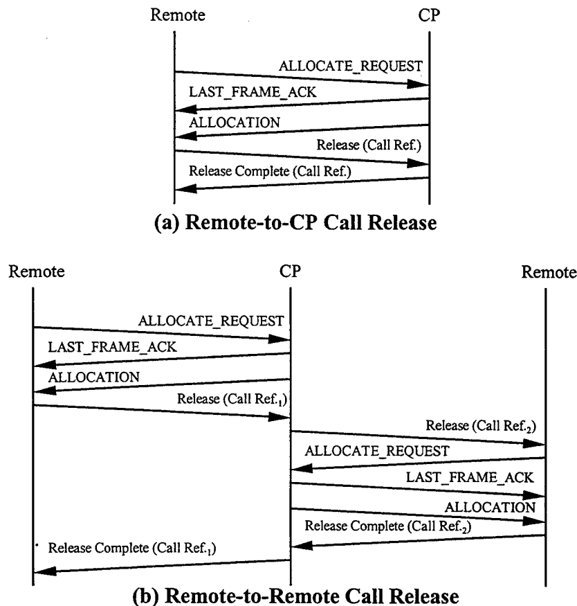
Figure III.8: Call-Release Procedure Diagrams
