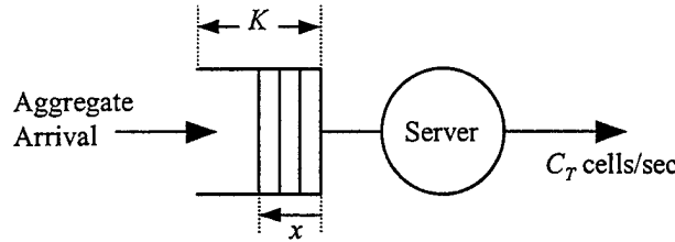
Figure V.2: Model of a Homogeneous Queueing System
