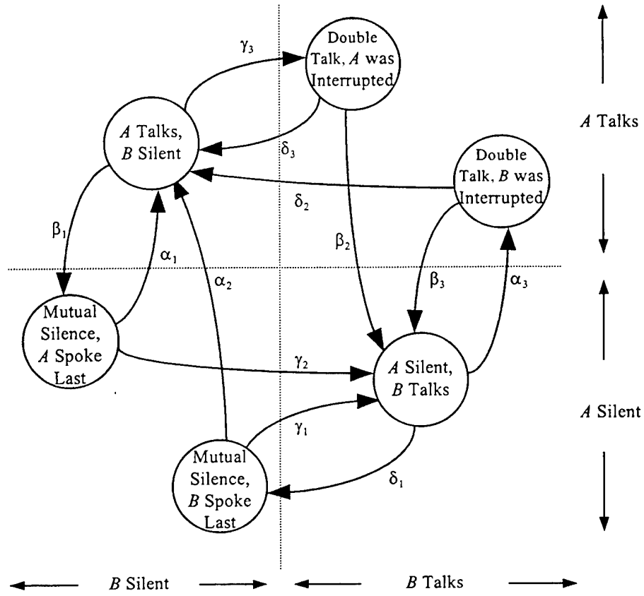
Figure IV.4: Markovian Model of a Two-Way Conversation [16]
