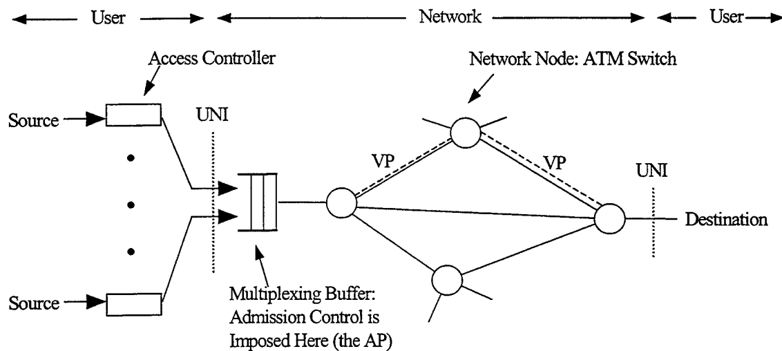
Figure II.2: General Structure of an ATM Network [80]
