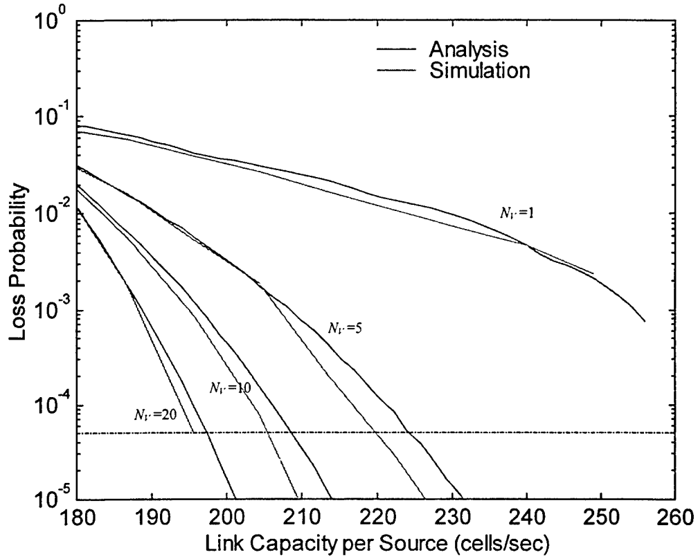
Figure V.5: Loss Probability for N_V Multiplexed Video Sources
