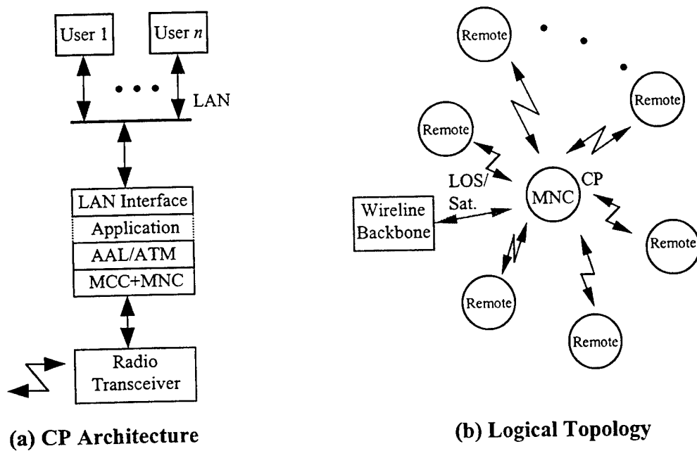
Figure II.12: CP Architecture with Combined MCC and MNC
