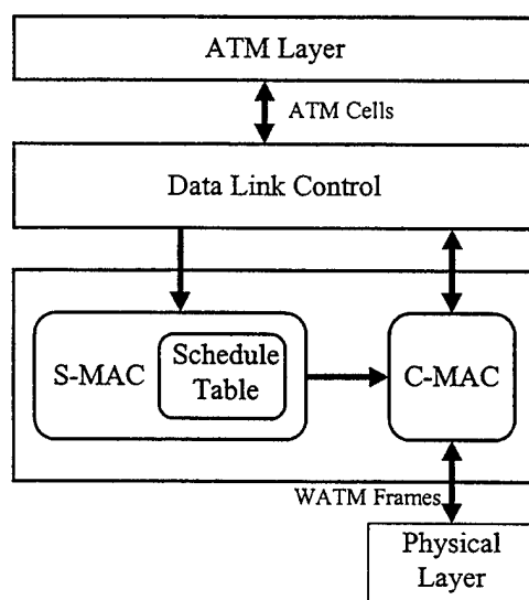
Figure II.8: Wireless ATM System Architecture [100]
