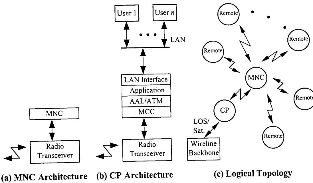
Figure II.11: CP Architecture with Separate MCC and MNC
