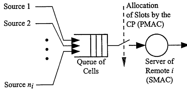
Figure VI.2: Multiplexing n_i Sources at Remote Station i
