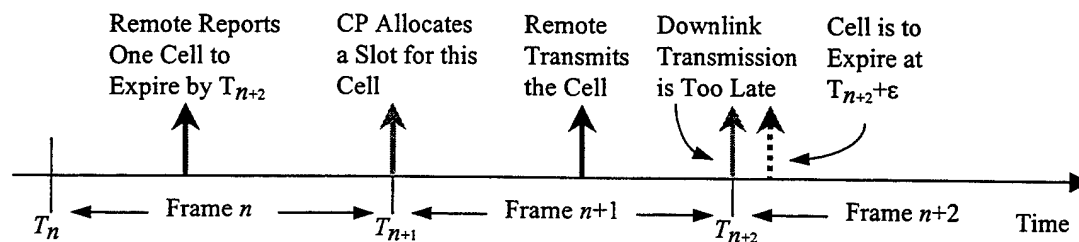
Figure VI.8: Cell Discarding in a Remote-to-Remote Connection when the Remote Reports the Cells to Expire by the End of the Next Two Frames
