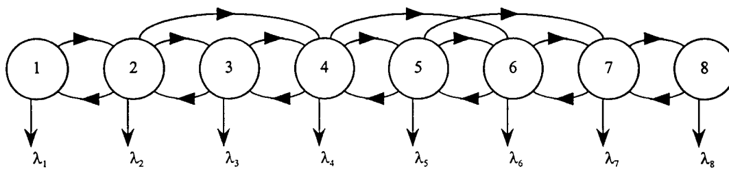
Figure IV.7: Eight-State MMPP Model of a Video Source; Selected Transitions [84]
