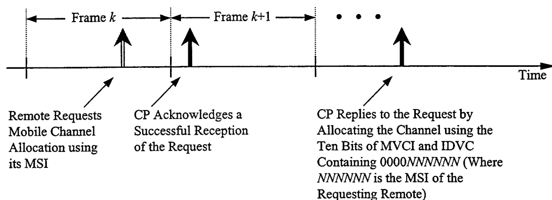
Figure III.4: Mobile-Channel Allocation Procedure for (Standard) ATM Signaling
