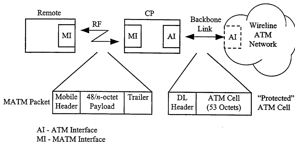
Figure II.13: Packet Formats in the Extended Integrates Services Network [76]
