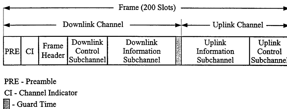
Figure VI.18: A Modified MAC Frame Format
