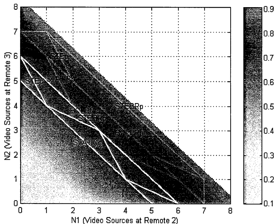
Figure VII.16: Admissible Region and Normalized Throughput for Partial- and Complete-Status Cases, Scenario 5
