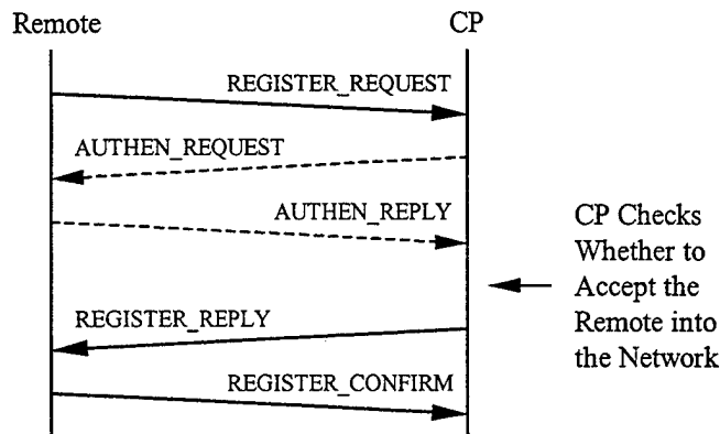
Figure III.5: Registration Procedure Diagram [101]
