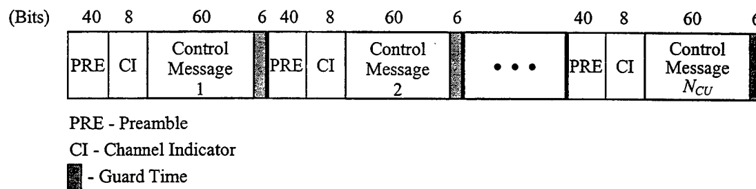
Figure III.18: Uplink-Control-Subchannel Frame Structure
