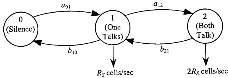
Figure IV.11: Three-State, Birth-Death, Voice-Conversion Model
