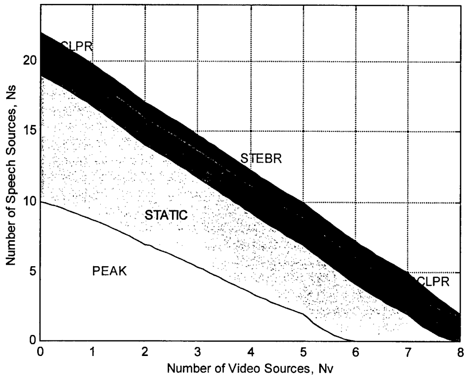
Figure V.21: Cut of the 3D Admissible Region at Zero Data Connections; N_D = 0
