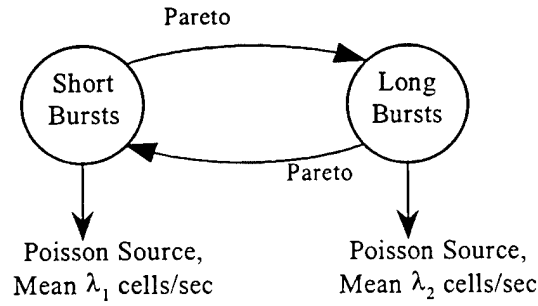
Figure IV.8: Switched Poisson Process with Heavy-Tail State Distribution [88]
