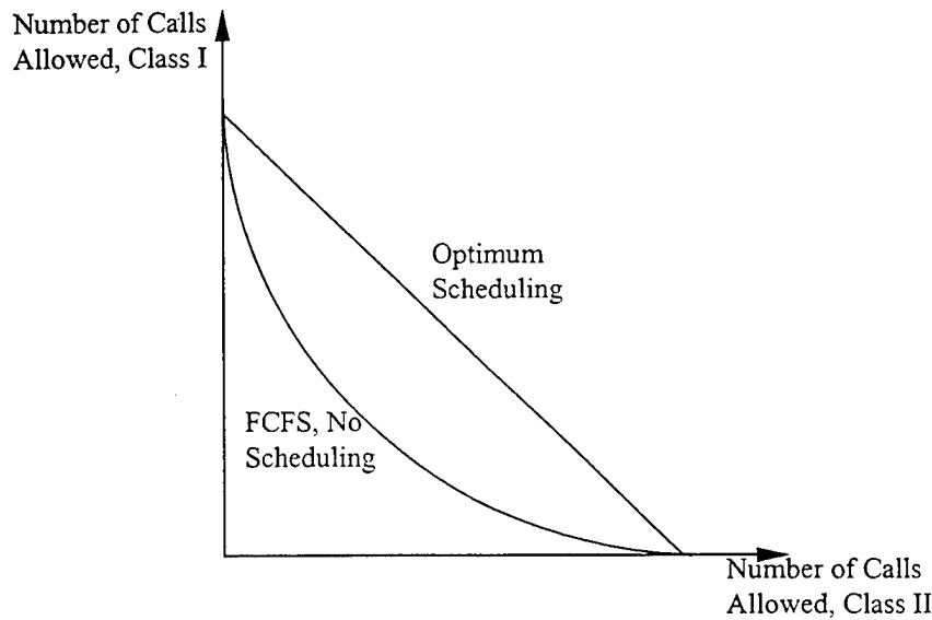
Figure II.4: Two-Class Admissible Region [80]
