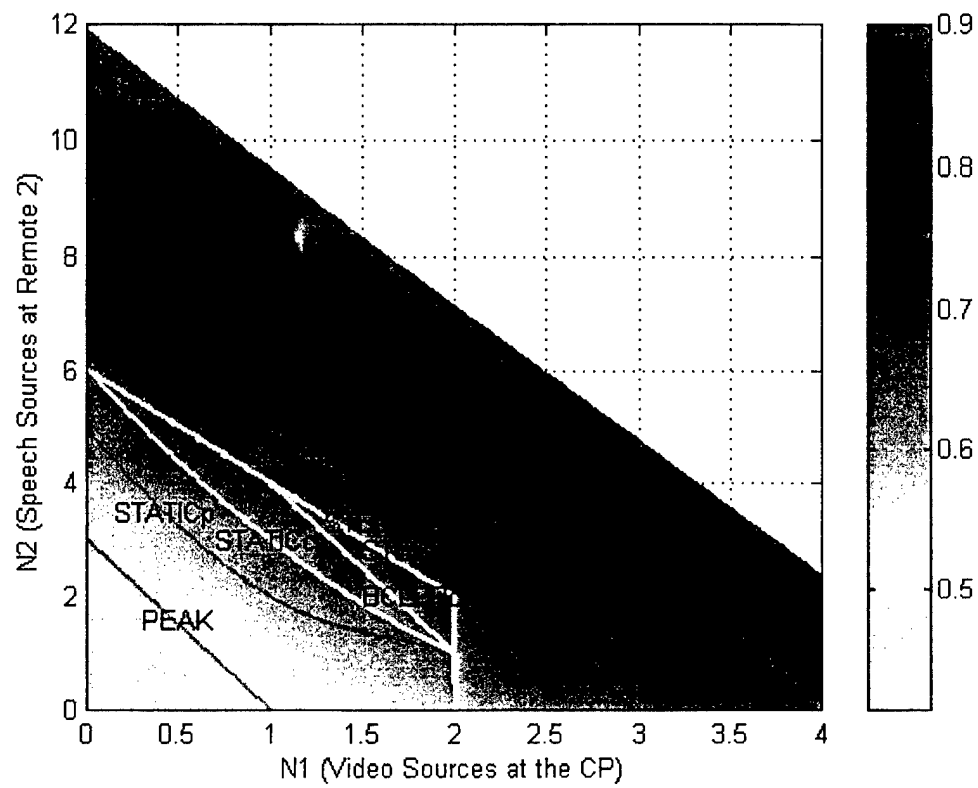
Figure VII.15: Admissible Region and Normalized Throughput for Partial- and Complete-Status Cases, Scenario 4
