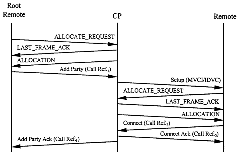
Figure III.9: Add-Party Procedure Diagram
