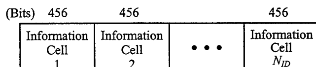
Figure III.16: Downlink-Information-Subchannel Frame Structure
