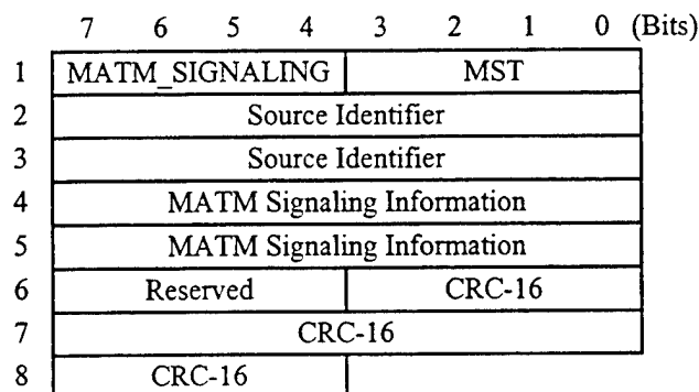
Figure III.15: MATM_SIGNALING Control Message
