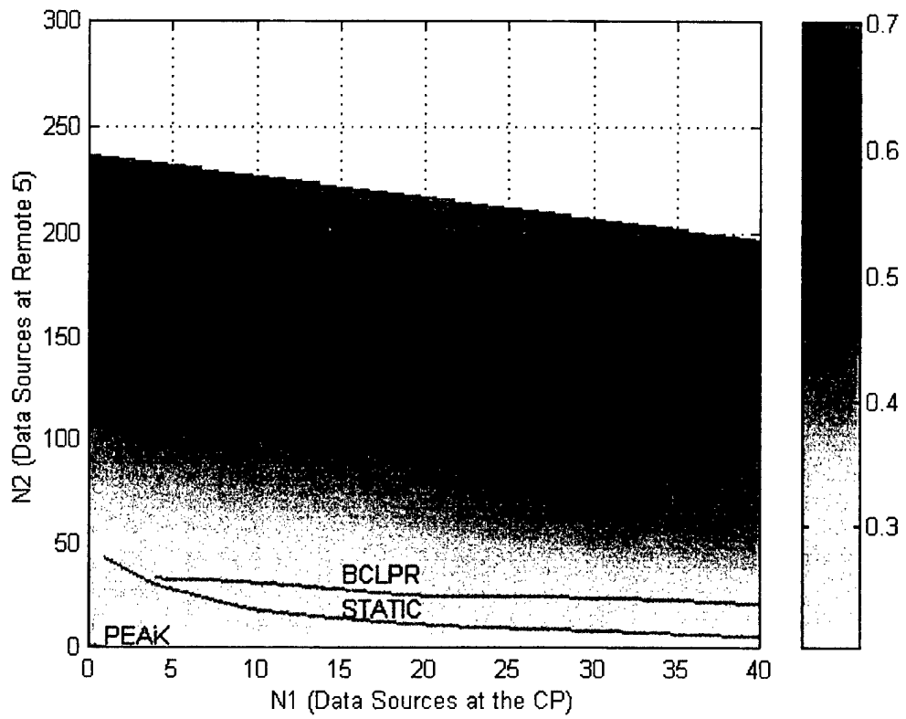
Figure VII.4: Admissible Region and Normalized Throughput for Partial Remote Status, Scenario 3
