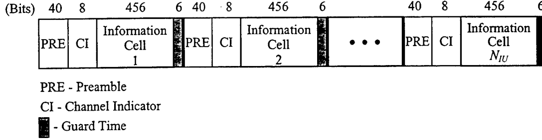
Figure III.20: Uplink-Information-Subchannel Frame Structure
