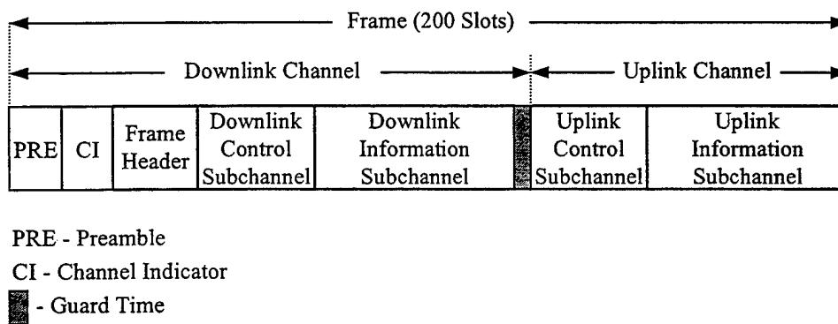
Figure III.11: MAC Frame Format
