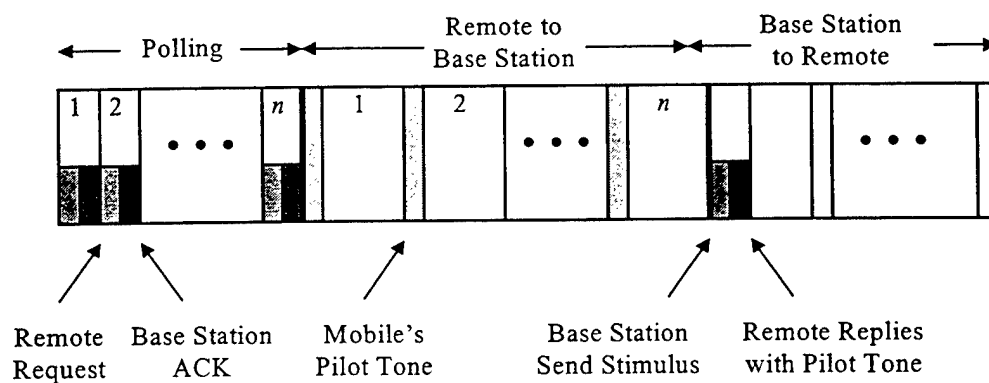
Figure II.7: Media Access Protocol Permitting Rapid Array Adaptation [2]
