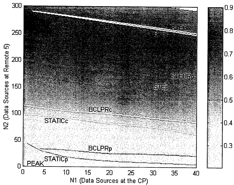
Figure VII.14: Admissible Region and Normalized Throughput for Partial- and Complete-Status Cases, Scenario 3
