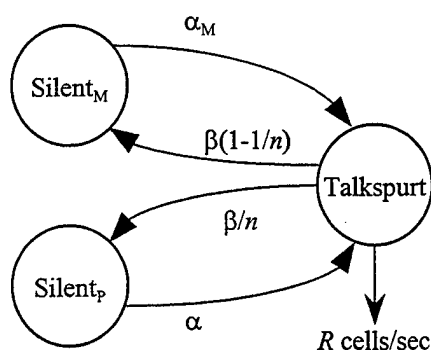
Figure IV.3: Voice Model Including Mini Gaps and Mini Talkspurts
