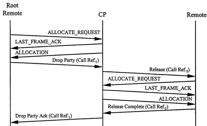
Figure III.10: Drop-Party Procedure Diagram
