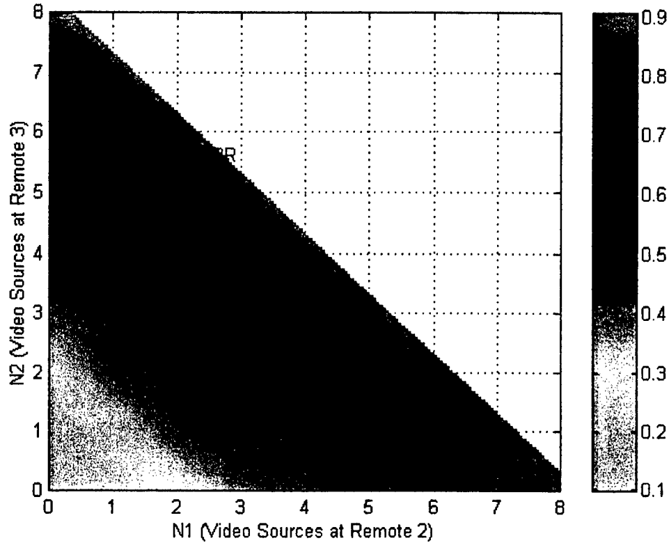
Figure VII.6: Admissible Region and Normalized Throughput for Partial Remote Status, Scenario 5
