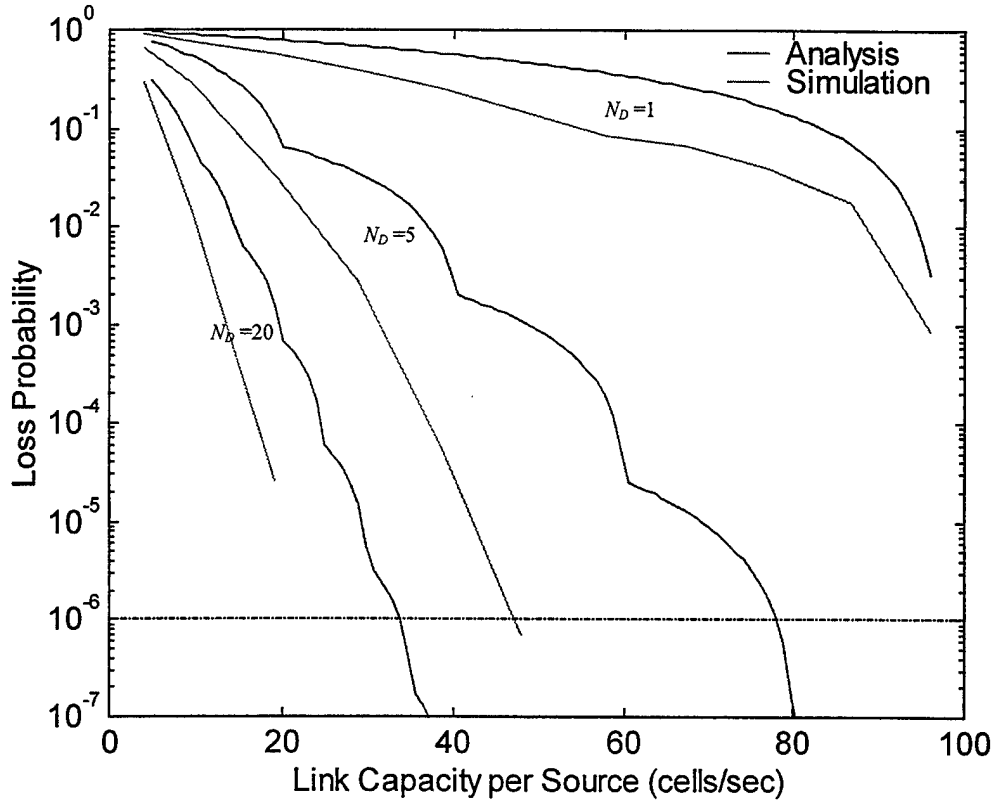
Figure V.6: Loss Probability for N_D Multiplexed Data Sources ( \max CTD_D = 1 Second)
