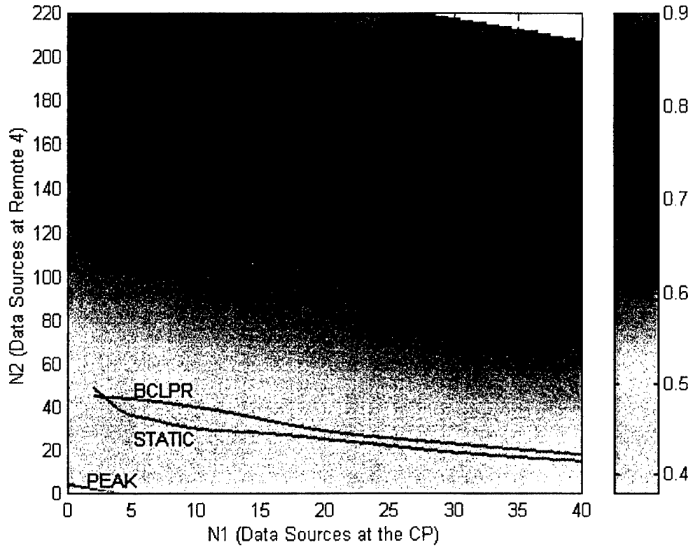
Figure VII.2: Admissible Region and Normalized Throughput for Partial Remote Status, Scenario 1
