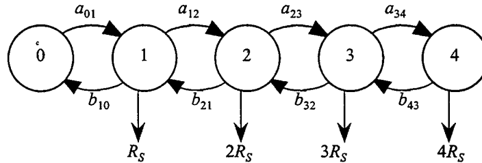
Figure IV.12: Aggregate Model for Two Conversations ( N_S = 2 )
