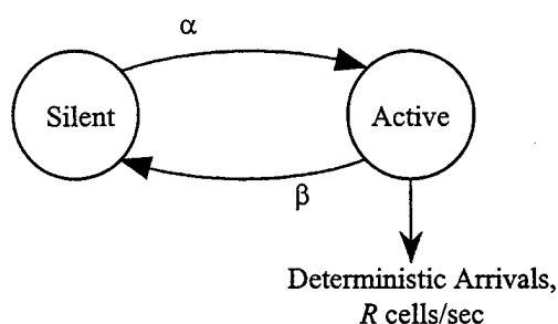
Figure IV.1: On-Off Model of a Voice Source [80]
