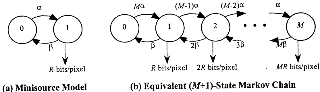
Figure IV.5: Multiple Minisources Model of a Video Source [82]
