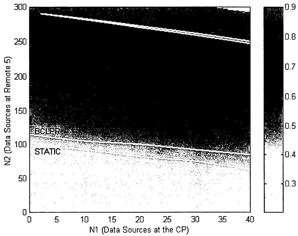
Figure VII.9: Admissible Region and Normalized Throughput for Complete Remote Status, Scenario 3
