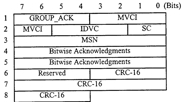
Figure III.19: GROUP_ACK Control Message
