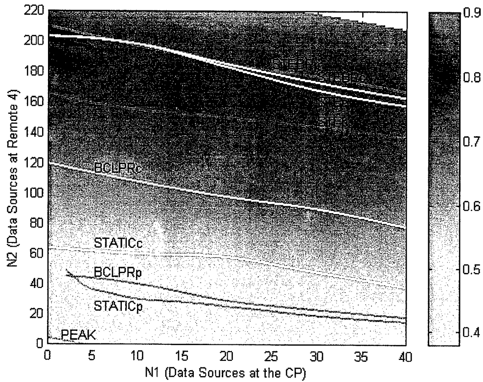
Figure VII.12: Admissible Region and Normalized Throughput for Partial- and Complete-Status Cases, Scenario 1
