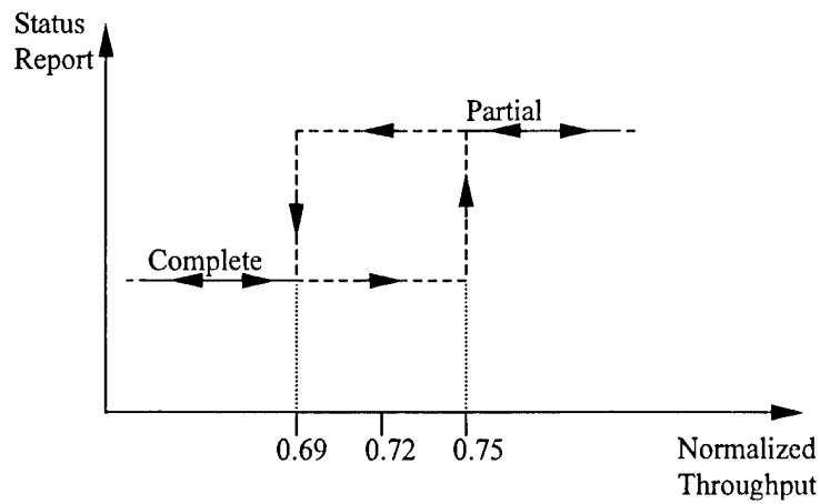
Figure VII.17: A Hybrid Scheme for the Scheduler Operation
