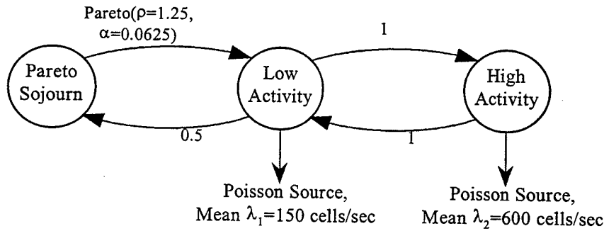
Figure IV.10: Hybrid Model for Self-Similar Traffic [48]
