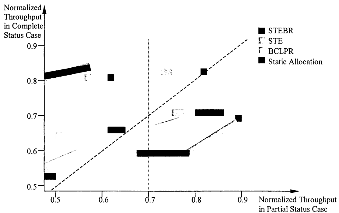
Figure VII.18: Normalized Throughput in Partial and Complete Status Reports
