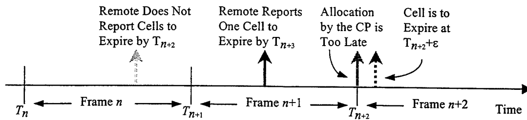
Figure VI.7: Cell Discarding in a Remote-to-CP Connection when the Remote Reports the Cells to Expire by the End of the Next Frame
