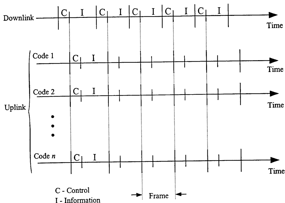
Figure VIII.2: MAC Architecture for Dynamic Allocation of PN Codes
