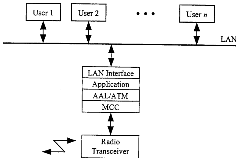
Figure II.10: General Architecture of a Mobile Station
