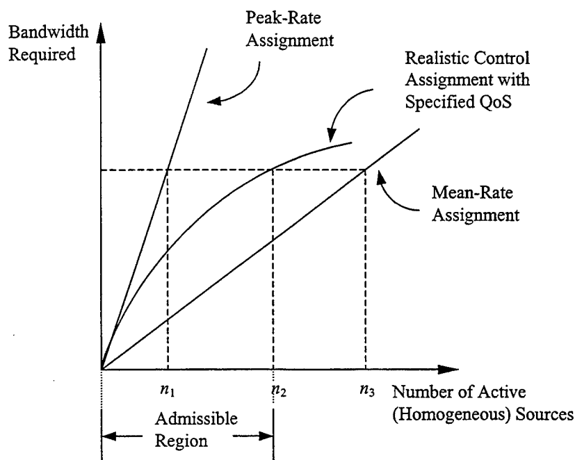
Figure II.5: Admission Control for Homogeneous ON-OFF Sources [80]
