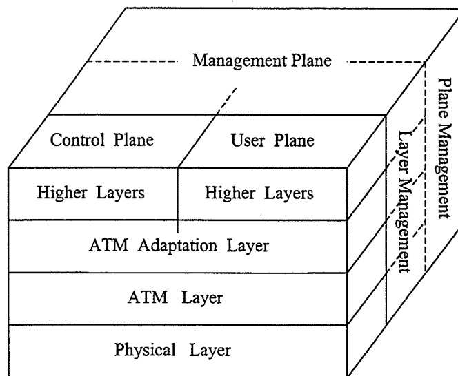
Figure II.1: B-ISDN Protocol Reference Model [40]
