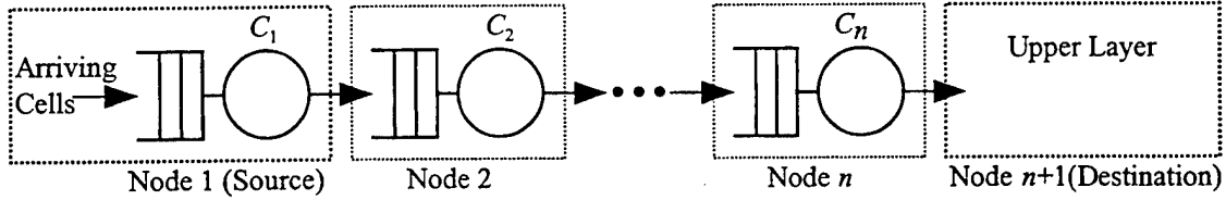
Figure VI.3: Queueing Model of a Multiple-Hop Connection
