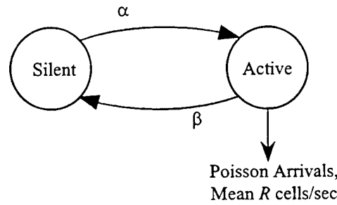
Figure IV.2: MMPP Model of a Voice Source [80]
