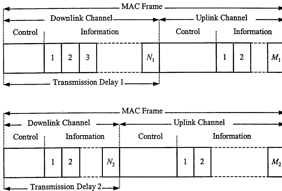
Figure VI.23: Variable Transmission Delays of Cells on the Downlink Channel
