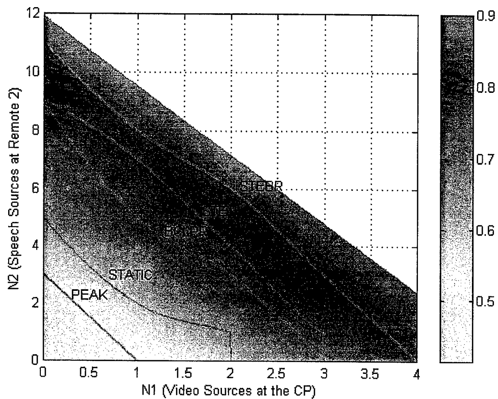
Figure VII.5: Admissible Region and Normalized Throughput for Partial Remote Status, Scenario 4
