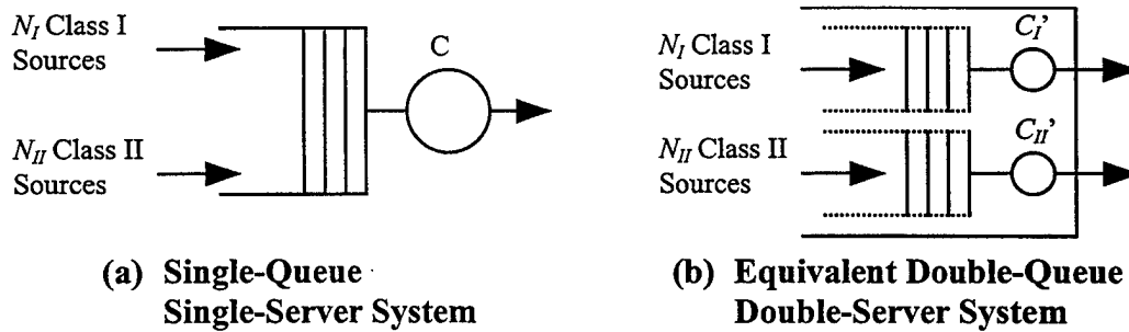
Figure V.8: Treatment of a Two-Class-Input, Single-Queue, Single-Server System as a Double-Queue Double-Server System
