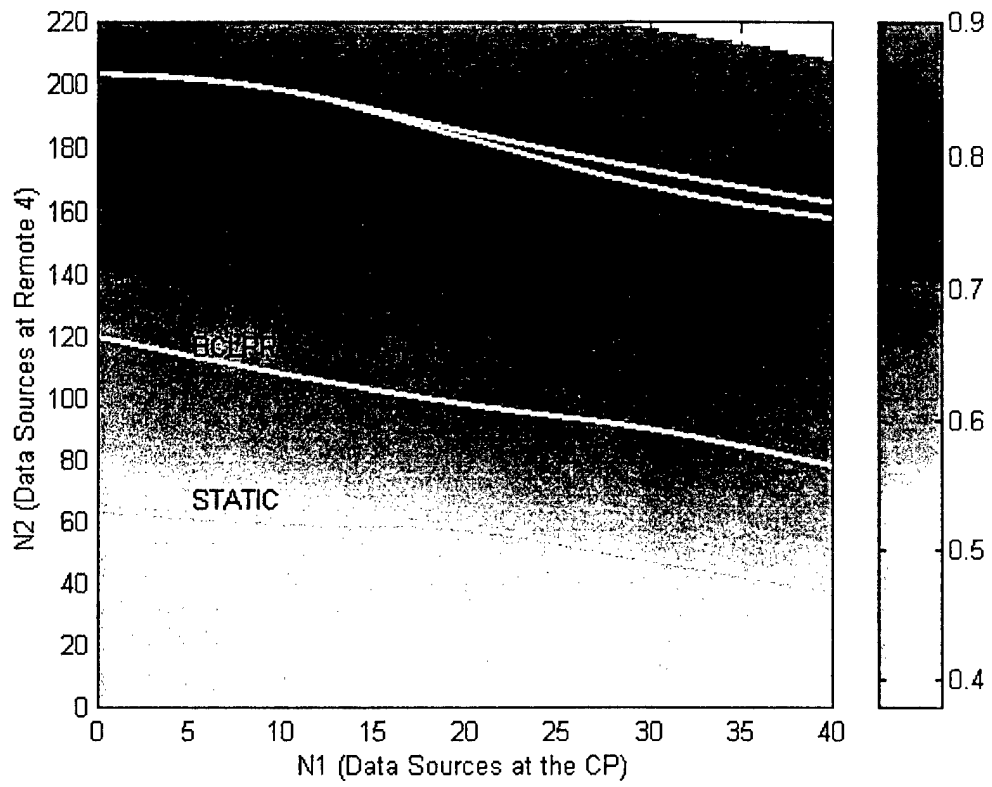
Figure VII.7: Admissible Region and Normalized Throughput for Complete Remote Status, Scenario 1
