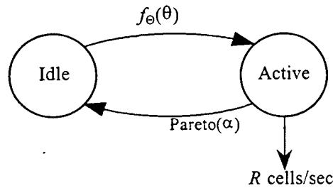
Figure IV.9: Self-Similar Process as an Aggregation of M On-Off Sources ( M \gg 1 ) [58]
