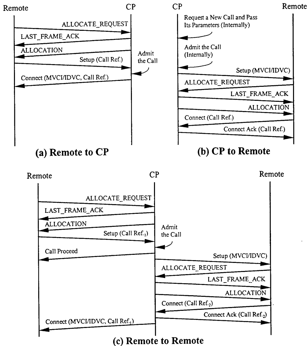
Figure III.7: Call-Setup Procedure Diagrams
