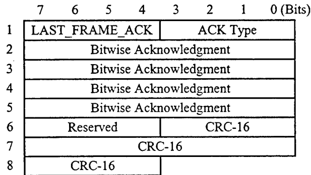
Figure III.14: LAST_FRAME_ACK Control Message
