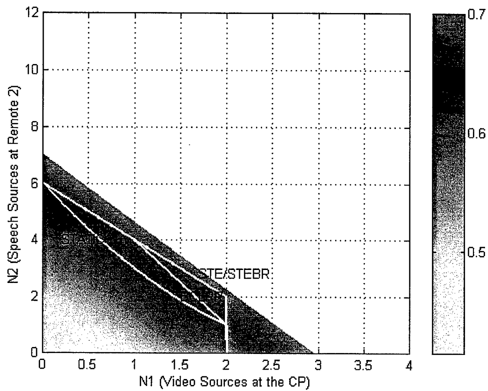
Figure VII.10: Admissible Region and Normalized Throughput for Complete Remote Status, Scenario 4
