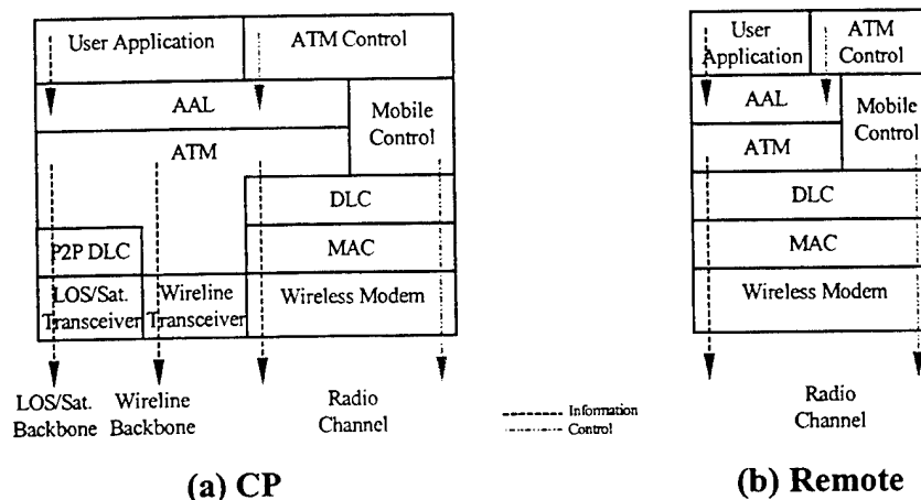
Figure II.14: Protocol Layering in a Wireless ATM Network
