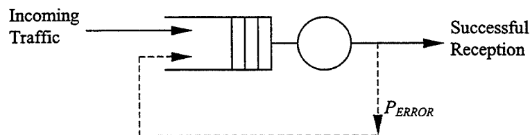
Figure VIII.3: Queueing Model of a Mobile Node in a Noisy Channel Environment
