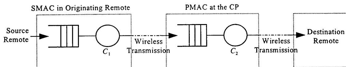
Figure VIII.1: Remote-to-Remote Connection Represented as Two Serial Queues
