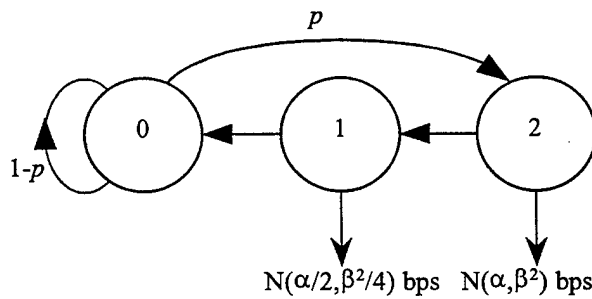
Figure IV.6: Three-State Markov Chain ( K_n ) Modeling Scene Changes
