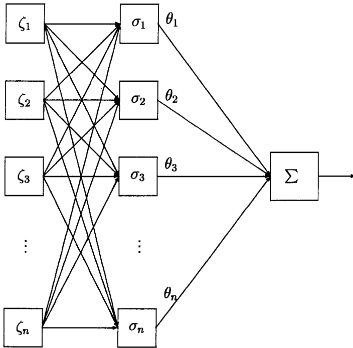
Figure 2: A feed-forward neural network
