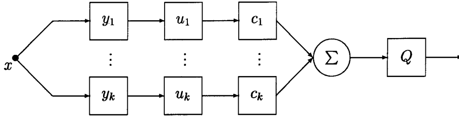
Figure 6: A classifying network
