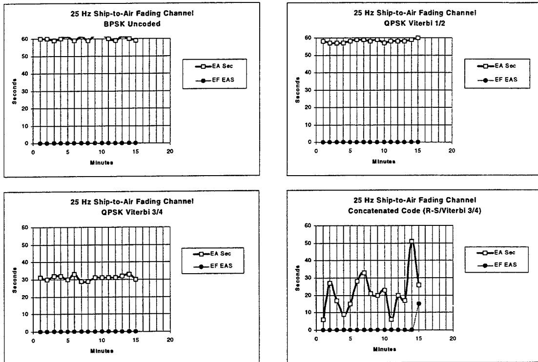
Figure 19. Standard ship-to-air channel results (fade rate = 25 Hz).
