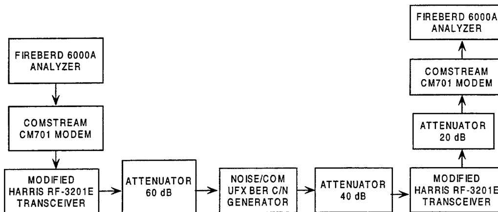
Figure 1. Equipment setup for baseline performance.
