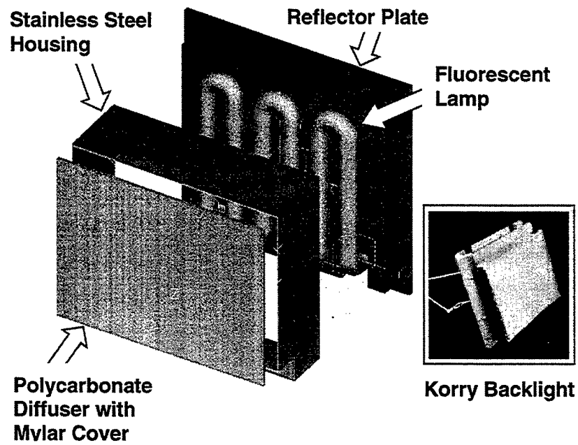
Figure 2-8 Exploded View of Backlight Components
