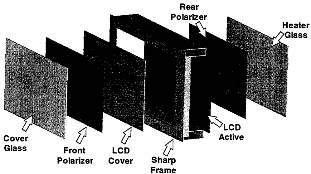
Figure 2-9 Exploded View of Backlight Components
