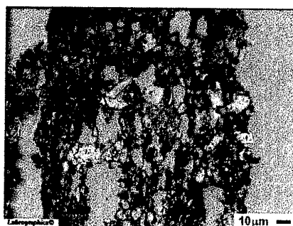
Fig 4 (a) Lead/Tin particles on a ferrogram
