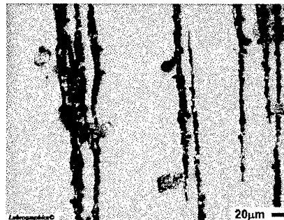
Fig 5 (b) Copper particles on a ferrogram
