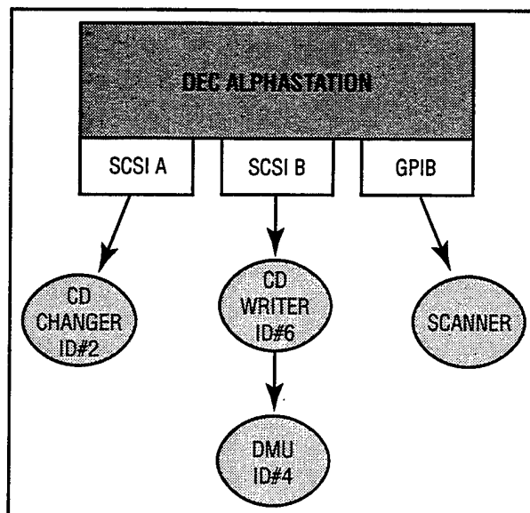
Fig. 2 — AV-8B MAP-II SCSI and GPIB connections
