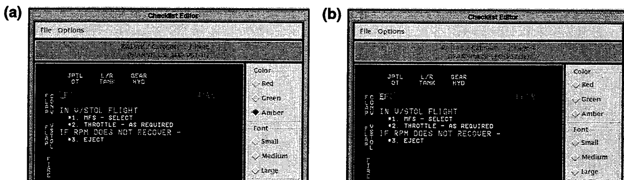
Fig. 44 — Example of changing text color in MMC checklist editor: (a) click on new color (e.g., amber) then (b) click on letter to change (e.g., from red)
