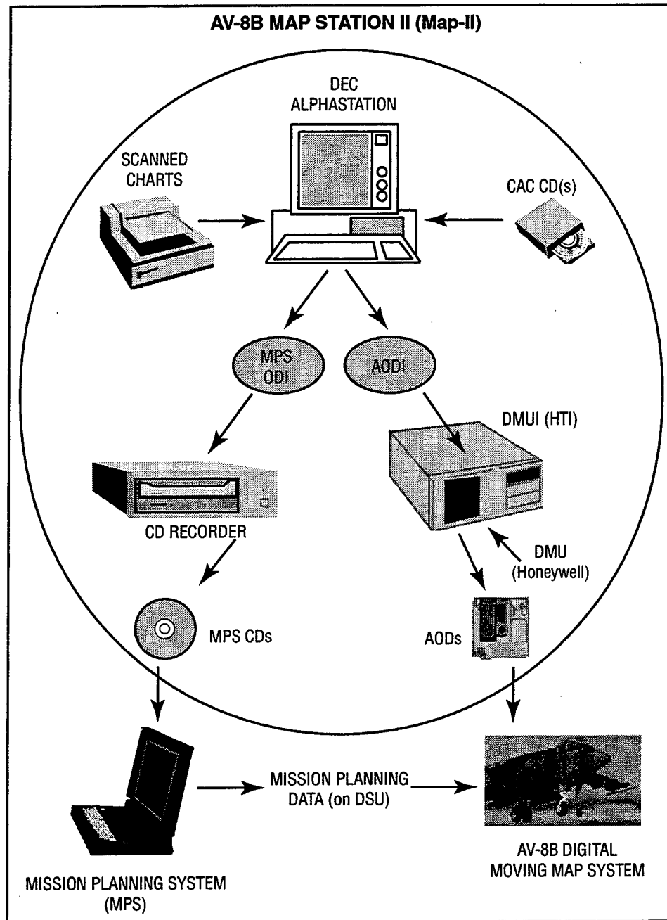
Fig. 1 — AV-8B MAP-II hardware components
