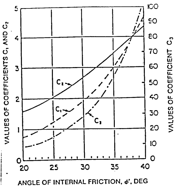
Fig. 79. Coefficients and function of \phi' . (after API RP2A, 1993)
