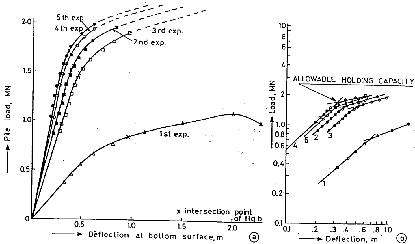
Fig. 78. Load-deflection diagram. (after Hogervorst, 1980)
