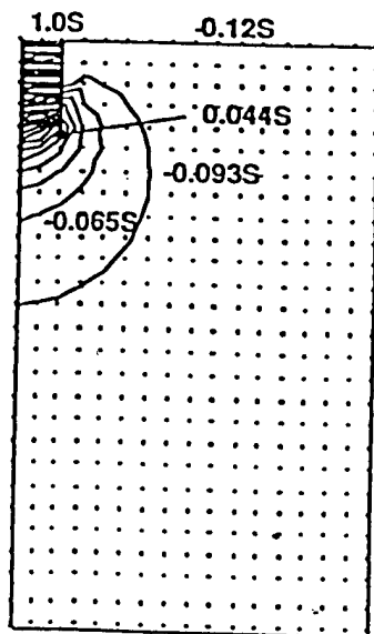
Fig. 36. Pore pressure distribution (steady state). (after Iskander et al., 1993)
