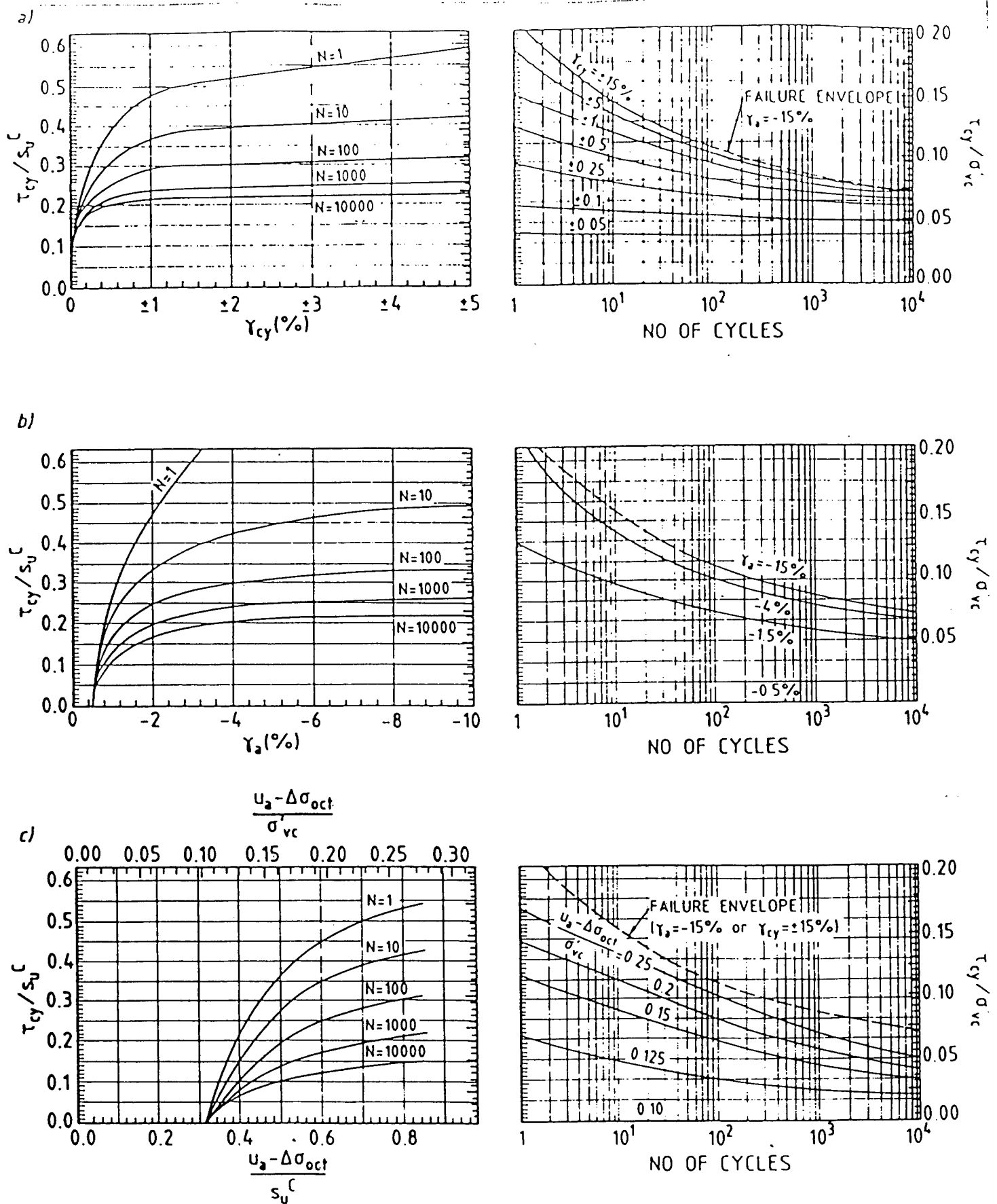
Figure 58. Contour diagram for triaxial tests with \tau_a = 0 on Drammen clay with OCR = 1: (a) cyclic shear strains, (b) average shear strains, (c) average pore pressures. (after Andersen and Lauritzen, 1988)
