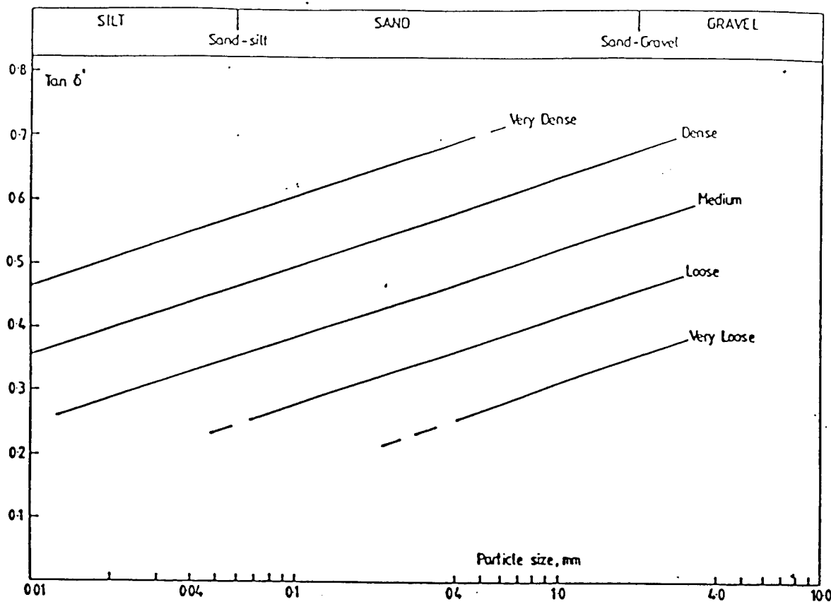
Fig. 7. Graphical interpretation of API recommended \delta' values in granular soils (after Jardine et al., 1993)
