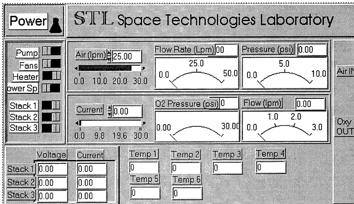
Figure 15. LabView interface.
