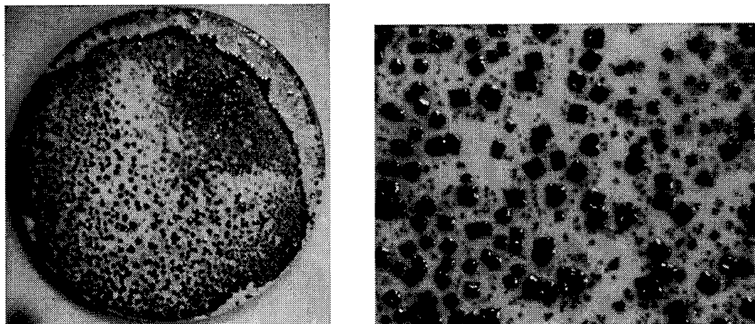
Figure 1. Optical micrograph of glass seal (GS004) and high magnification of crystallites in glass. Largest crystallites are \approx 100\text{ }\mu\text{m} .
