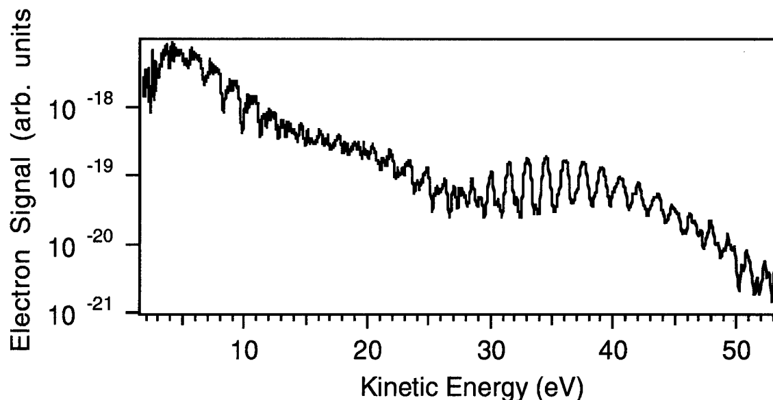
Fig. 1. High resolution photoelectron spectrum of xenon taken at 1.51 \times 10^{14} W/cm 2 .
