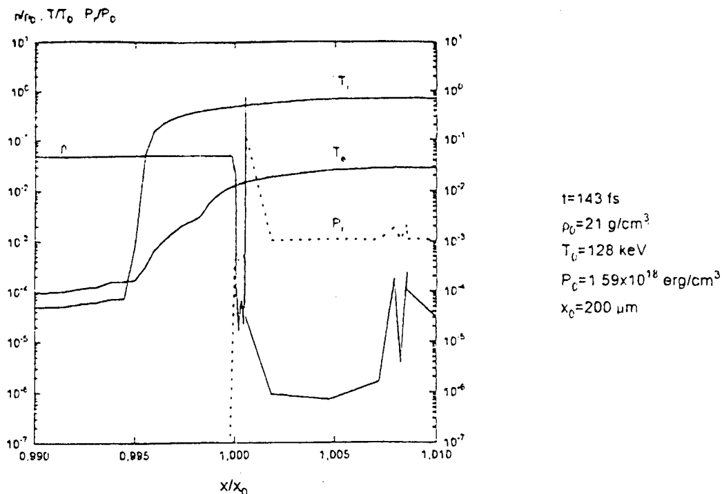
Fig 1. Hydro code simulations of the electron and ion temperatures T_e and T_i , and the plasma density \rho , and pressure, P .
