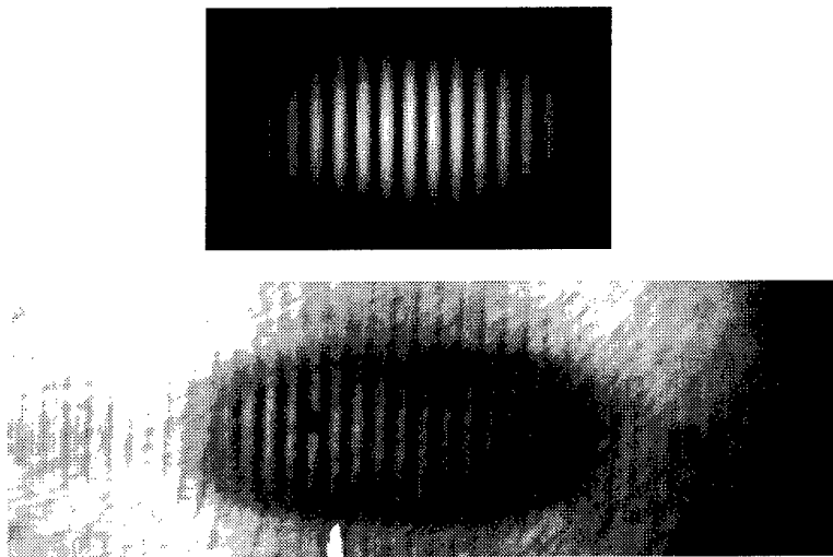
Figure 1 Above is the computed form of a 1D optical mode pattern of 15 micron wavelength used to drive a 2 micron thick Al foil at 210^{13} Wcm -2 . Below is a Ge XUV laser radiograph with 50 ps exposure time recorded after 500 ps of drive. It shows perturbations induced in the foil which correspond to 5% variations in its thickness
