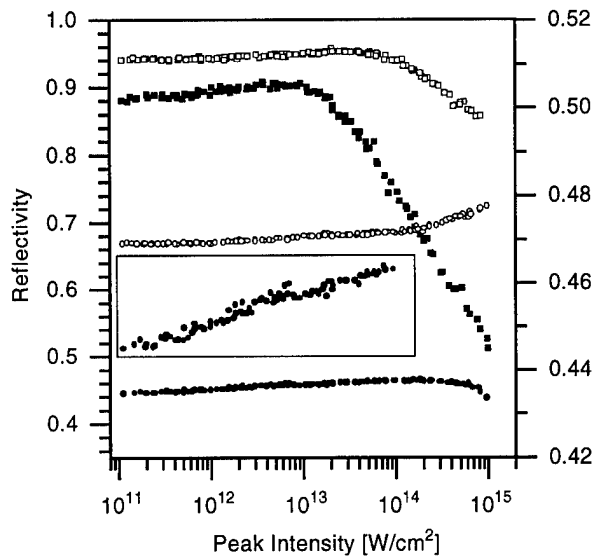
Figure 1: Reflectivity of 120 fs pulses from Al and Fe surfaces vs. peak pulse intensity, at a 45° angle of incidence. Al data are shown with squares, Fe with circles. Measurements with polarization parallel to the plane of incidence (p-pol.) are shown with filled points; open points are used for polarization perpendicular to the plane of incidence (s-pol.). A section of the Fe, p-polarized data is shown in the inset, magnified vertically as indicated by the right-side axis.
