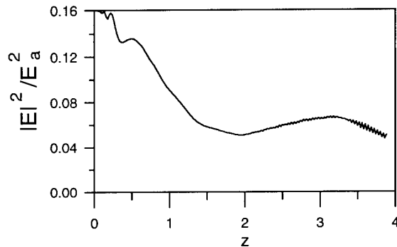
Fig.4 Field intensity at the axis of the channel in the middle of the temporal profile of the pulse as a function of propagation distance z measured in Rayleigh lengths.
