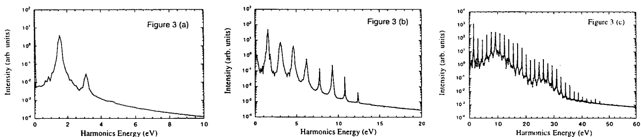
Figure 3 : harmonics spectra for For I=1 \times 10^{10} W/cm 2 , 5 \times 10^{11} W/cm 2 and 1 \times 10^{13} W/cm 2
