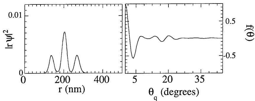
Fig.2. A three-peaked "tailored" wave packet at the target time (left panel) and its form factor (right panel). The wavelength is assumed to be 22.2 nm.
