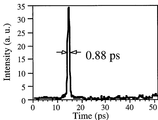
Figure 1: The 0.88 ps time-response of our streak camera using femtosecond x-rays at 17 nm produced by high-harmonic generation.
