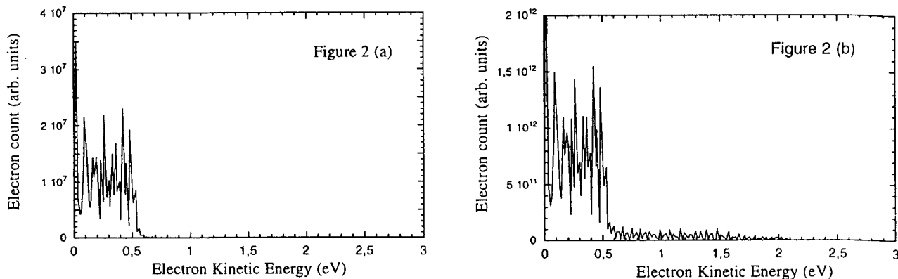
Figure 2 : electron spectra for For I=1 \times 10^{10} W/cm 2 and For I=5 \times 10^{11} W/cm 2
