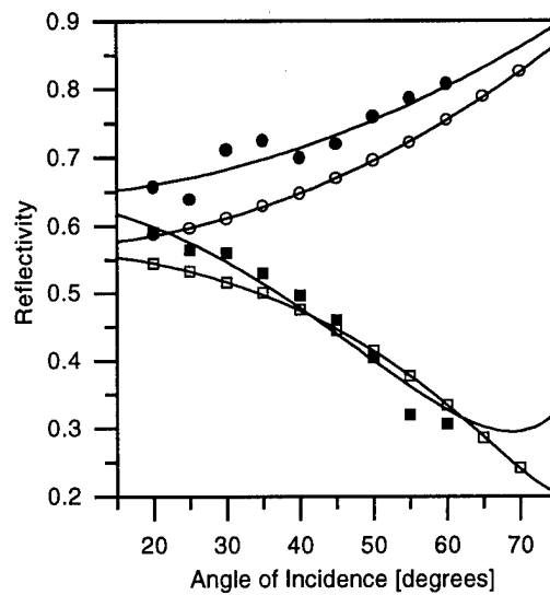
Figure 2: Reflectivity of Fe vs. angle of incidence at I = 10^{11} W/cm 2 (open points) and 2 \times 10^{14} W/cm 2 (filled points) for s-polarization (circles) and p-polarization (squares). The reflectivity of a density gradient calculated from the corresponding best fit results are shown with lines.
