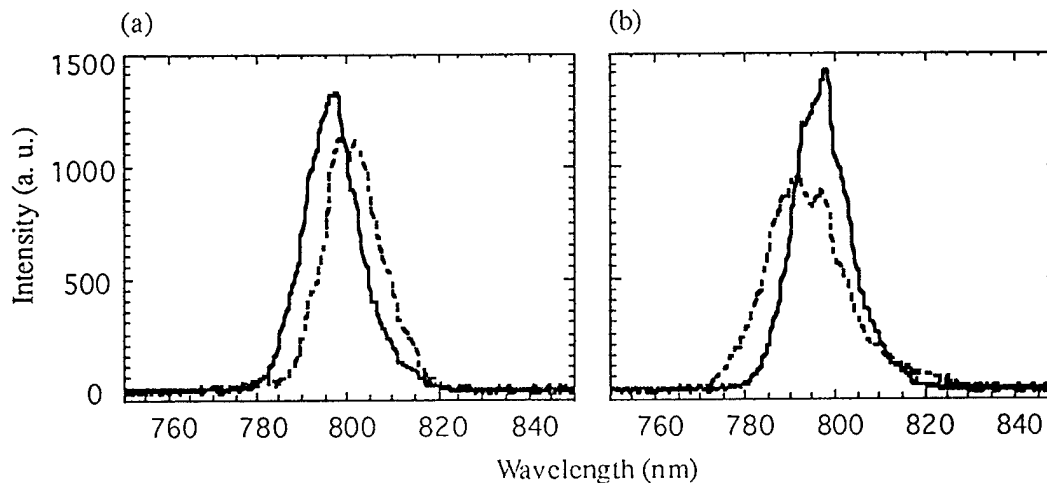
Figure 2: Experimental spectra of the probe beam from the Ti:sapphire chain at different time delays, without the pump beam (solid line) and in presence of the pump beam (dashed line).
