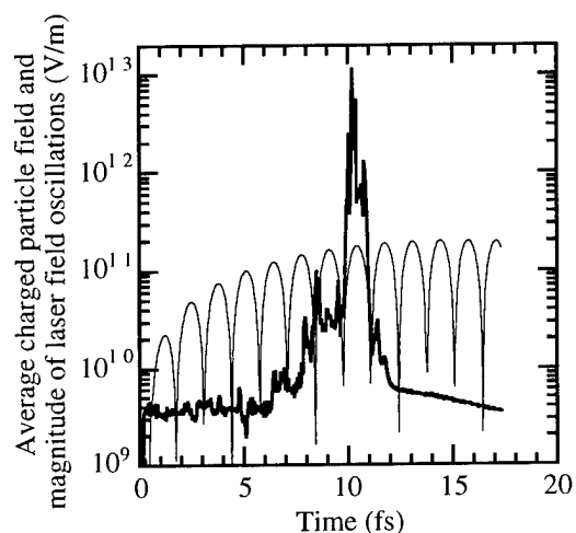
Fig.3: Average electric field from other ions and ionized electrons at the position of the nuclei of a 25-atom argon cluster. The cluster is illuminated by a 800 nm, 15 fs laser pulse with a peak intensity of 5 \times 10^{15} \text{ W/cm}^2 whose electric field oscillations are drawn as a thin line. Note the logarithmic scale.
