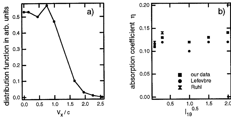
Figure 1: a) distribution function for normal incidence. x/l_s = 3 , \omega_0 t = 180 . b) absorption coefficient \eta as a function of the square-root of laser intensity in units of 10^{19}W/cm^2 .
