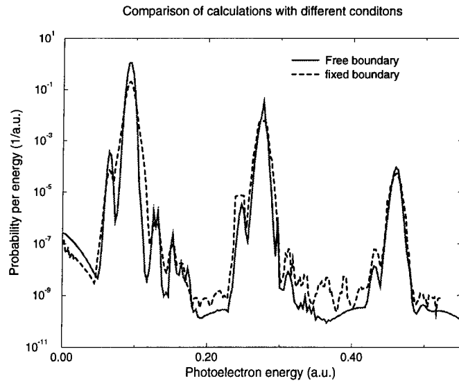
Figure 1: Comparison of calculations with different boundary conditions. I = 10^{12} W/cm^2 , \hbar\omega = 5 eV.
