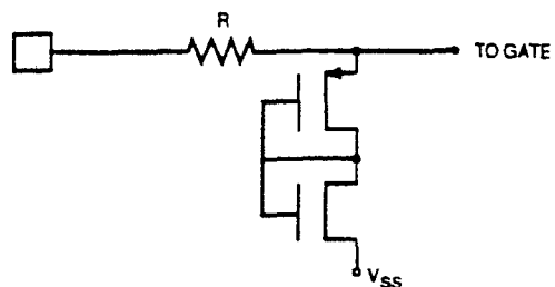
e. Transistor Bilateral Devices
