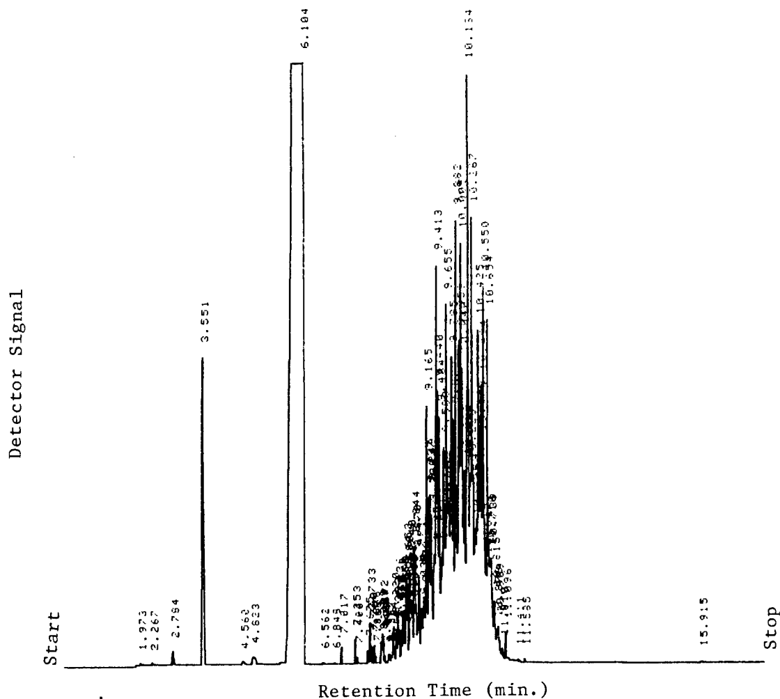
Figure 3 Gas Chromatograph and Peak Integration of RP-1/Quadricyclane
