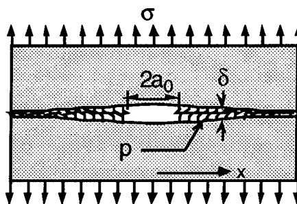
Figure 2. Crack-face spring bridging.
