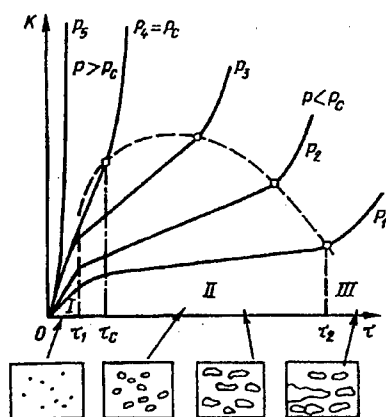
Figure 1. Typical time dependences of a characteristics ( K ) of deformation and/or fracture for different values of a parameter P governing the loading conditions : I, II, III — stages of damage accumulation.
