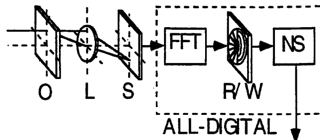
Fig. 2. All-digital recognition system shown in dashed box, including software embodiment for FFT, ring-wedge data format, and neural software.
