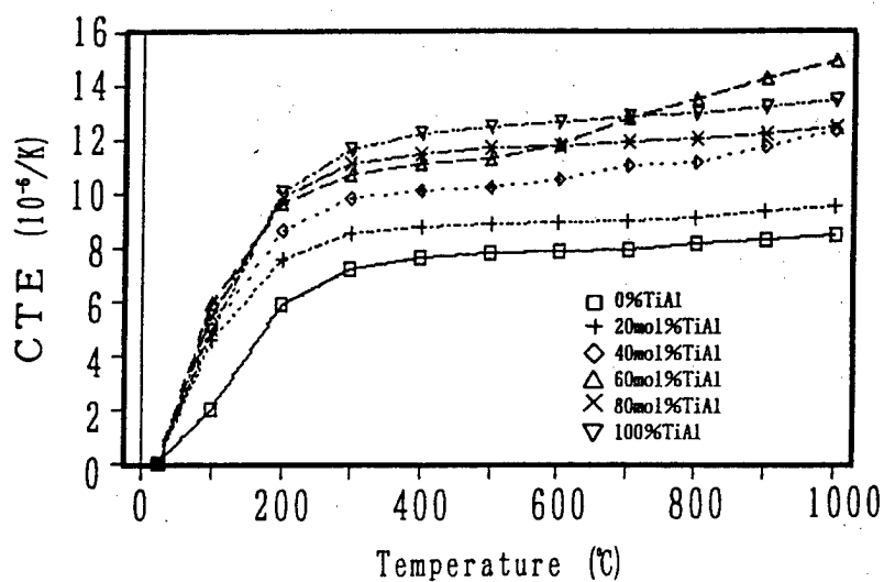
Average Thermal Expansion Coefficient of NFGMs
