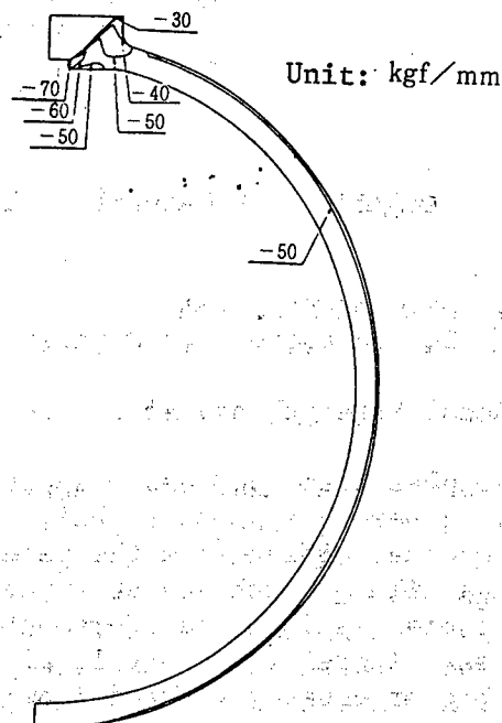
Figure 4. Stress Contour Along Latitude Section (External pressure 680 \text{ kgf/cm}^2 )
