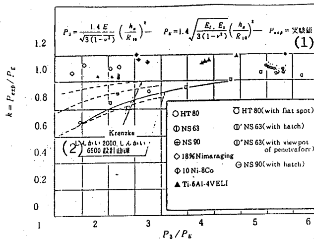
Figure 2. Compressive Strength for Spherical Pressure Hull
