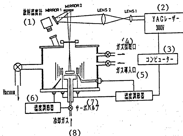
Figure 3. Temperature Gradient-Added Sintering Device
