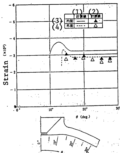
Figure 13. Longitudinal Strain Distribution Around Viewport Coaming (external pressure 680 kgf/cm²)
