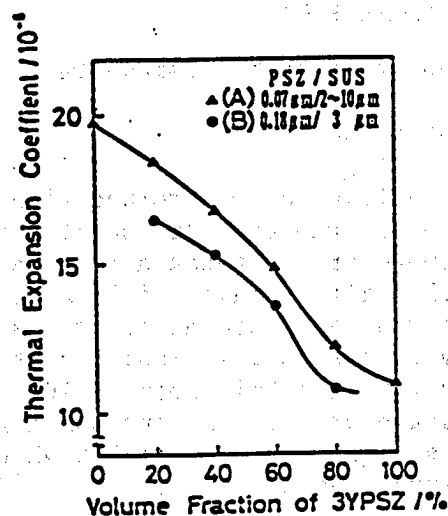
Figure 7. Relationship Between Thermal Expansion Coefficient and Composition for Zirconia/Stainless Steel-Base Sintered Mixture
