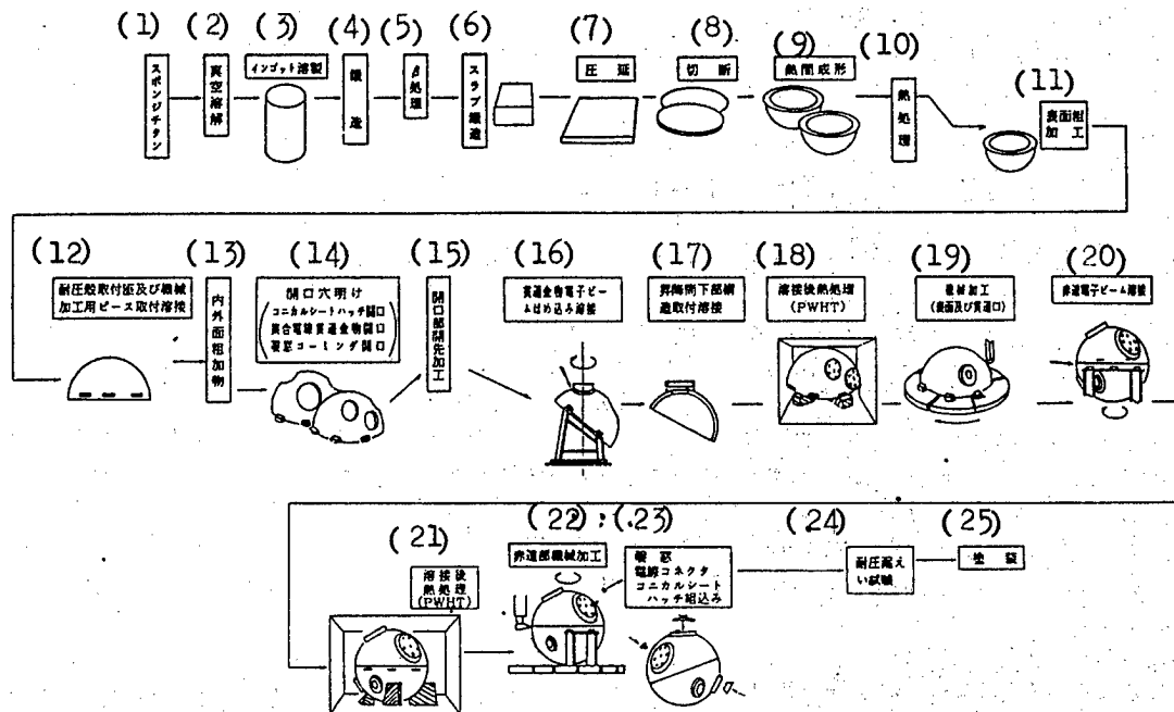
Figure 6. Production Procedure of Pressure Hull
