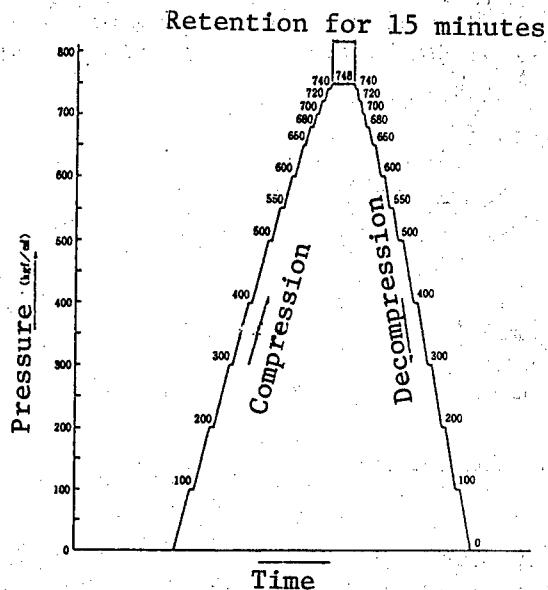
Figure 10. Procedure of Compression and Decompression
