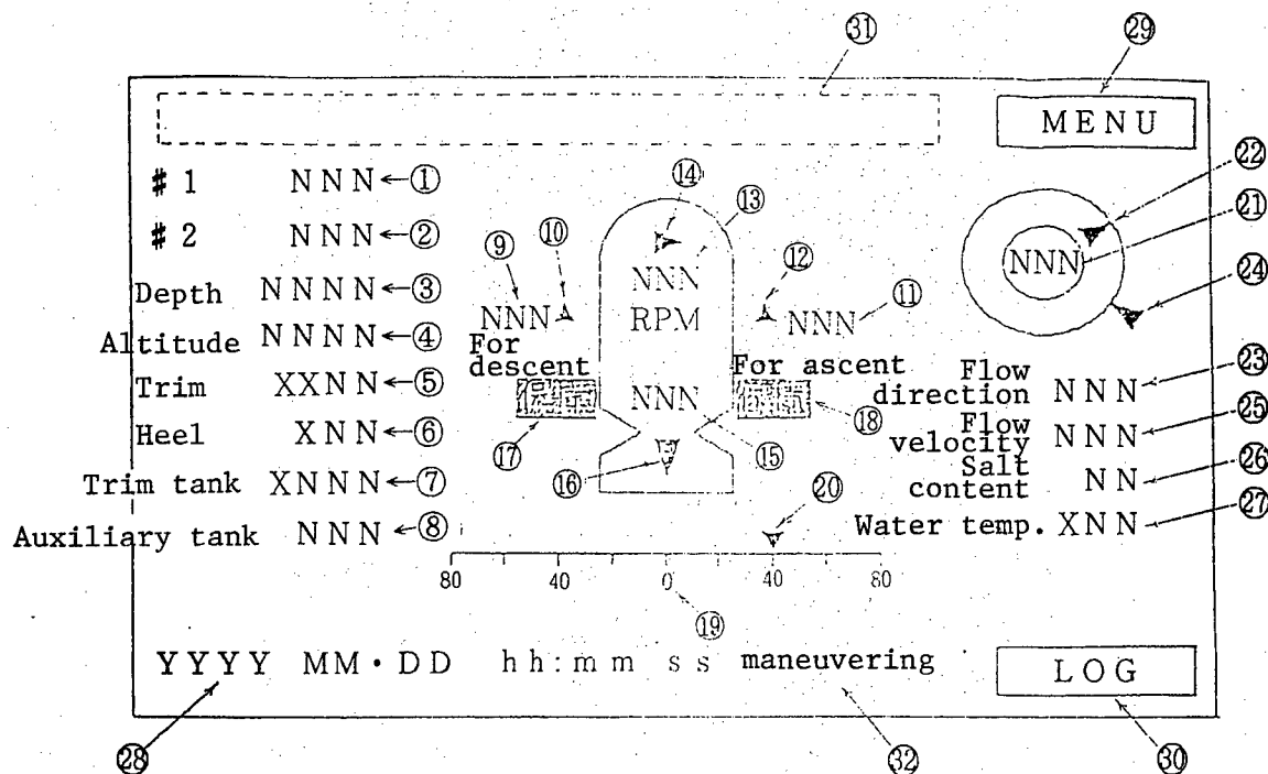
Figure 7. Display Pattern of Maneuvering Mode
