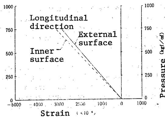
Figure 12. Stress-Strain Transition (Bottom of Viewport Coaming)
