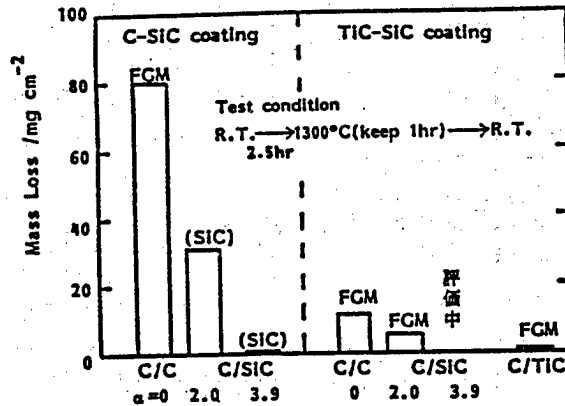
Figure 15. Antioxidation Stability of Various Coated Carbon Fiber-Reinforced Composites
