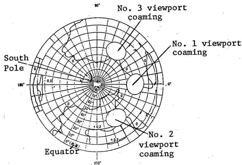
Figure 8. Sphericity Deviation (Radius) Distribution of S-Hemisphere
