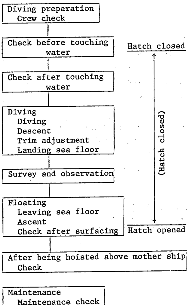
Figure 5. Operation Flow and Corresponding Software
