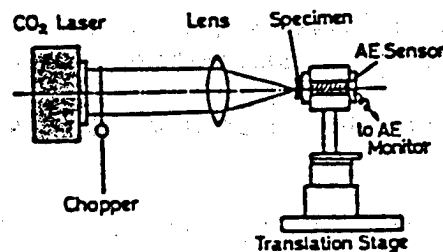
Figure 12. Schematic Presentation of Laser Thermal Shock Test for Thermal Shock Resistance Evaluation of FGMs
