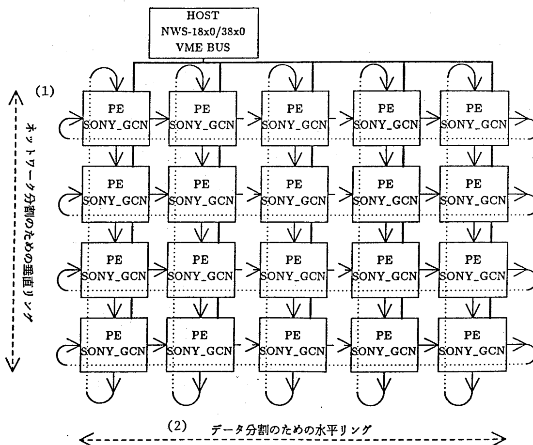
Figure 3. Net Data Division Method Over Mesh Connected GCN
