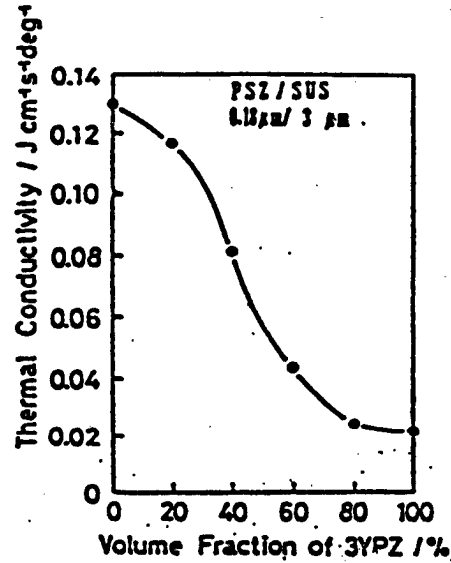
Figure 8. Relationship Between Thermal Conductivity and Composition for Zirconia/Stainless Steel-Base Sintered Mixture
