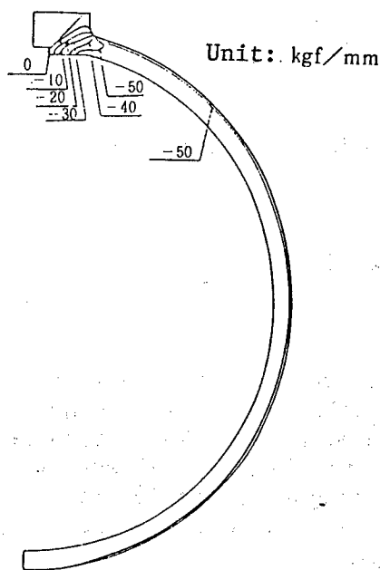
Figure 3. Stress Contour Along Longitude Section (External pressure 680 \text{ kgf/cm}^2 )
