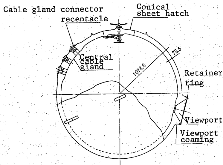
Figure 1. Structure of Pressure Hull
