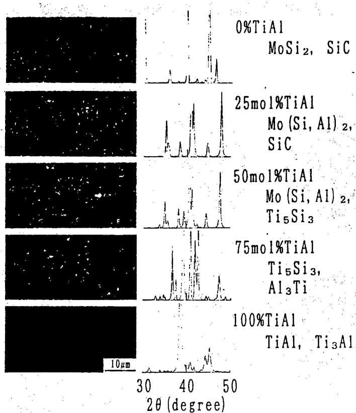
Microstructure and X-Ray Composition of NFGM
