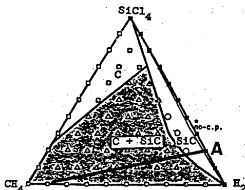
Figure 2. Equilibrium Precipitation Phase Diagram for \text{SiCl}_4 - \text{CH}_4 - \text{H}_2 System (at 1,400^\circ\text{C} and 60 torr)
