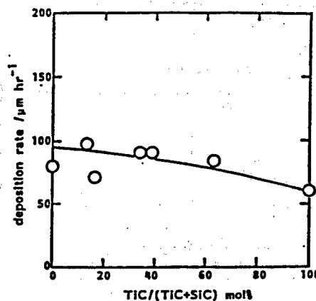
Figure 11. Relationship Between Precipitated Layer Composition and Precipitation Speed
