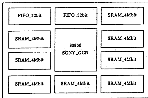
Super-chip for GCN
