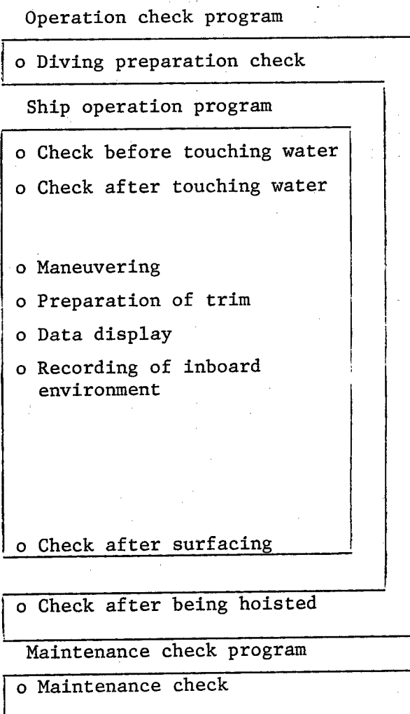
Figure 5. Operation Flow and Corresponding Software
