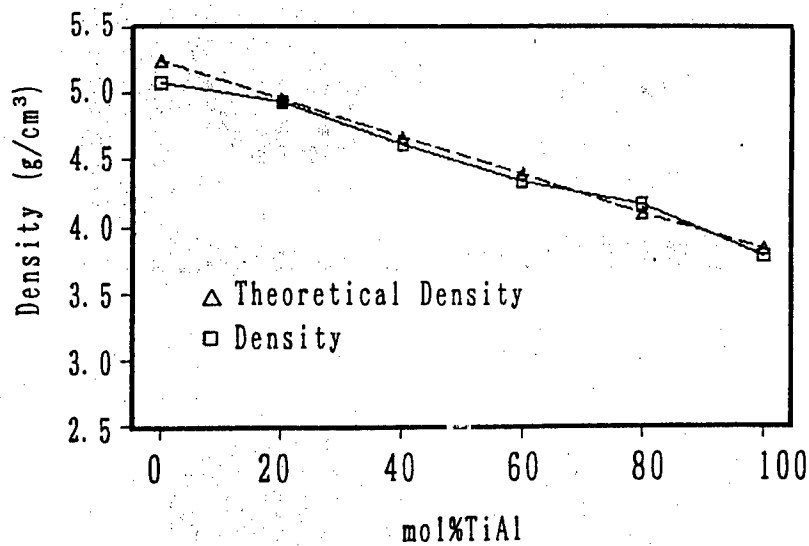
Density of (MoSi 2 -SiC)-TiAl (0 to 100 weight percent) (NFGM)
