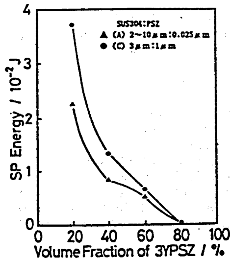
Figure 11. Transition from Pliability to Brittleness With Compositional Change in Zirconia/Stainless Steel-Base Sintered Mixture
