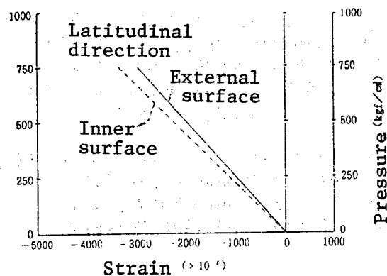
Figure 11. Stress-Strain Transition (General Part of Hull)
