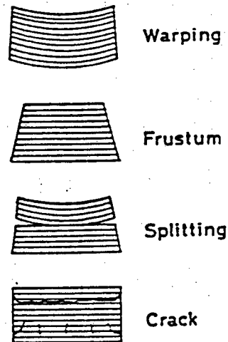
Figure 4. Flaws Created by Sintering Imbalance
