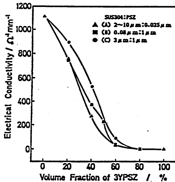
Figure 9. Relationship Between Electrical Conductivity and Composition for Zirconia/Stainless Steel-Base Sintered Mixture
