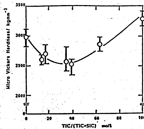
Figure 13. Relationship Between Precipitated Layer Composition and Hardness
