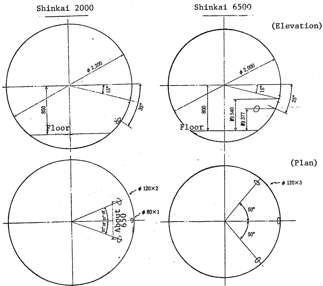
Figure 2. Comparison of the View Port Location
