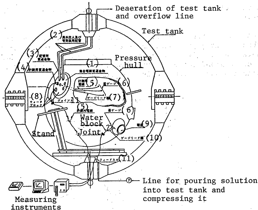
Figure 9. Arrangement of Pressure Test in DTRC
