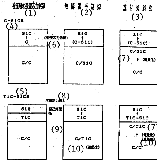
Figure 1. Conceptual Diagrams for Compositional Gradient Coating and Functional Gradient Matrix Formation To Produce Super Heat Resistant Structural Material
