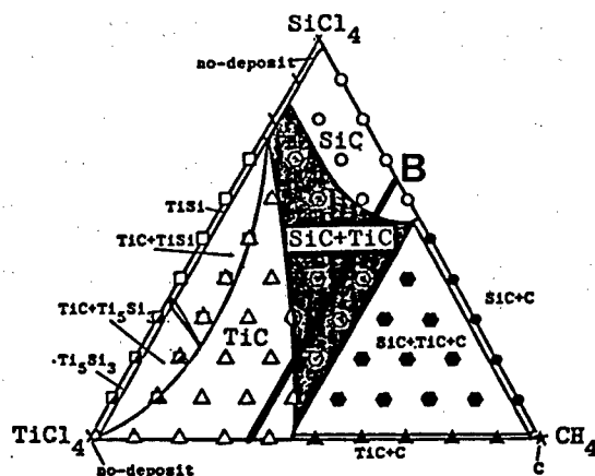
Figure 9. Equilibrium Precipitation Phase Diagram for \text{SiCl}_4 - \text{TiCl}_4 - \text{CH}_4 - \text{H}_2 System (at 1,350°C and 60 torr)
