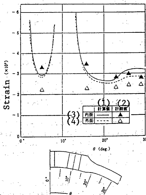
Figure 14. Latitudinal Strain Distribution Around Central Watertight Cable Gland (external pressure 680 kgf/cm²)
