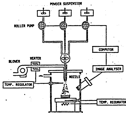
Figure 2. Particle Spouting Arrangement Device for Compositional Gradient Formation
