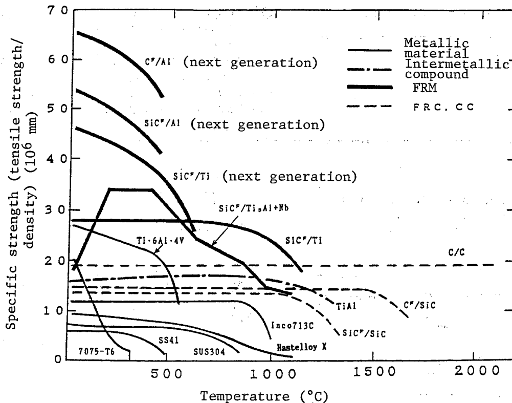
Relationship Between Specific Strength and Temperature of Prospective Low Temperature Side Materials of Thermal Stress Alleviating FGMs
