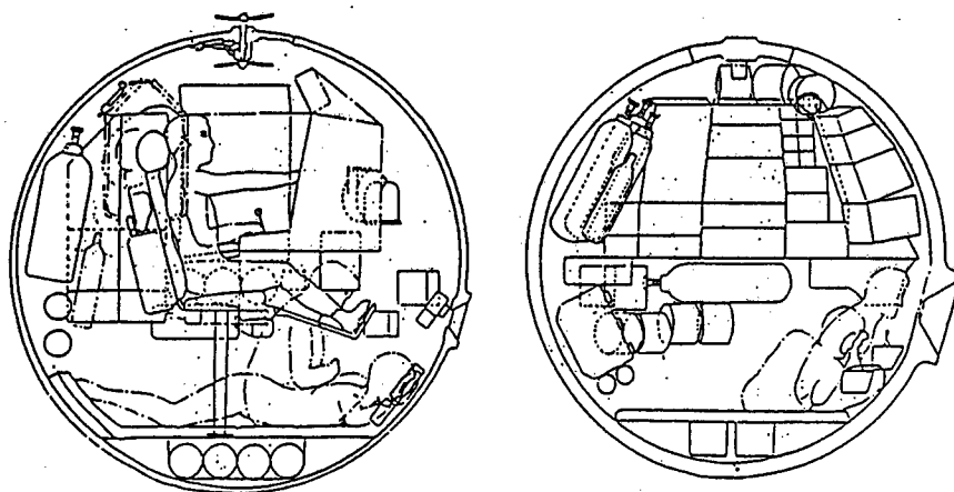
Figure 1. Inside of the Pressure Hull of Shinkai 2000 (left) and Shinkai 6500 (right)
