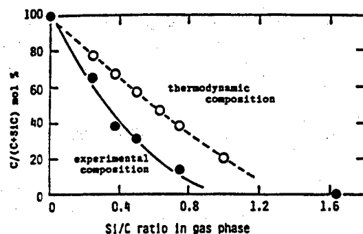
Figure 3. Relationship Between Raw Material Gas Composition and Precipitated Layer Composition
