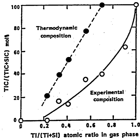
Figure 10. Relationship Between Raw Material Gas Composition and Precipitated Layer Composition
