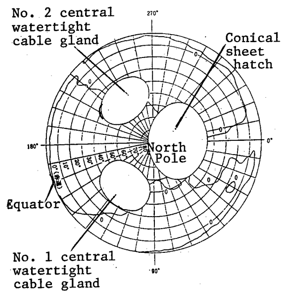
Figure 7. Sphericity Deviation (Radius) Distribution of N-Hemisphere
