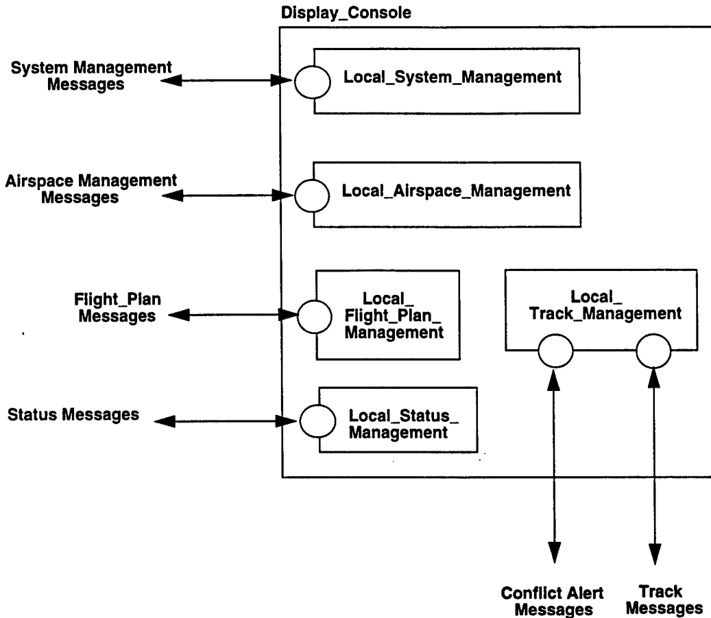
Figure 62: POSIX.21 Design for Display Console
