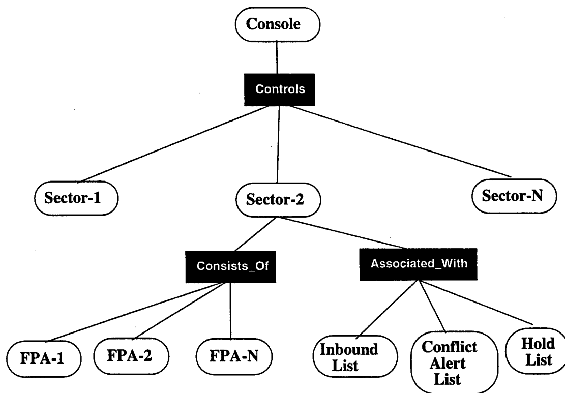
Figure 19: Console-Object Relationships
