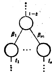
Figure 2. Rule Selection Layer
