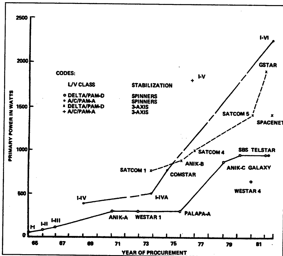
Figure 16. Satellite Power , From Ref. [11]
