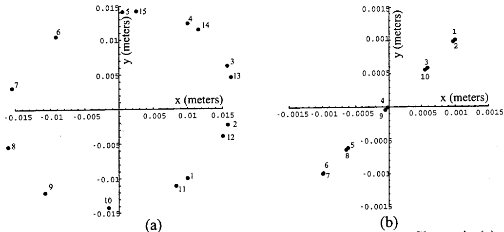
Figure 8.9. Output spot patterns of Herriott time-delay resonator. Shown in (a) are the first 15 outputs spots of a near circular output pattern. Input parameters were \{d = .353, f_x = 3.75, f_y = 3.75, x_o = .01, x' = .01, y_o = .01, y' = -.01\} . In (b), the output has collapsed to a nearly a straight line. Input parameters were \{d = .353, f_x = 3.75, f_y = 3.75, x_o = .001, x' = .0001, y_o = .001, y' = .0001\} .
