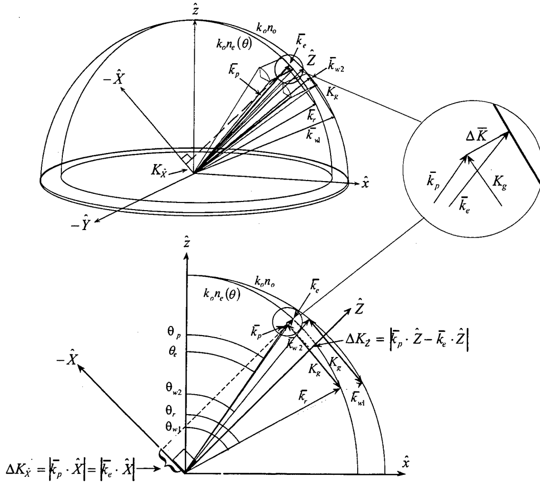
Figure 5.6. Read/write geometry in both 3 and 2D momentum space showing grating vector \bar{K}_g written between \bar{k}_{w1} and \bar{k}_{w2} and read out by \bar{k}_r . Bragg mismatch results in momentum mismatched component \Delta\bar{K} , shown in figure inset.
