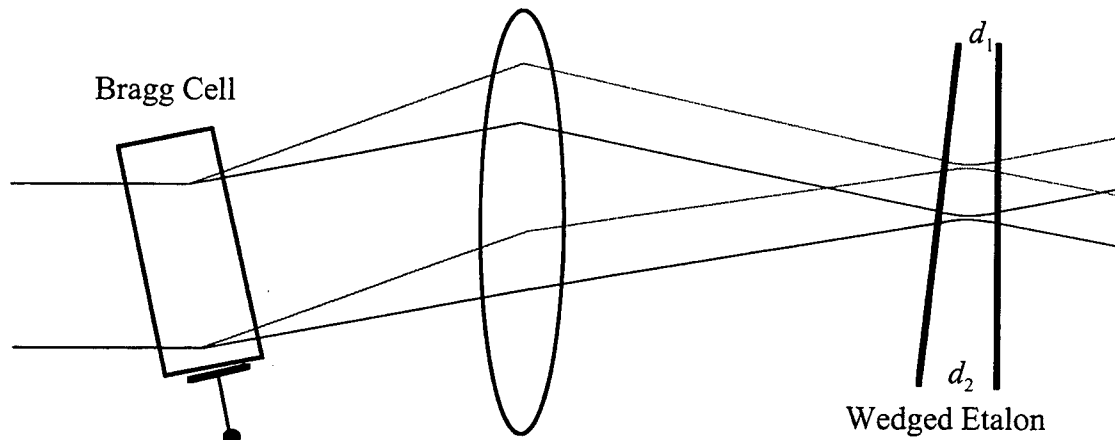
Figure 8.5. Wedged etalon with position dependent frequency bandpass function is placed in the Fourier plane of the Bragg cell.
