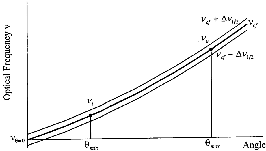
Figure 8.2. Transfer curve of cavity resonant frequency v_{cf} versus angle \theta for tilted Fabry-Perot etalon.
