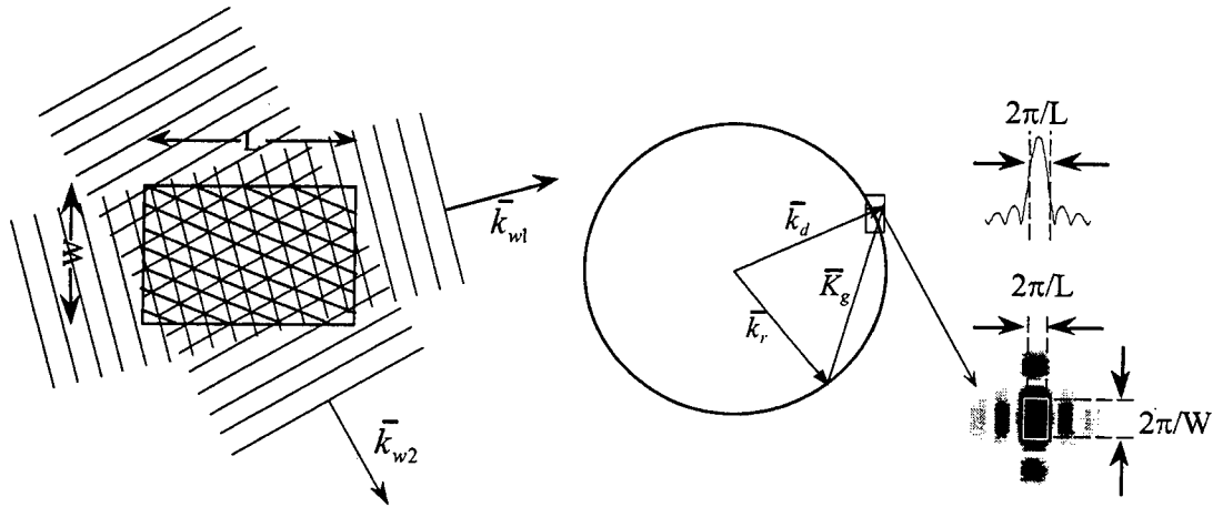
Figure 5.1. Rectangular holographic interaction region of dimensions L \times W creates two-dimensional \text{sinc}^2 in Fourier space. The half-width to the first zero in each dimension of the \text{sinc}^2 function, corresponding to 2\pi/L and 2\pi/W , define the momentum uncertainty box in two dimensions.
