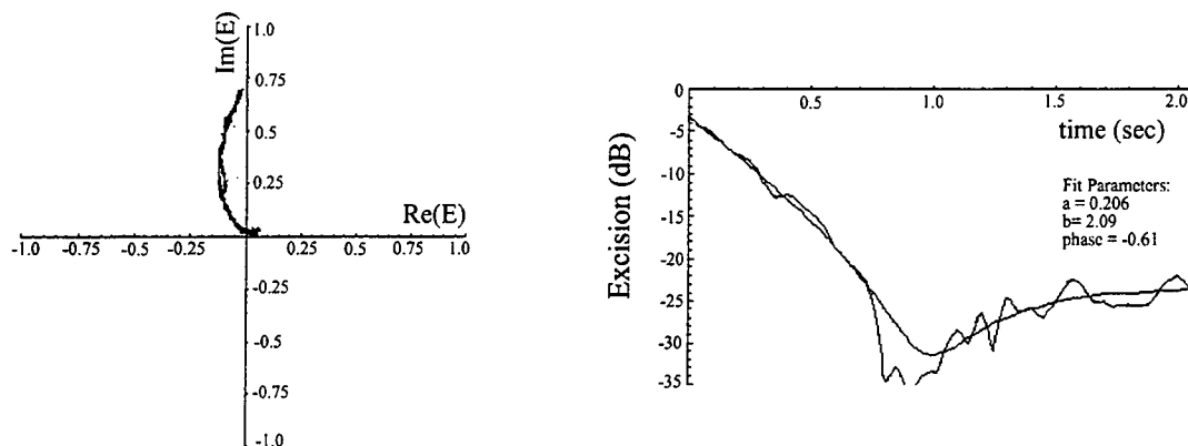
Figure 7.25. (a) Experimental data of excision plotted in complex plane, superimposed over fit of theoretical model, (b) magnitude of excision versus time, also with theoretical fit.
