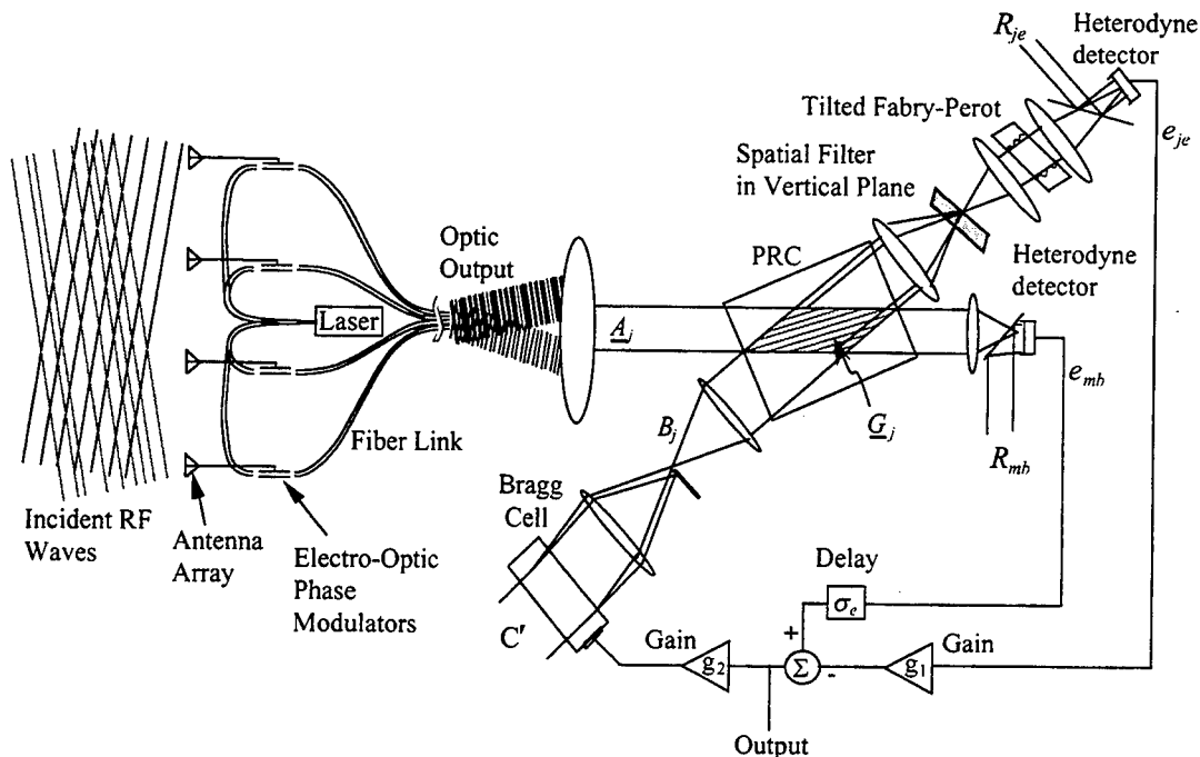
Figure 7.1. Schematic of adaptive jammer-nulling processor.
