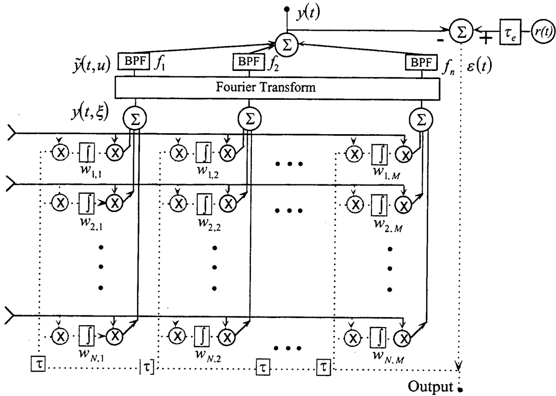
Figure 2.11. Schematic of optically implemented LMS algorithm.
