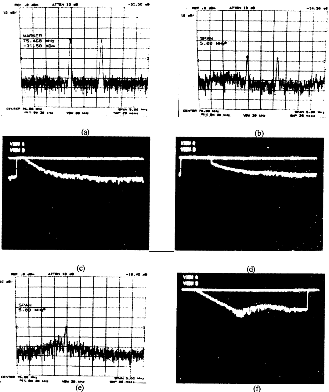
Figure 7.28. Spectrum analyzer trace of two equal strength narrowband jammers at 75.5 and 76.7 MHz: (a) before suppression, and (b) suppressed by 14.3 dB, (.5 MHz/div, 10dB/div). Figures (c) and (d) show the suppression time dynamics (decay rate) of 75.5 and 76.7 MHz jammers respectively (.2 sec/div, 10 dB/div). A single 75.5 MHz jammer is shown in (e) with increased suppression of 4 dB after turning off second jammer, while suppression rate is unaffected as shown in (f). Figures (c), (d), and (f) were obtained by using the spectrum analyzer in zero-span mode.
