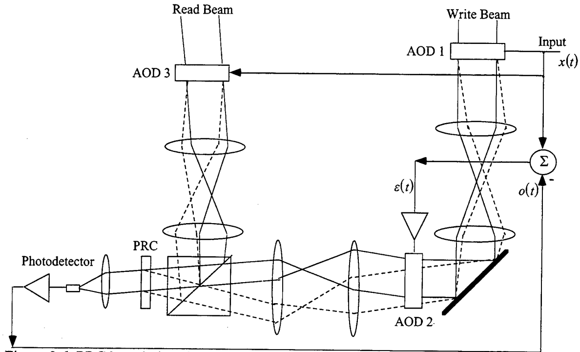
Figure 3.6. PRC based, time-integrating adaptive filter.
