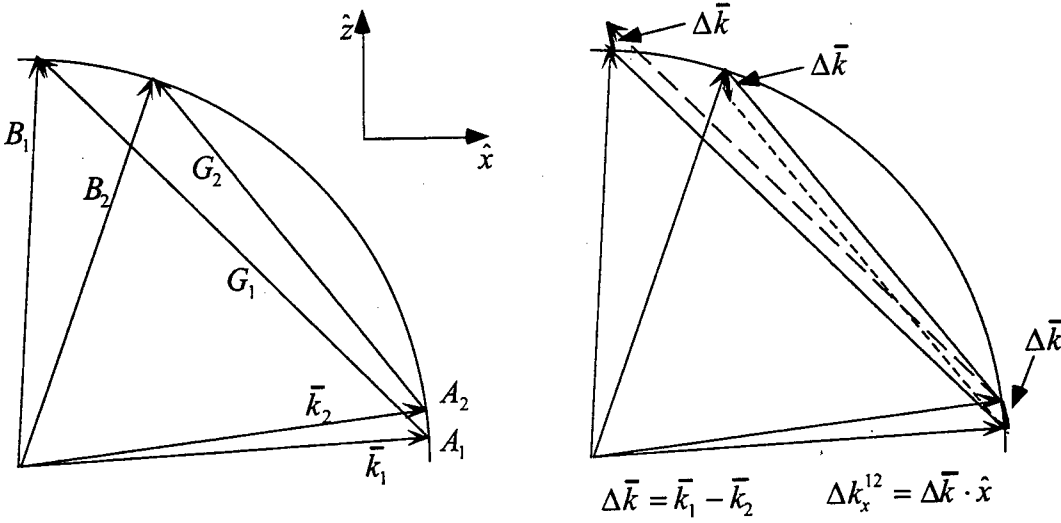
Figure 7.5. Two planewave jammers, A_1 and A_2 , of frequency \omega_1 and \omega_2 respectively, shown in momentum space, write independent gratings G_1 and G_2 . Each jammer can diffract off of the grating written by the other jammer, with momentum mismatch \Delta\bar{k} .
