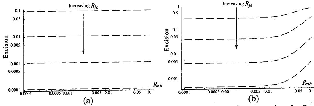
Figure 7.17. Excision versus main-beam heterodyne reference signal R_{MB} , parameterized in jammer estimate heterodyne reference signal R_{JE} , where R_{JE} = 10^{-4}, 10^{-3}, 10^{-2}, 10^{-1} . There is no desired signal in (a), and there is a desired signal of amplitude D = 10^{-3} in (b). The simulation parameters were: A = 0.1 , U = 10^{-7} , with units of volts/meter, and r = 1 . N_{JE} = N_{MB} = 10^{-7} in units of amps, g_2C = 4 \times 10^4 , with units of volts/meter, and f = 0 , which is unitless.
