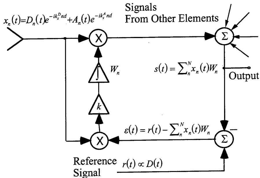
Figure 7.12. Single LMS adaptive loop as discussed in Chapter 2.
