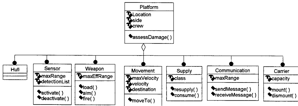
Figure 32. Platform Class Aggregation
