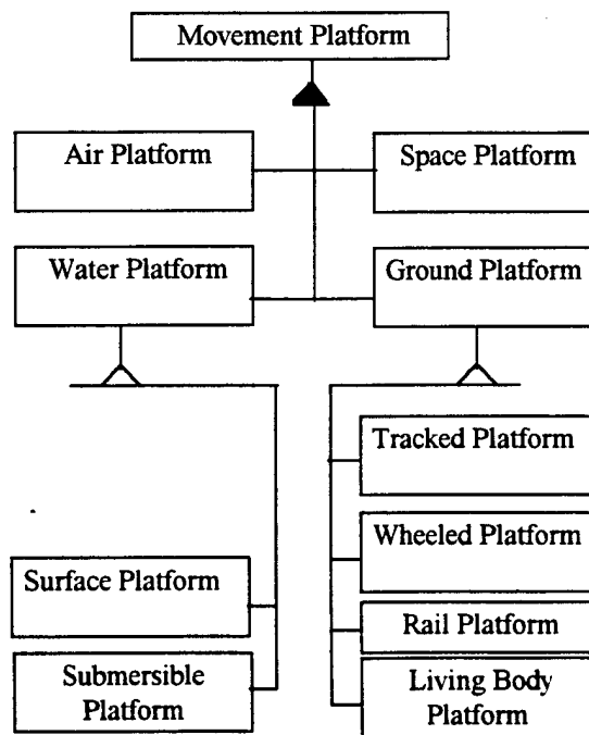
Figure 17. WARSIM 2000 Movement Platform Class [Hopkins, 1997]
