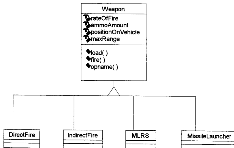
Figure 12. ModSAF Weapon Class
