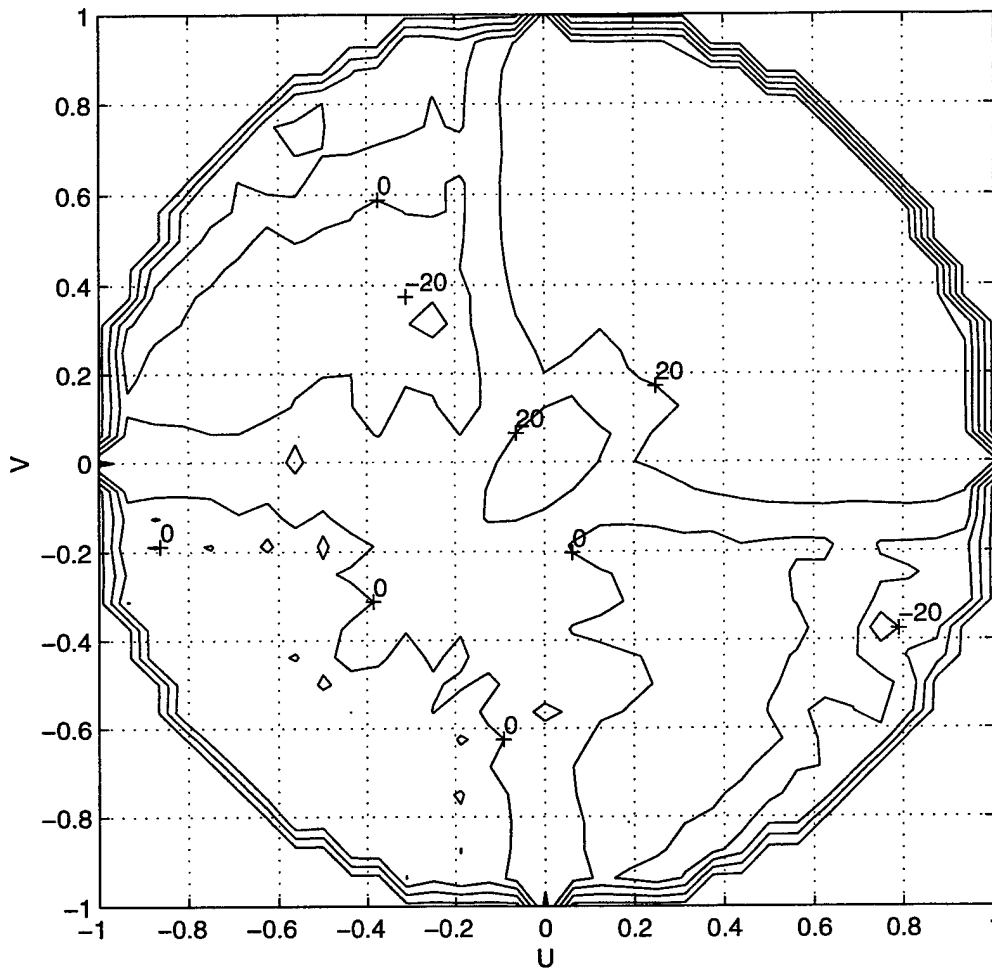
Figure 22. Three triangular plate geometry at frequency of 120 MHz and 25 edges/side using Patch .
