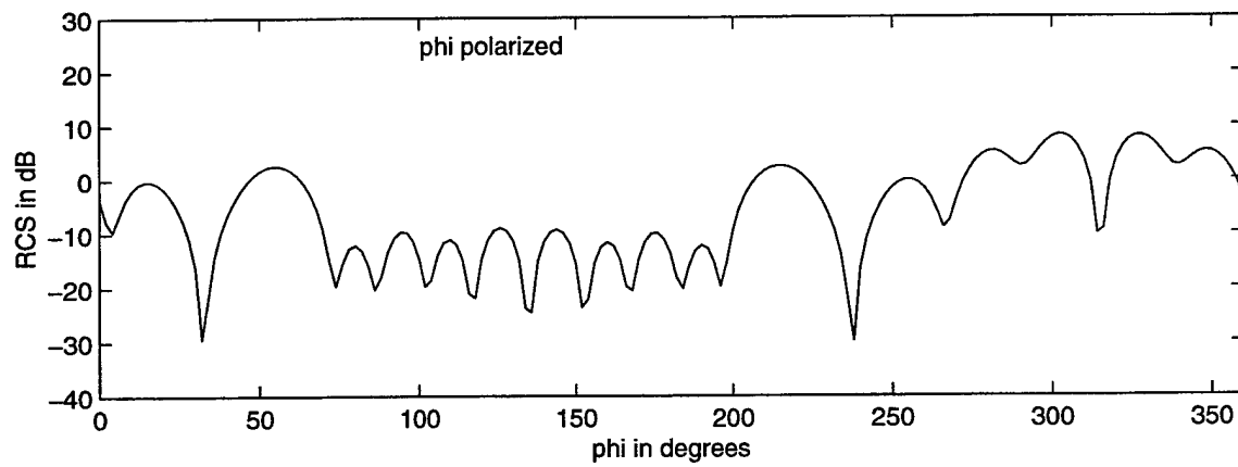
Figure 17. RCS of three triangular plate geometry at frequency of 60 MHz and 20 edges/side for \theta = 60^\circ using Patch.
