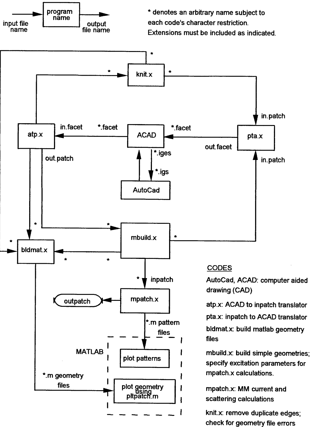
Figure 6. Relationships between computer codes.
