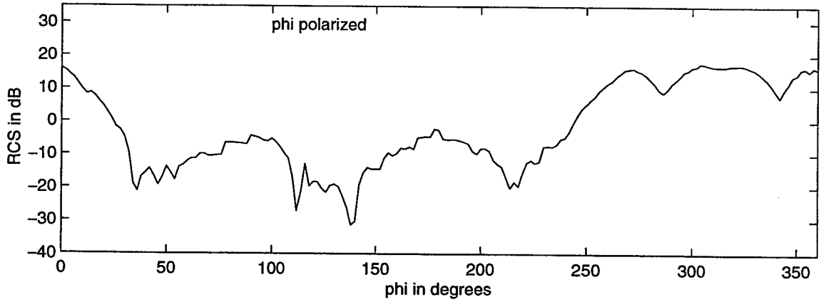
Figure 18. RCS of three triangular plate geometry at frequency of 60 MHz and 20 edges/side for \theta = 60^\circ using Xpatch.
