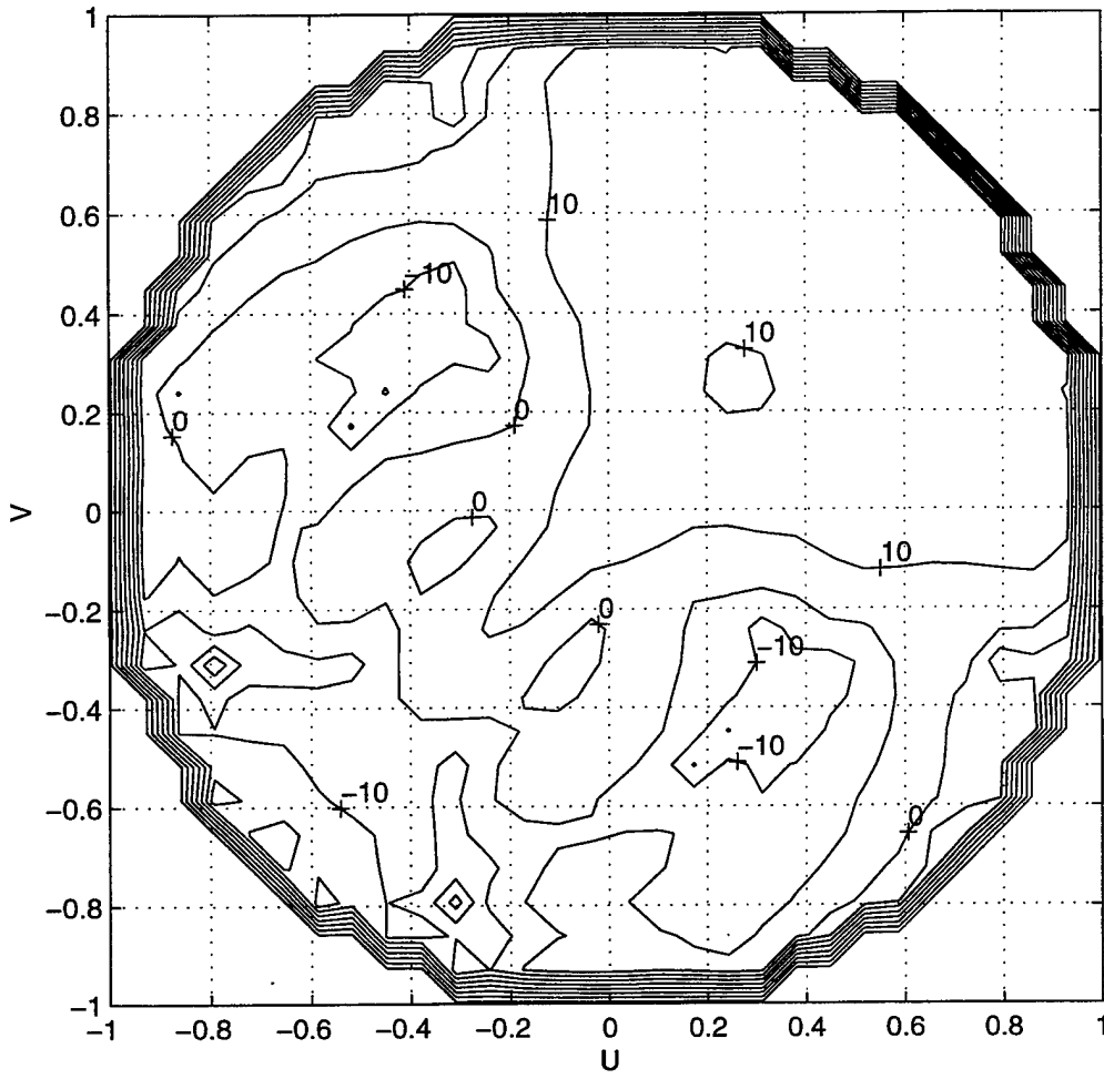
Figure 11. RCS of three triangular plate geometry at frequency of 60 MHz and 20 edges/side using Patch .
