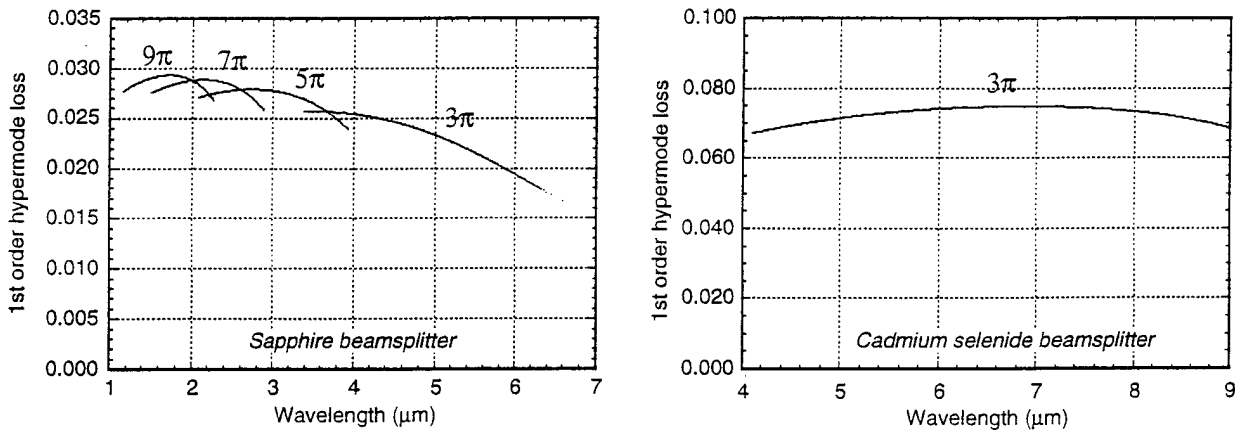
Figure 3. Round-trip, sideband mode losses for the 9\pi , 7\pi , 5\pi , and 3\pi phase retardations in sapphire, and for the 3\pi phase retardation in CdSe, across their respective tuning ranges for beamsplitter rotation angles of \pm 22^\circ .
