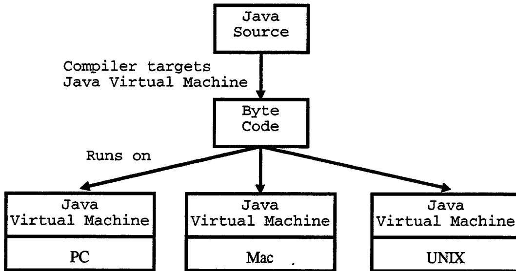
Figure 10. Compilation and Execution for Java. After (PRI, 1997)
