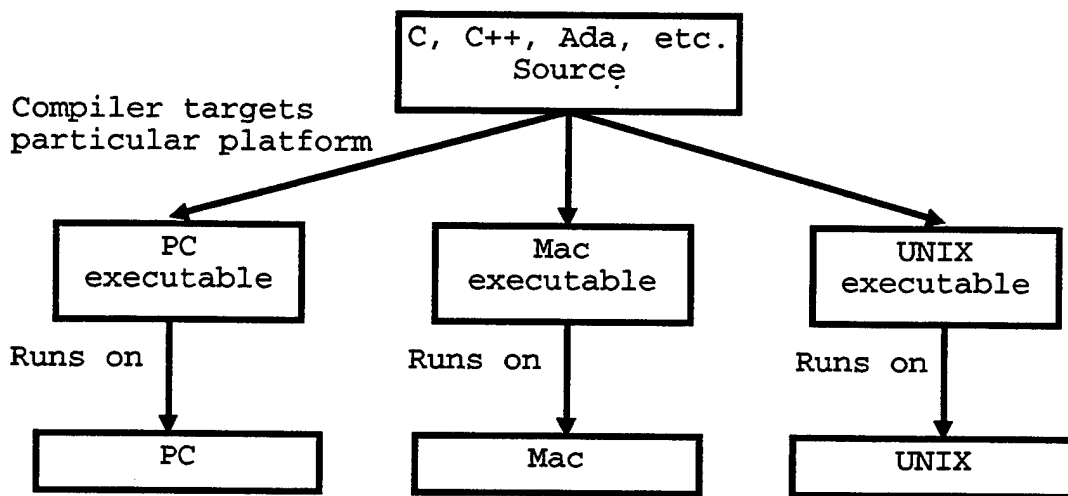
Figure 9. Compilation and Execution for Conventional Programming Languages.
