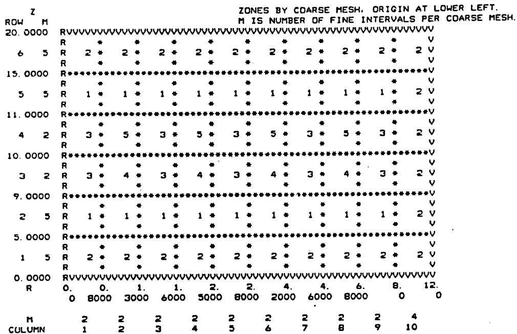
Figure 7 TWODANT Core Map
