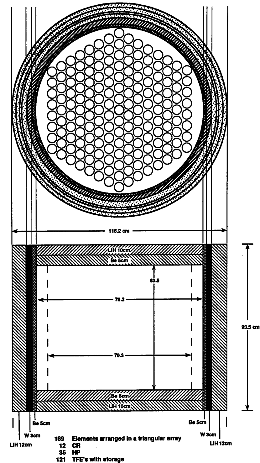
Figure 2.12. Schematic Showing Relative Zones of OTS Reactor Concept
