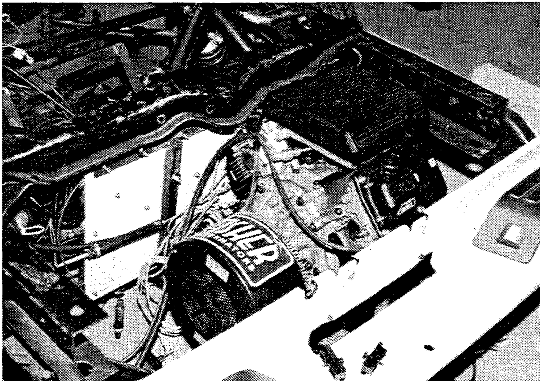
FIGURE 31. SwRI APU INSTALLED IN S-10 VEHICLE (REAR MOUNT)
