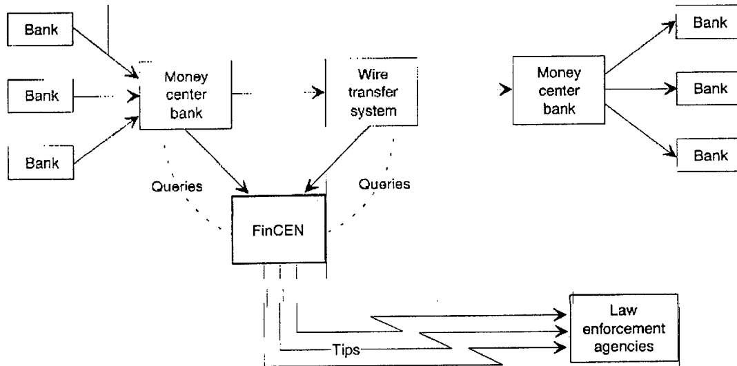
Figure 7-4: Targeted Access
