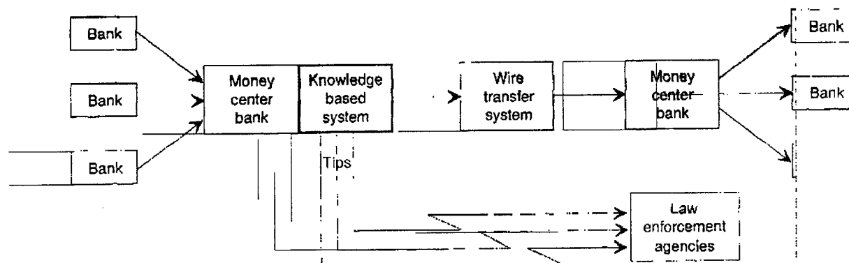
Figure 7-2: Automated Informant
