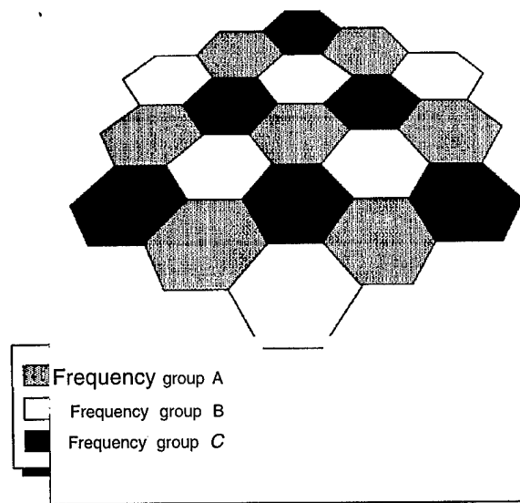
FIGURE 3-6: Frequency Reuse Concept
