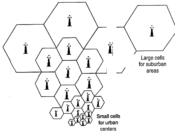
FIGURE 3-7: Cell-Splitting
