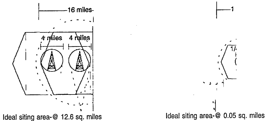
FIGURE 8-1: Theoretical Antenna Siting Constraints
