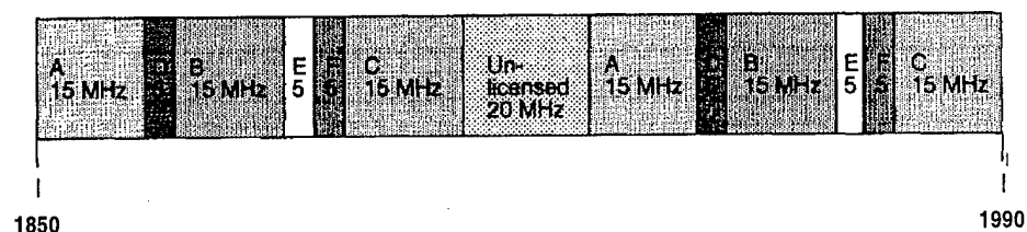
FIGURE 3-3: PCS Spectru
