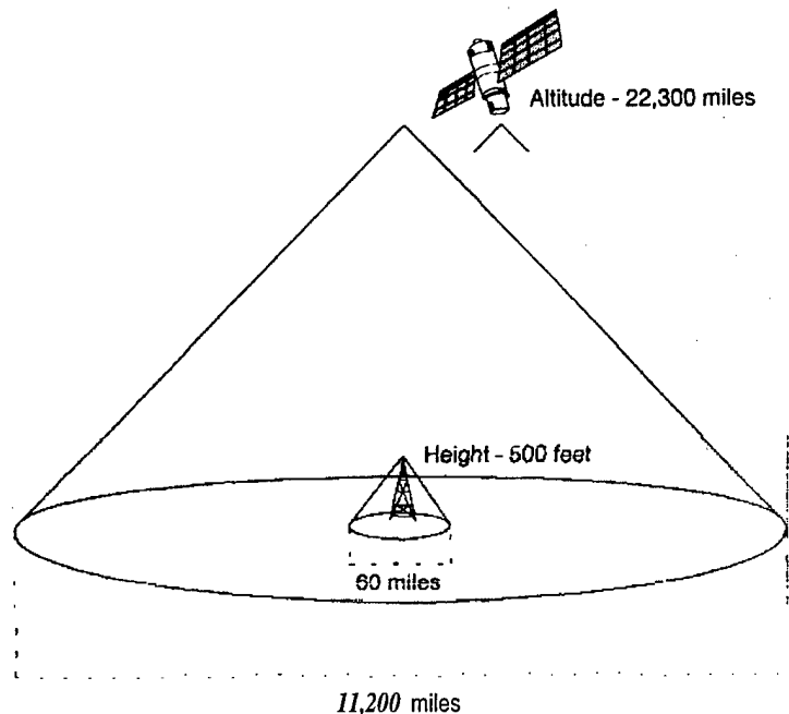
FIGURE A-8: Terrestrial and Satellite Transmission Ranges
