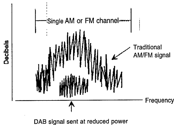
FIGURE 5-2: In-Band, On-Channel Digital Audio Broadcasting Systems
