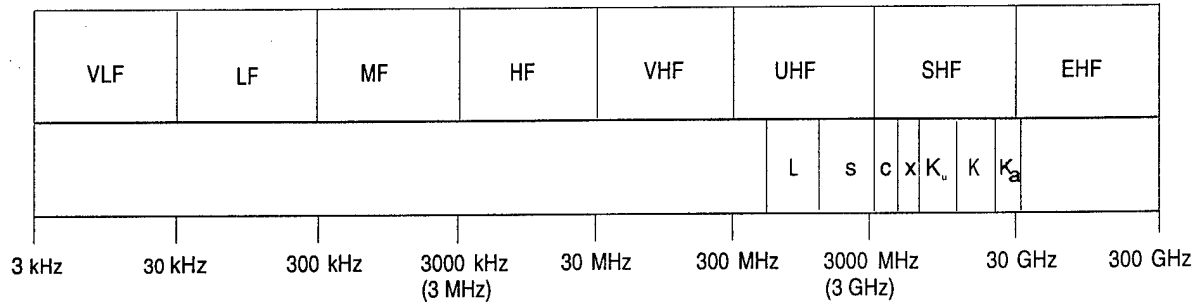
FIGURE A-7: Frequency Band Designations
