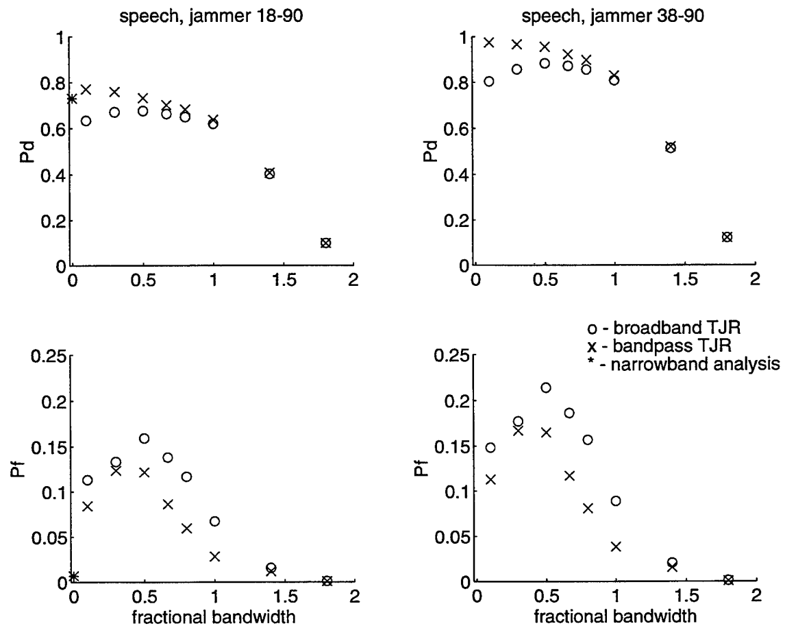
Figure 5-12: Simulation results showing rates of detection and false alarms, as a function of bandwidth, for speech and babble received by two microphones in an anechoic environment. The points labeled with 'x' indicate the performance referenced to the bandpass TJR, while the points labeled with 'o' indicate the performance referenced to the broadband TJR. The points labeled with '*' correspond to the values determined by the narrowband analysis of Sec. 5.2.3.
