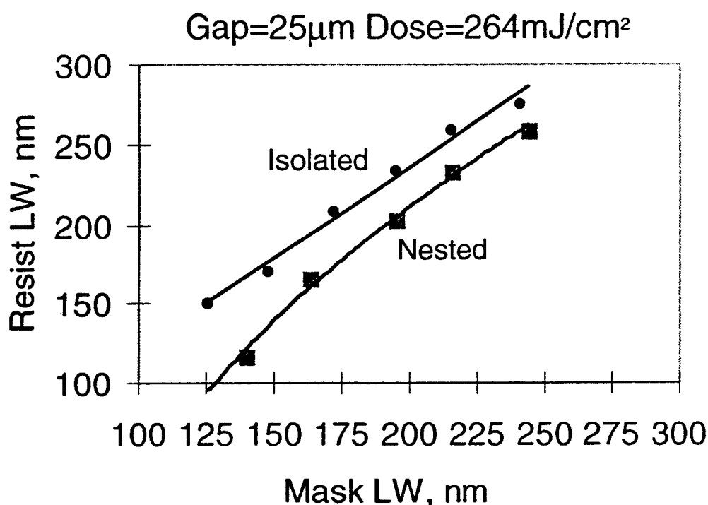
Figure 27. UV-4 Linearity
