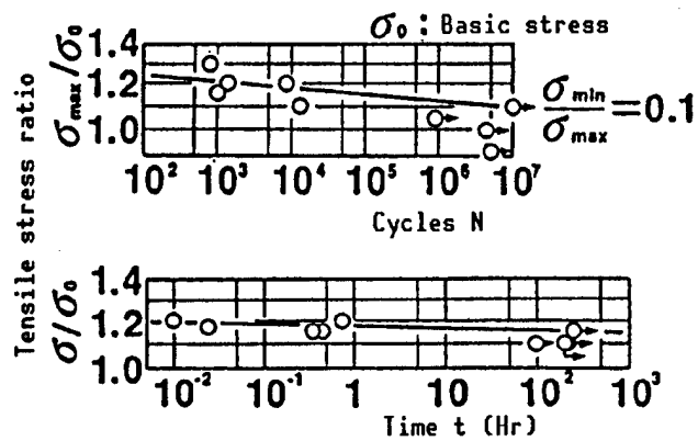
Figure 5.1.3.9 Fatigue Strength Diagram for \text{Si}_3\text{N}_4
