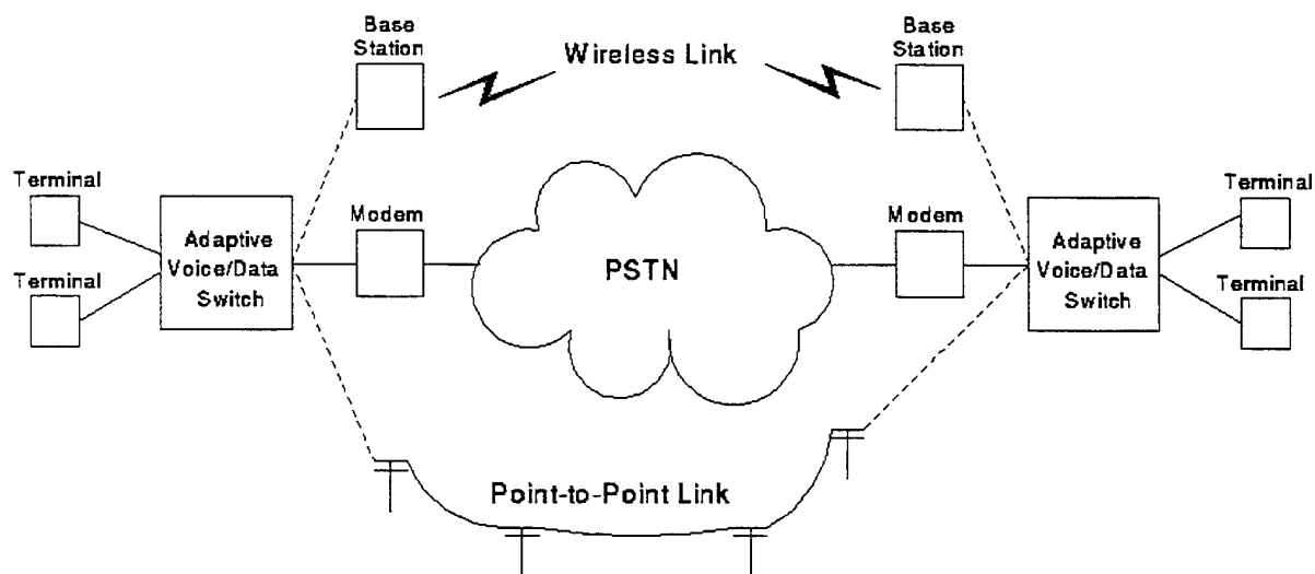
Figure 11.13: AVDnet environment
