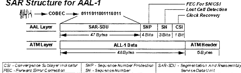
Figure 3.9: AAL 1
