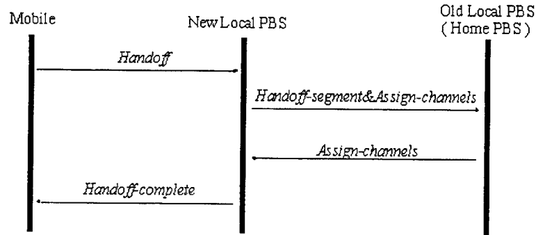
Figure 11.8: Handover messages
