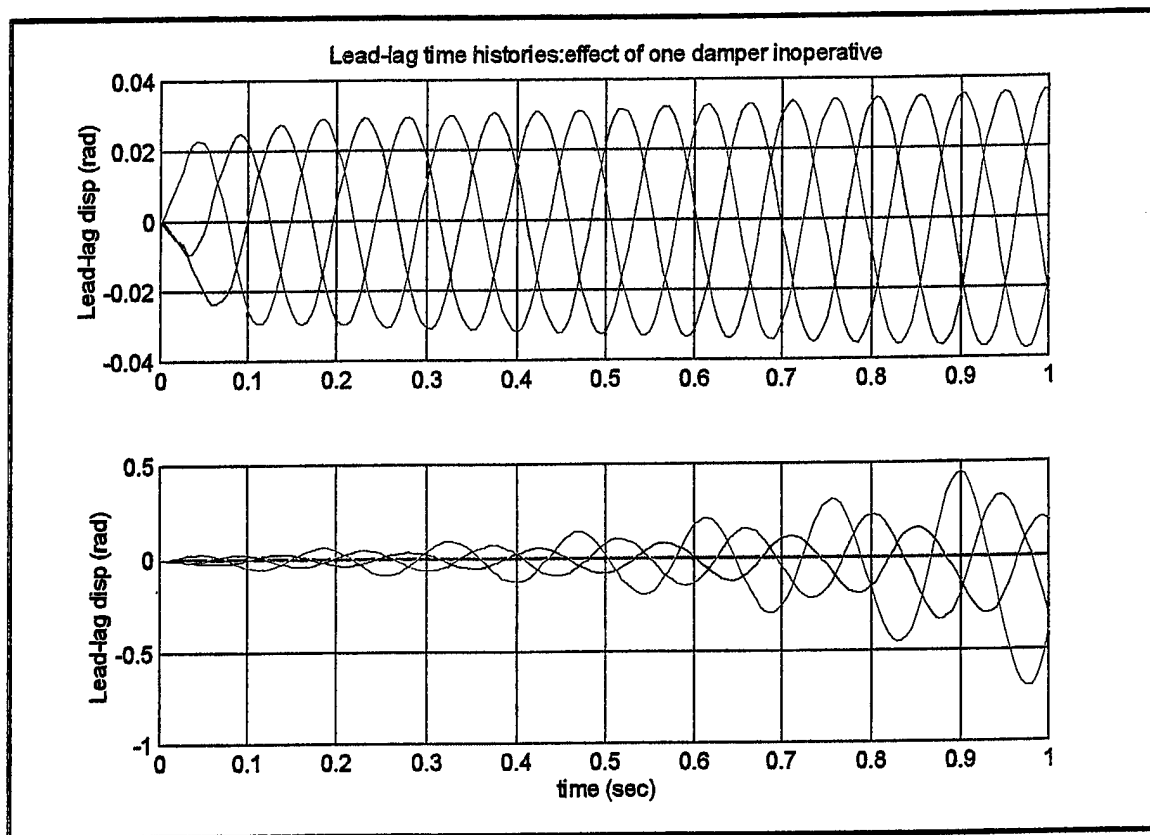
Figure 6.9 One Lead-Lag Damper Inoperative
