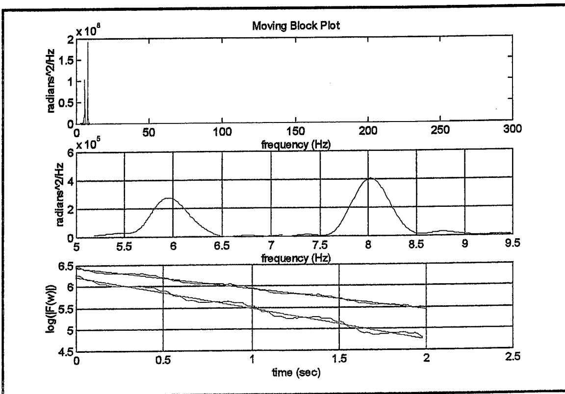
Figure 8.2 Result of Moving Block on Test Signal
