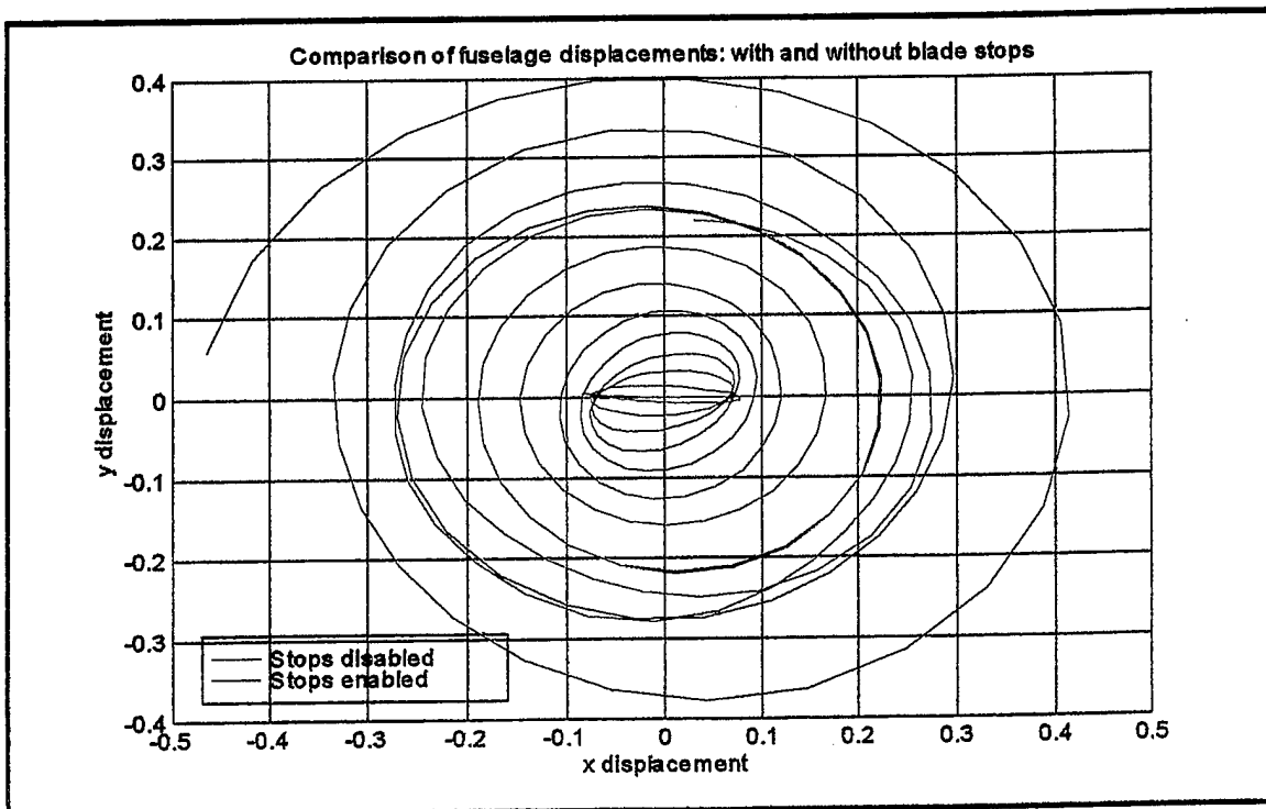
Figure 6.12 Fuselage Displacements with and without Simulated Lead-lag Stops
