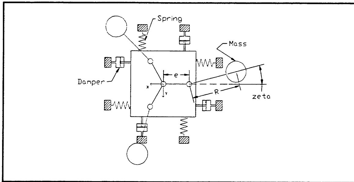
Figure 3. 1 Schematic of Simplified Rotor-Fuselage System
