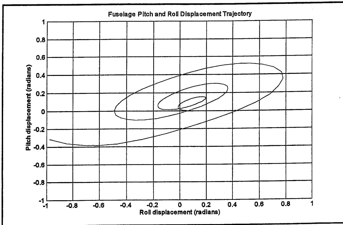
Figure 6.18 Fuselage Displacement Trajectory with Ground Resonance Excited
