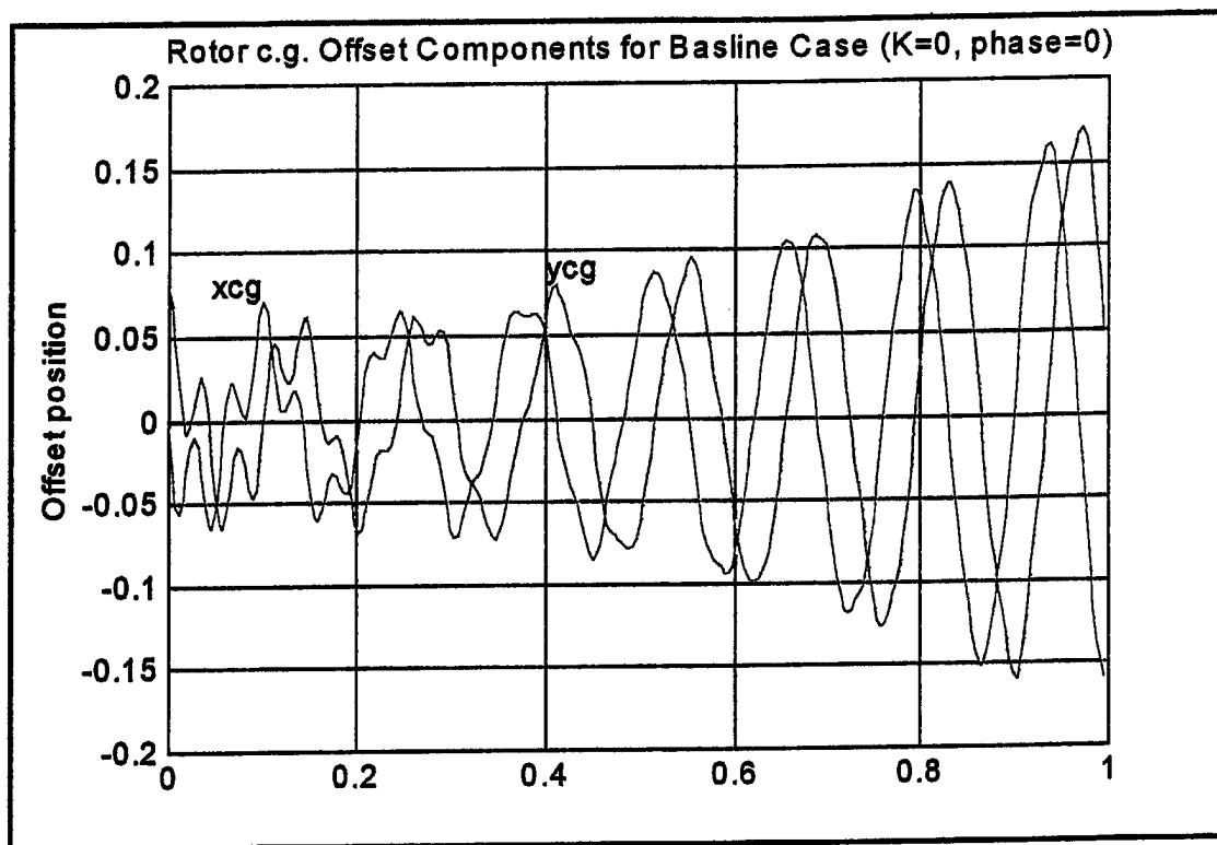
Figure 9.1 Rotor c.g. Offset For Baseline Case ( K=0 , \phi=0 )
