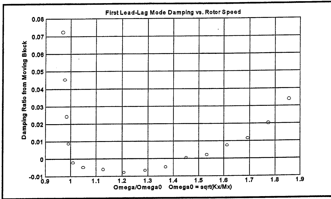
Figure 8.3 Effect of Varying Rotor Speed on First Lead-lag Mode Damping
