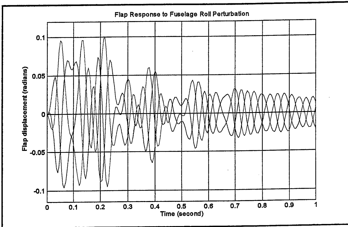
Figure 6.14 Flap Response to Fuselage Roll Perturbation
