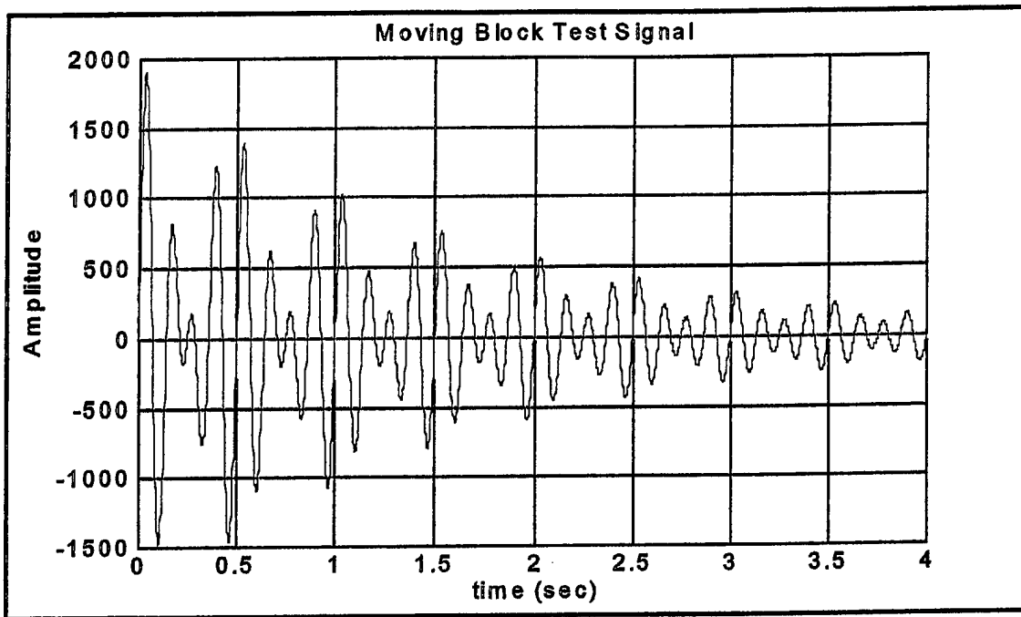
Figure 8.1 Moving Block Test Signal
