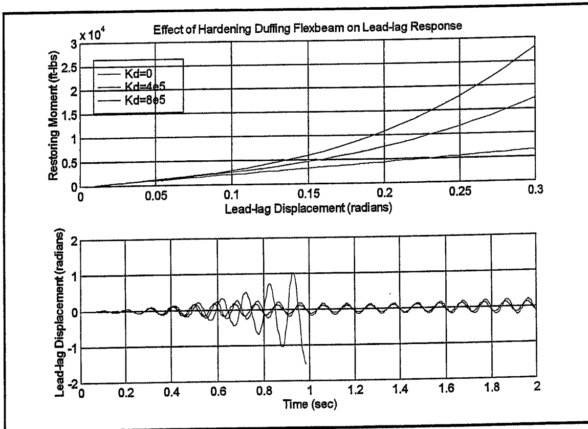
Figure 6.13 Effect of Hardening Duffing Flexbeam on Lead-lag Response
