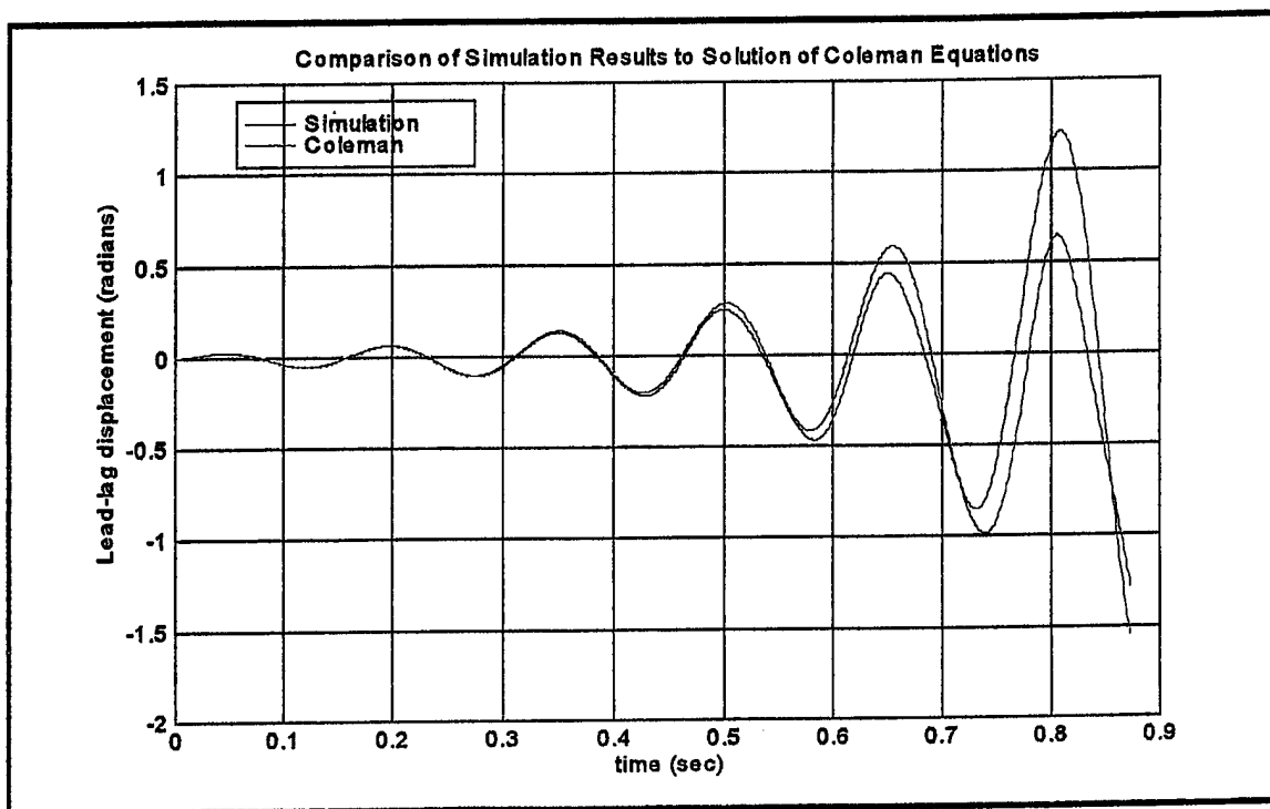
Figure 6.8 Comparison of Simulation Model to Coleman's Model
