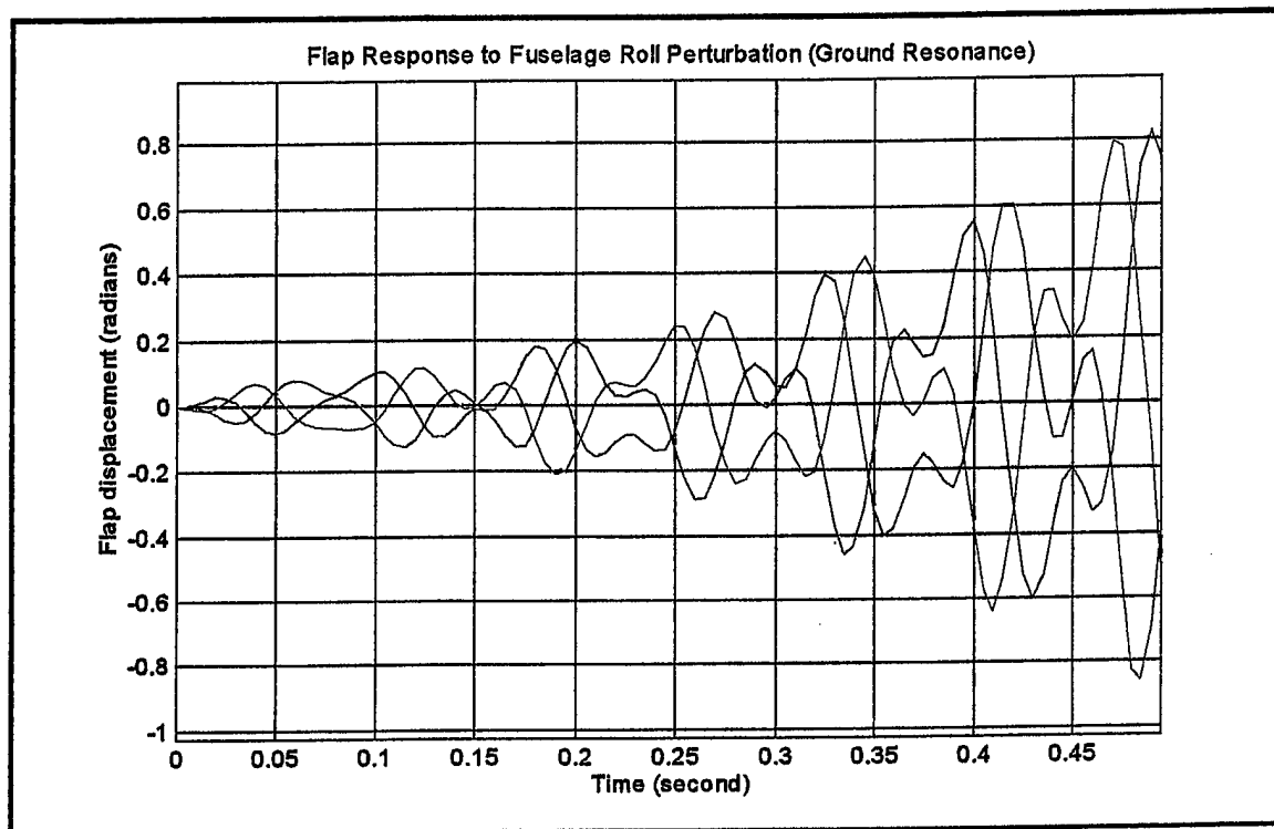
Figure 6.16 Flap Response with Ground Resonance Excited
