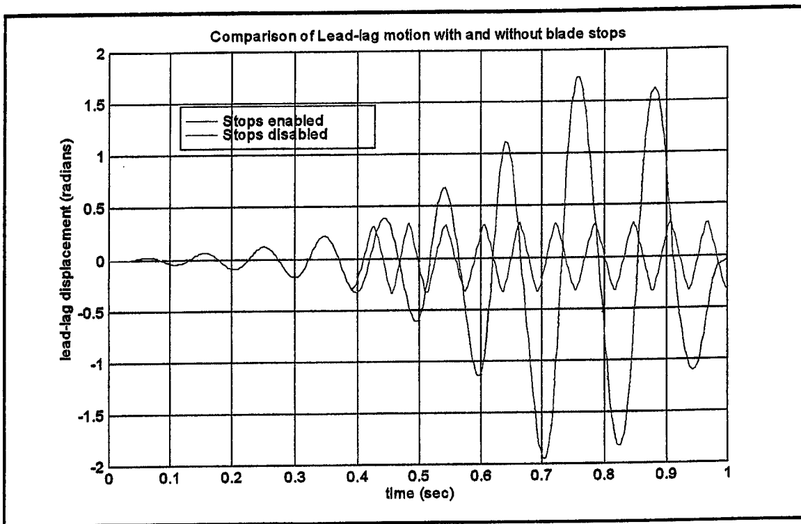
Figure 6.11 Effect of Lead-Lag Stops
