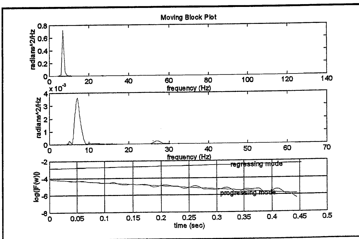
Figure 9.2 Moving Block Results for Baseline Simulation ( K=0 , \phi=0 )
