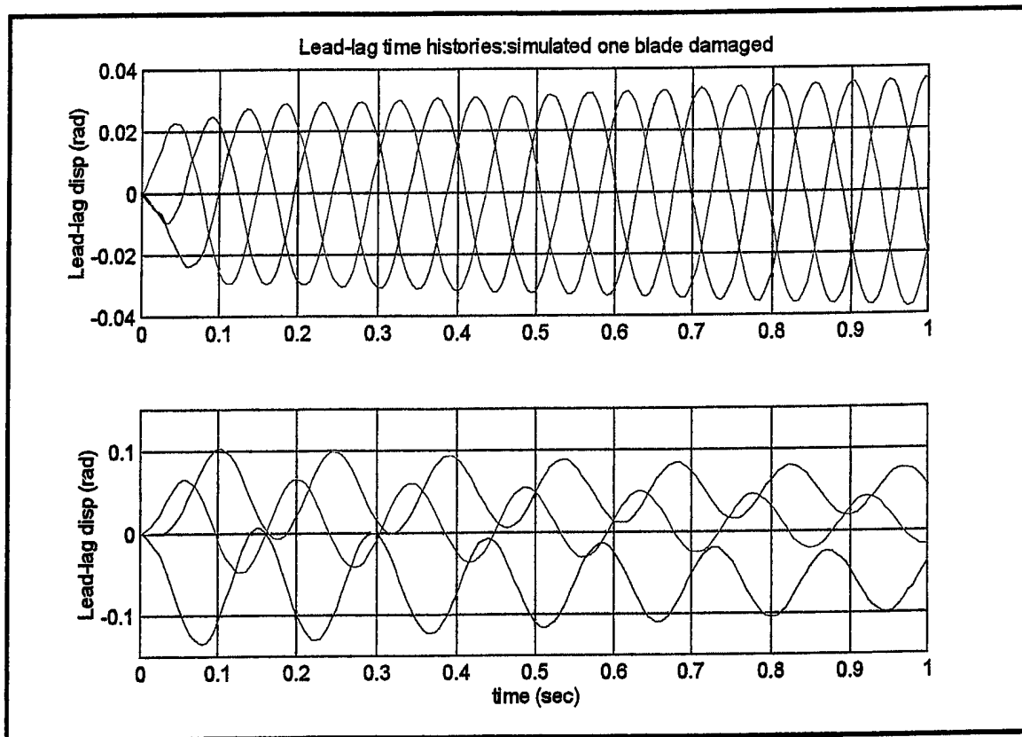
Figure 6.10 Simulated One Rotor Blade Damaged
