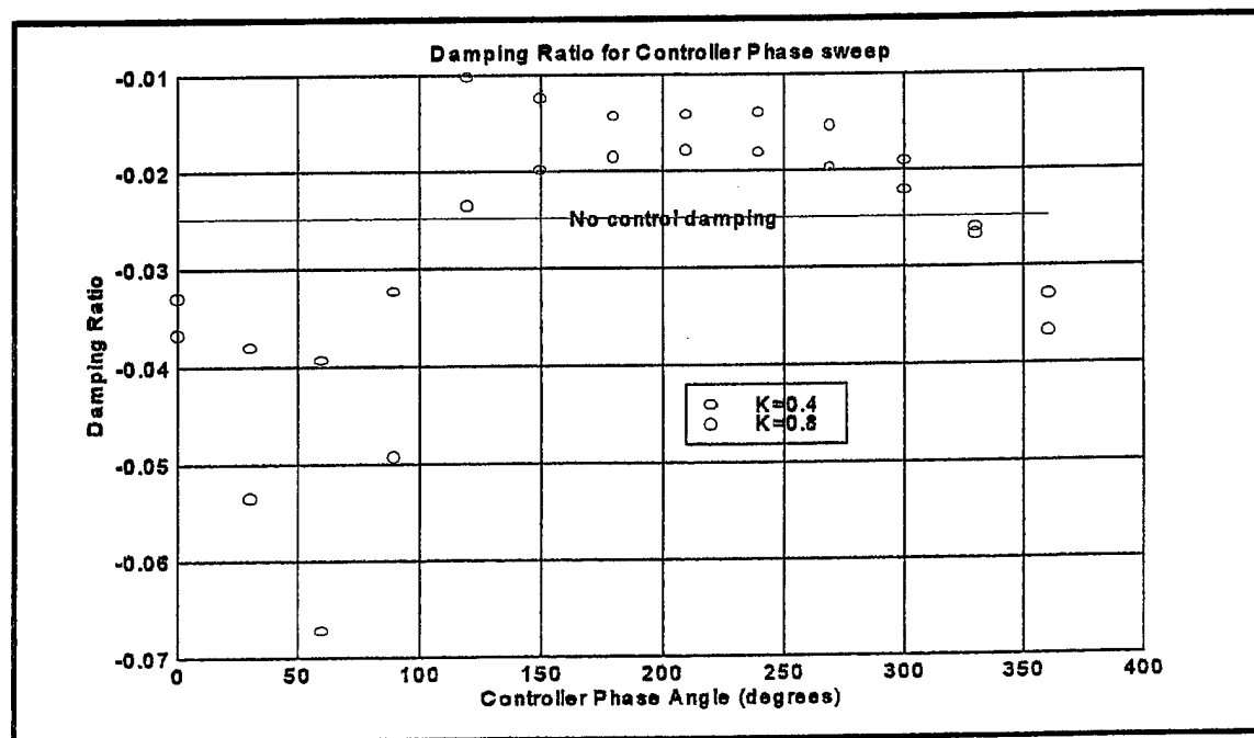
Figure 9.3 Damping Ratio For Controller Phase Sweep ( K=0.4 and K=0.8 )
