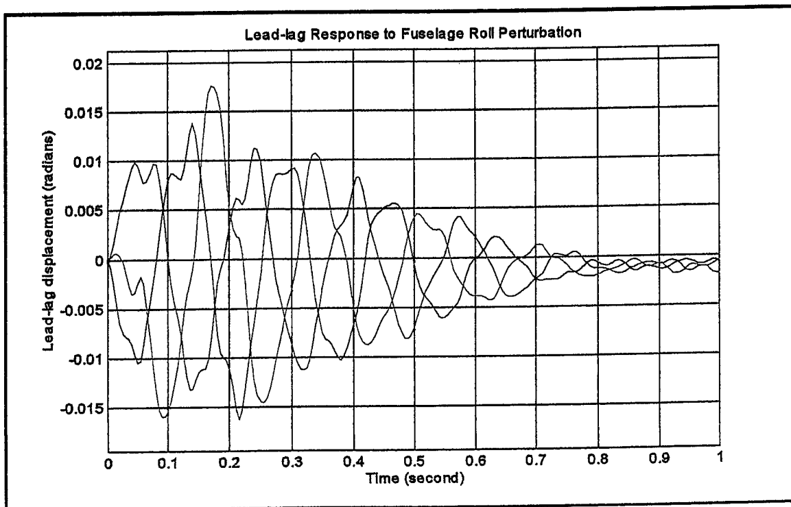
Figure 6.15 Lead-lag Response to Fuselage Roll Perturbation
