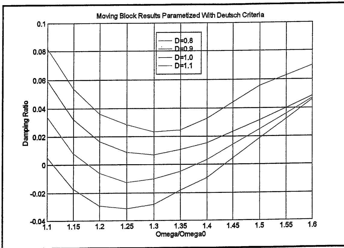
Figure 8.4 Moving Block Results Parametized by Deutsch Number
