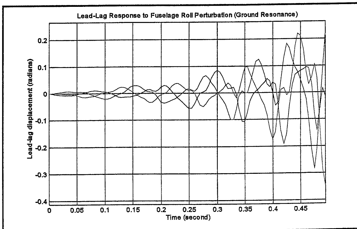
Figure 6.17 Lead-lag Response with Ground Resonance Excited
