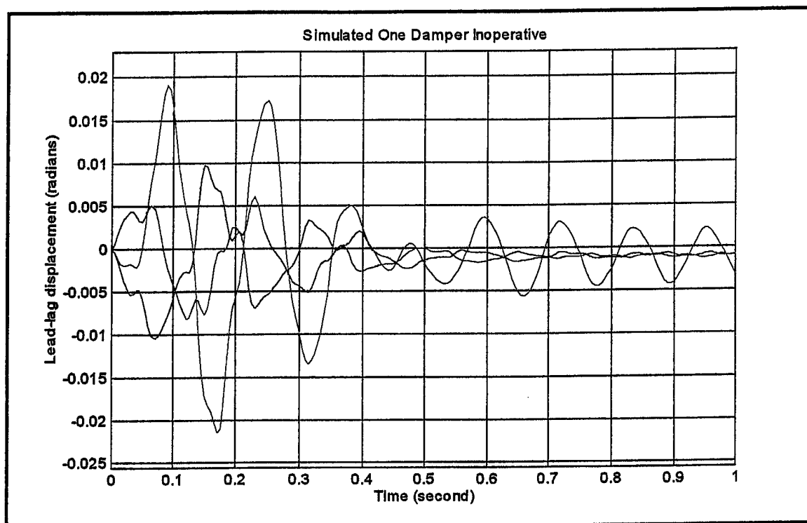
Figure 6.19 Lead-lag Response with One Damper Inoperative
