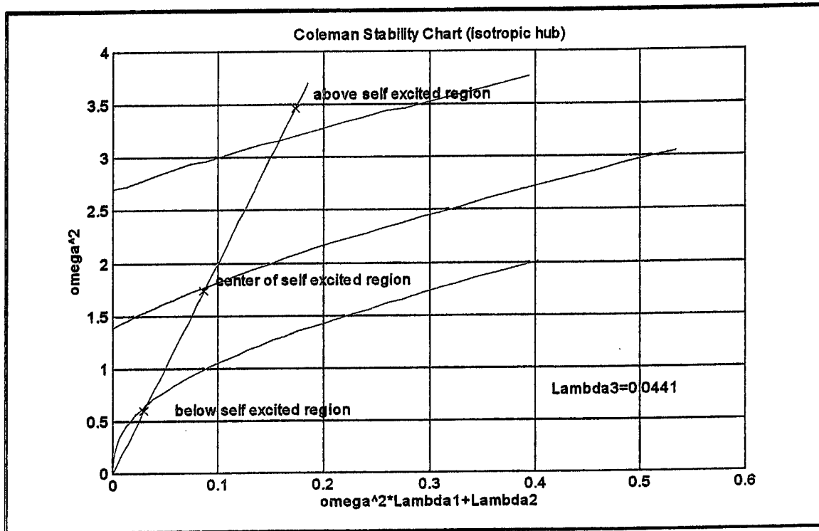
Figure 6.7 Coleman Stability Plot for Basic Case
