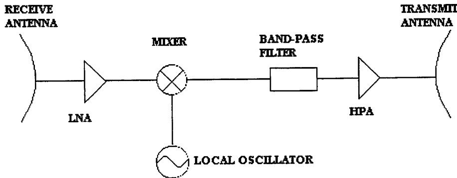
Figure 1.8: Simplified Bent-Pipe Satellite Transponder
