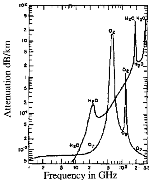
Figure 3.1: Attenuation for atmospheric gases for 15 degrees C and 7.5 g/m 3 humidity [From Ref. 5]
