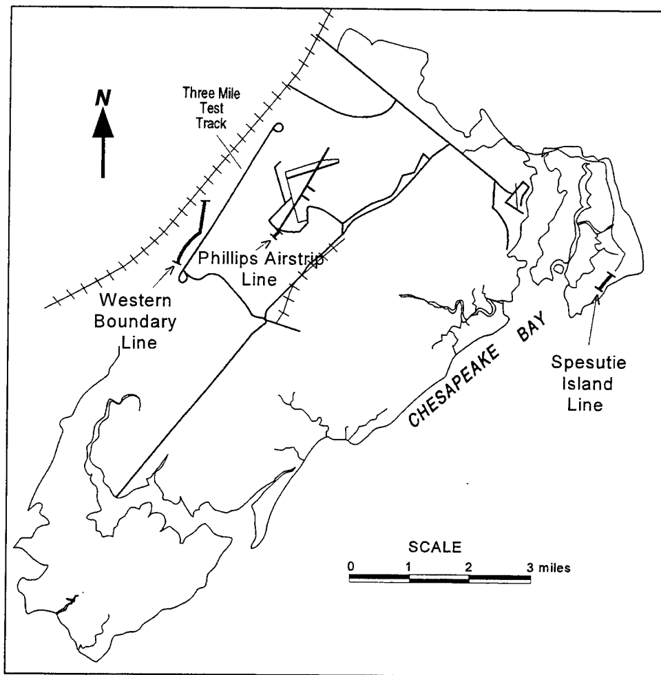
Figure 26. Location of seismic profile lines on APG-AA
