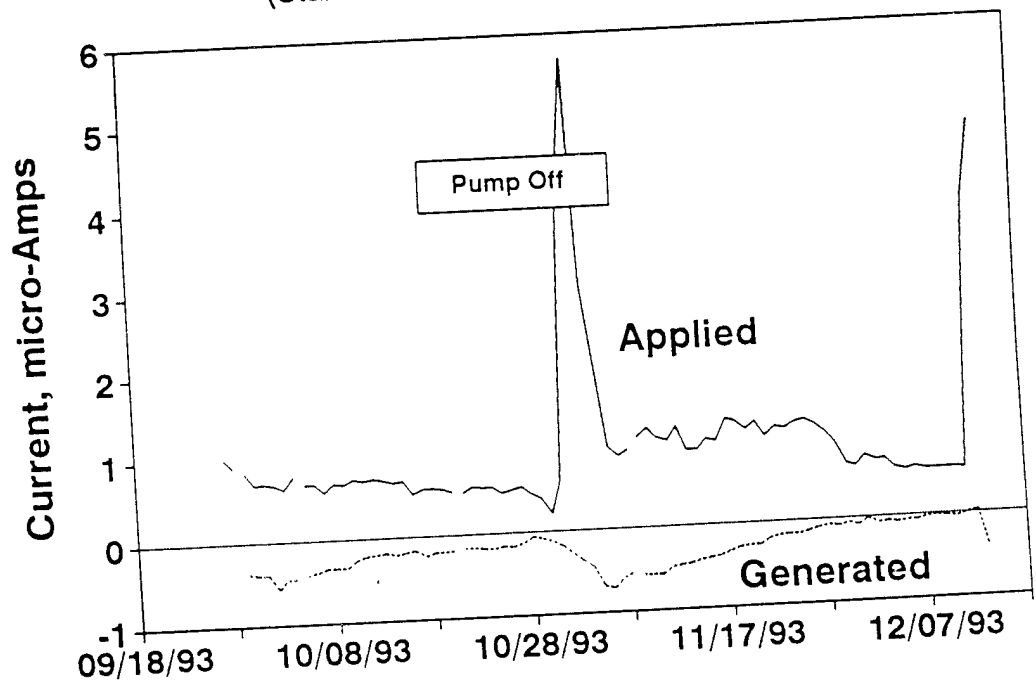
Figure 4. BlOGEORGE Probes Results from NSWC (Titanium, 200mV, Test #1)
