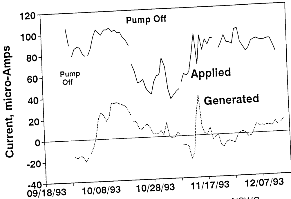
Figure 3. BlOGEORGE Probe Results from NSWC (Stainless Steel, 200 mV, Test #1)
