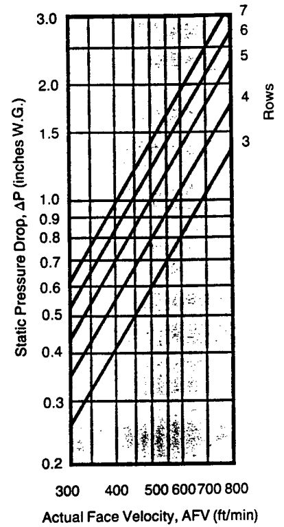
FIGURE 10 — TRU-125 PRESSURE DROP
