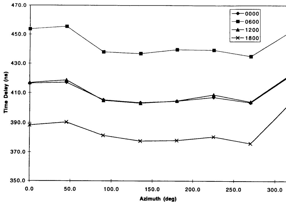
Fig. 25 — D.C., August (HIRAS surface data—0° elevation angle)
