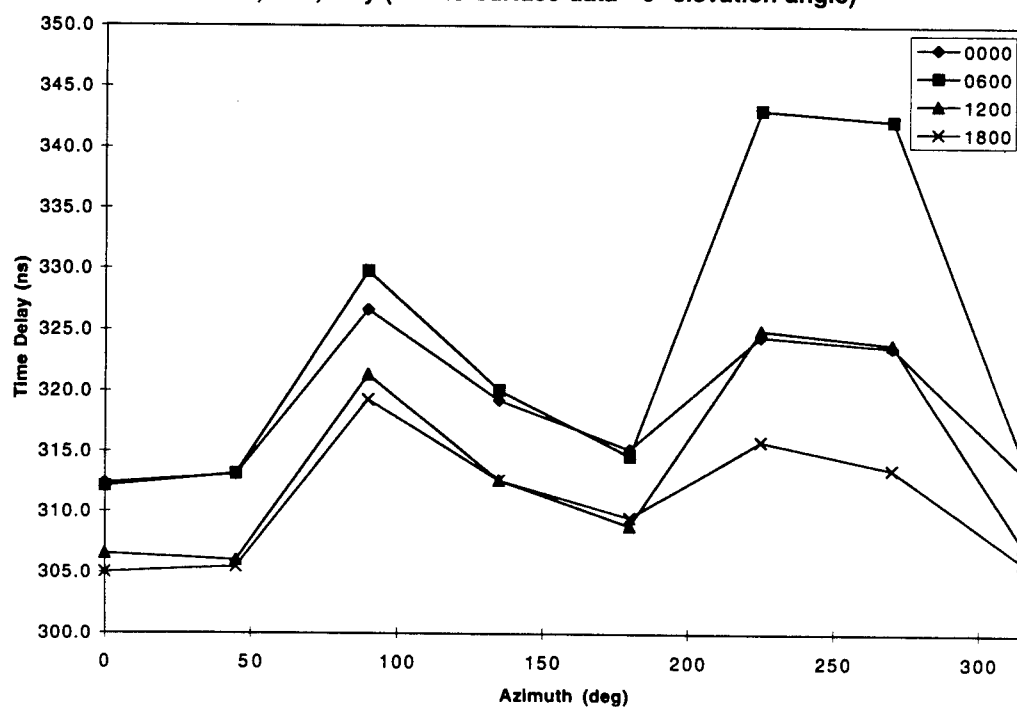
Tehran, Iran, May (HIRAS surface data—0° elevation angle)
