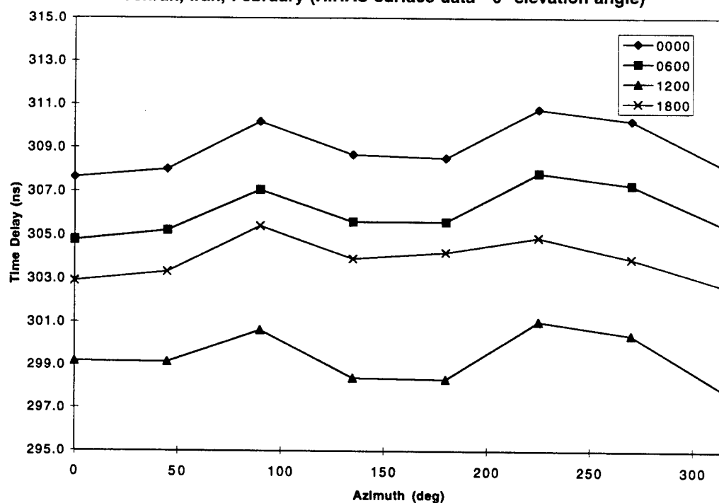
Tehran, Iran, February (HIRAS surface data—0° elevation angle)
