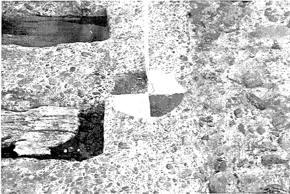
Figure 9. Typical target established on dolosse at Humboldt Bay
