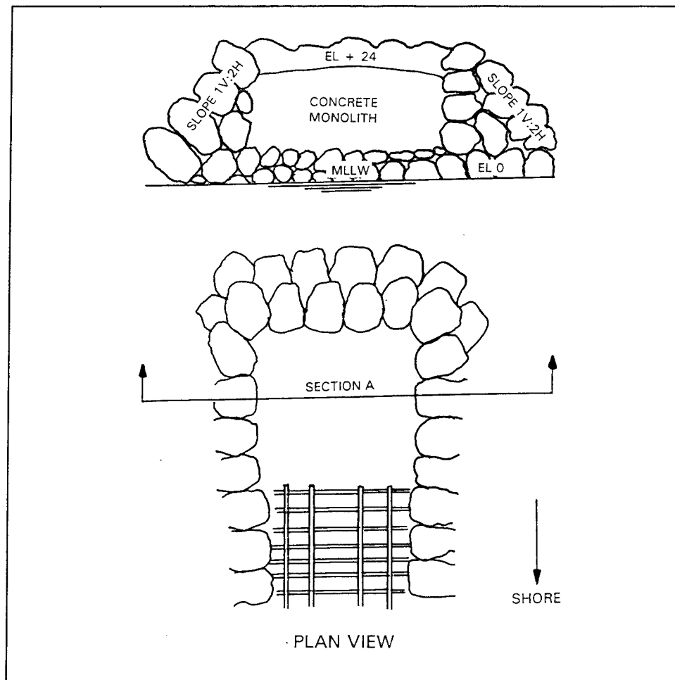
Figure 2. Concrete monolith structure constructed on south jetty in 1911
