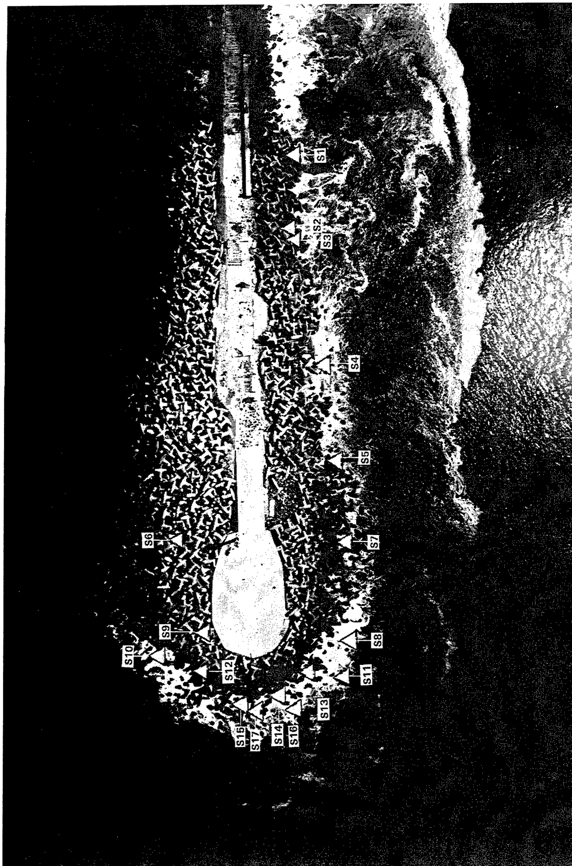
Figure 22. Approximate locations of broken/cracked dolos armor units on the south jetty
