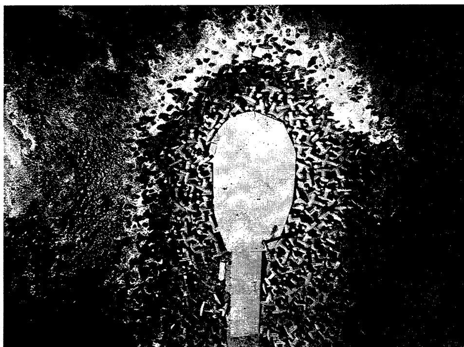
Figure 14. Stereo pair photographs for a portion of the south jetty
