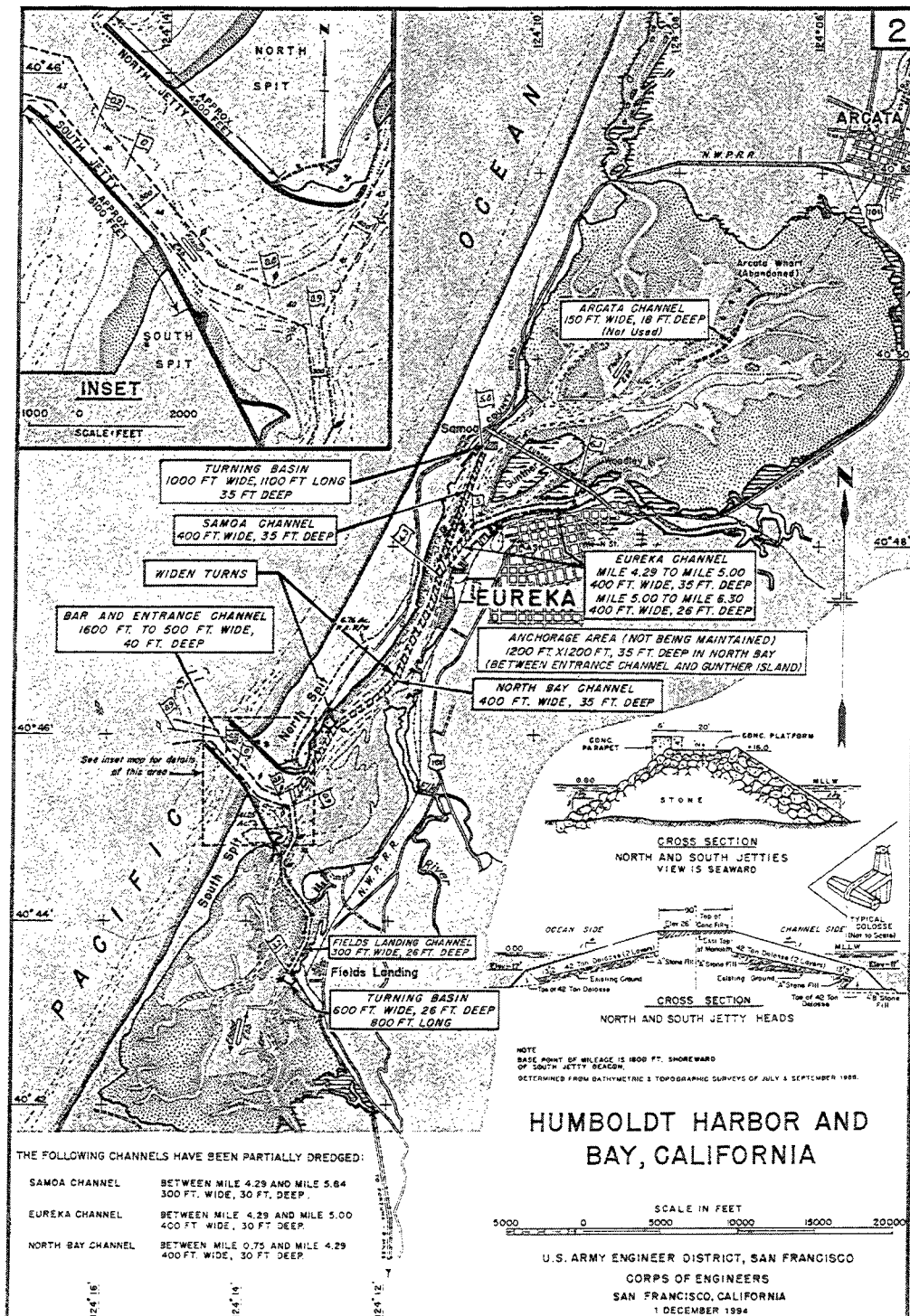
Figure 6. Current project as of December 1994
