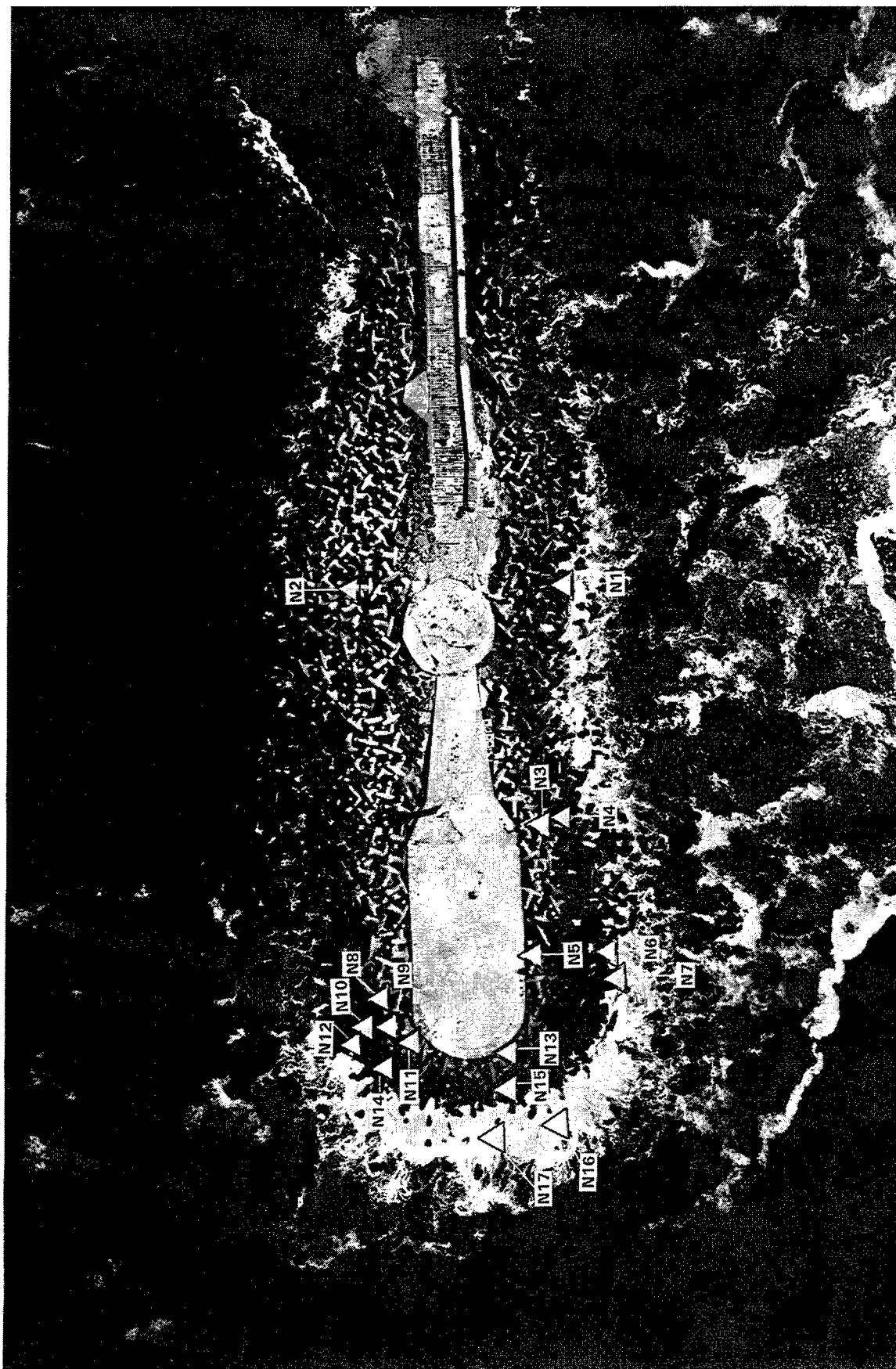
Figure 21. Approximate locations of broken/cracked dolos armor units on the north jetty
