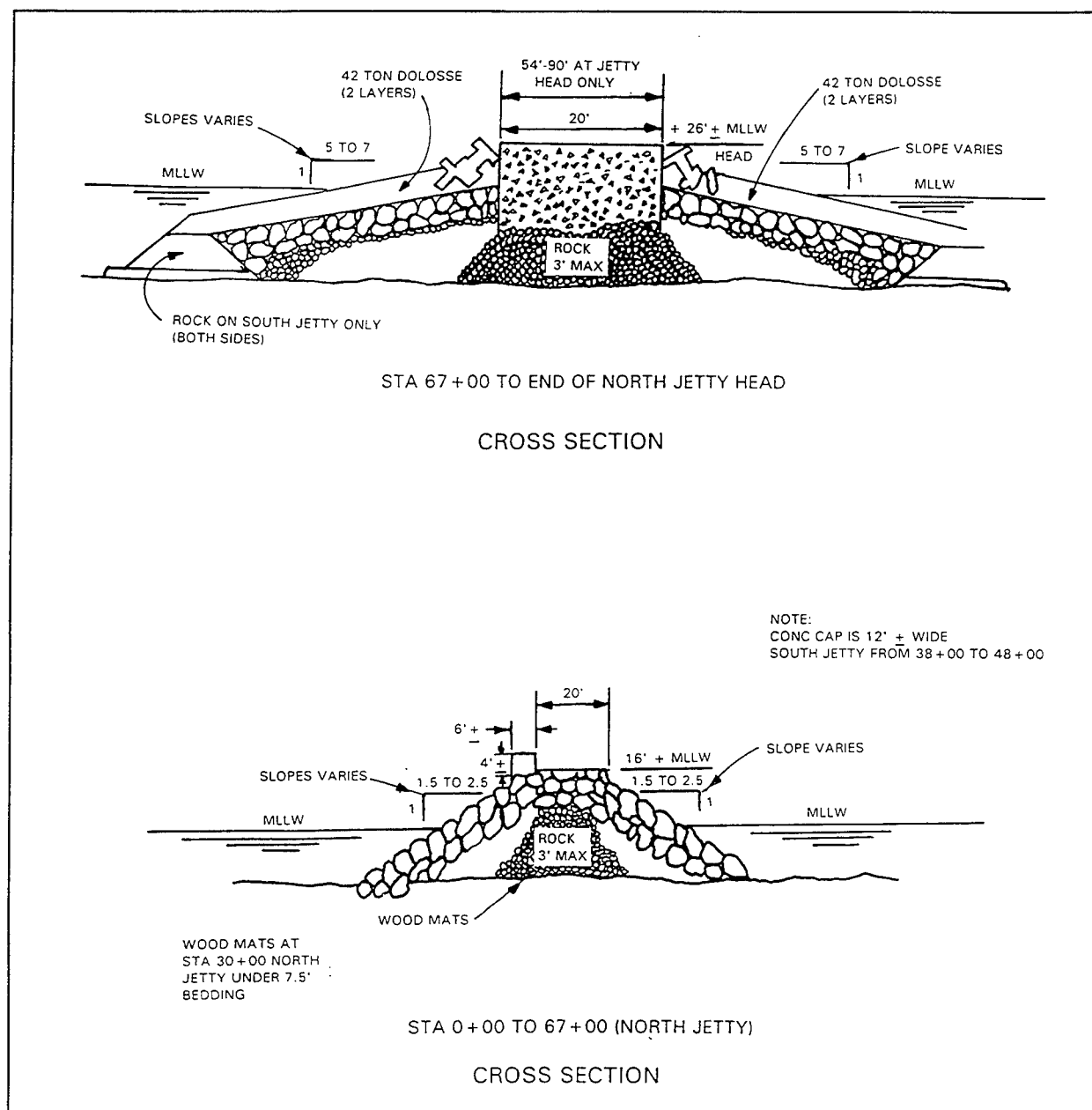
Figure 3. Typical cross section of north jetty
