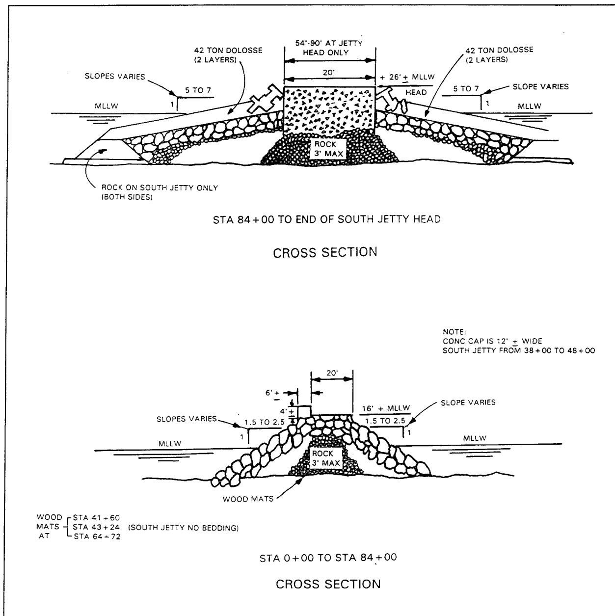
Figure 4. Typical cross section of south jetty
