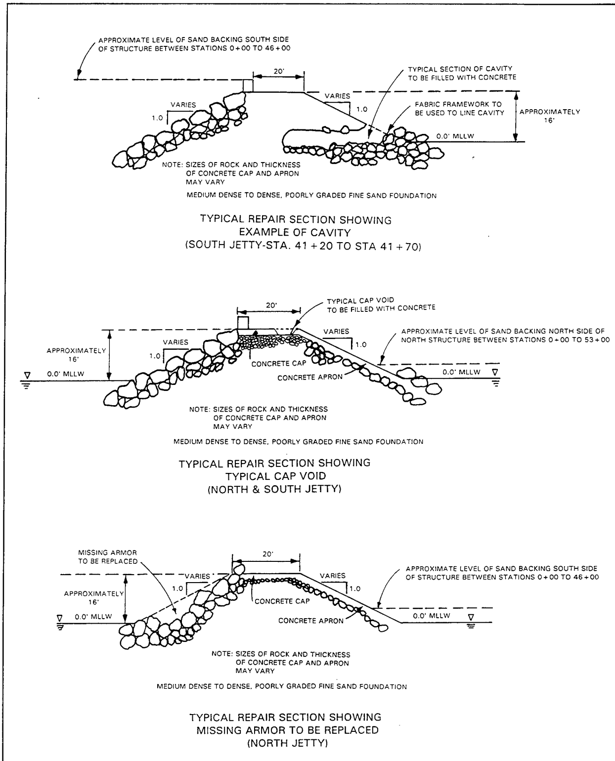
Figure 5. Typical repairs made to jetties in 1988
