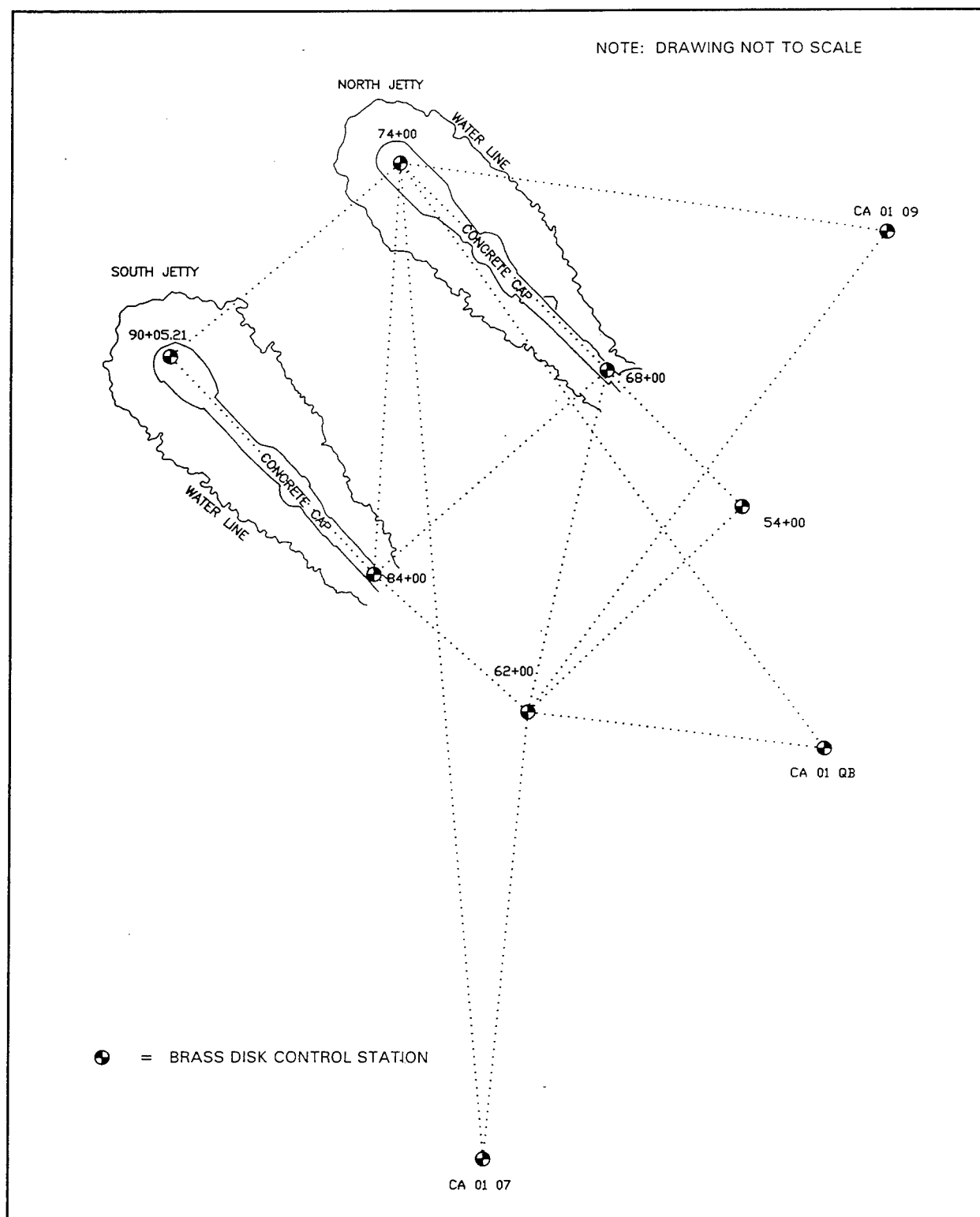
Figure 8. Diagram of monuments used for survey control at Humboldt Bay
