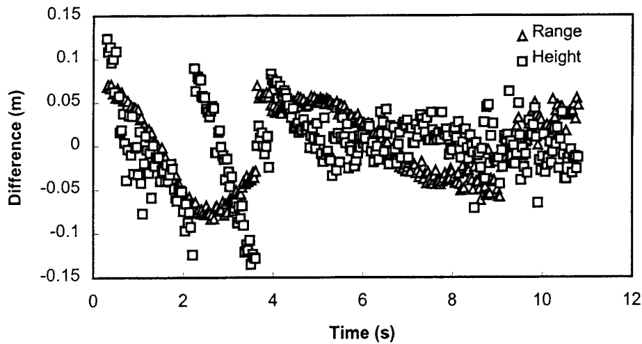
Figure 6. Difference in range and height as a function of time between the input and output of the parameter estimation model.
